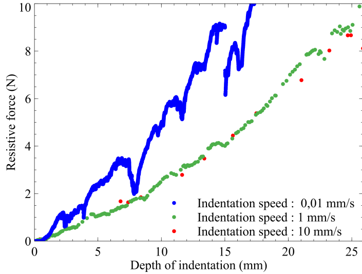
Figure 2.4 – Measured resistive force against depth of indentation for different indentation speeds.
