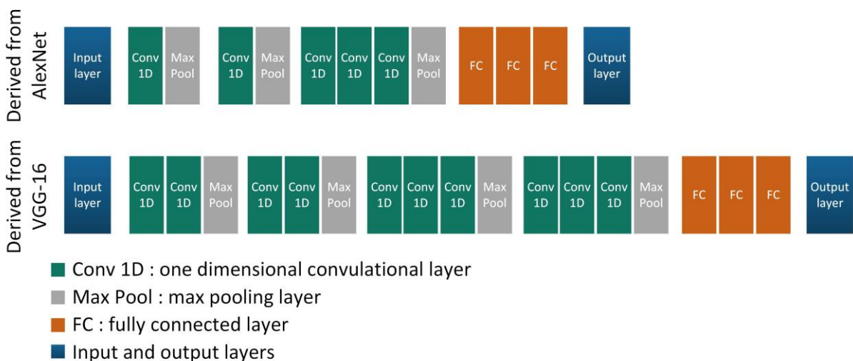
Figure 1.9: 1D-CNN architectures tested
