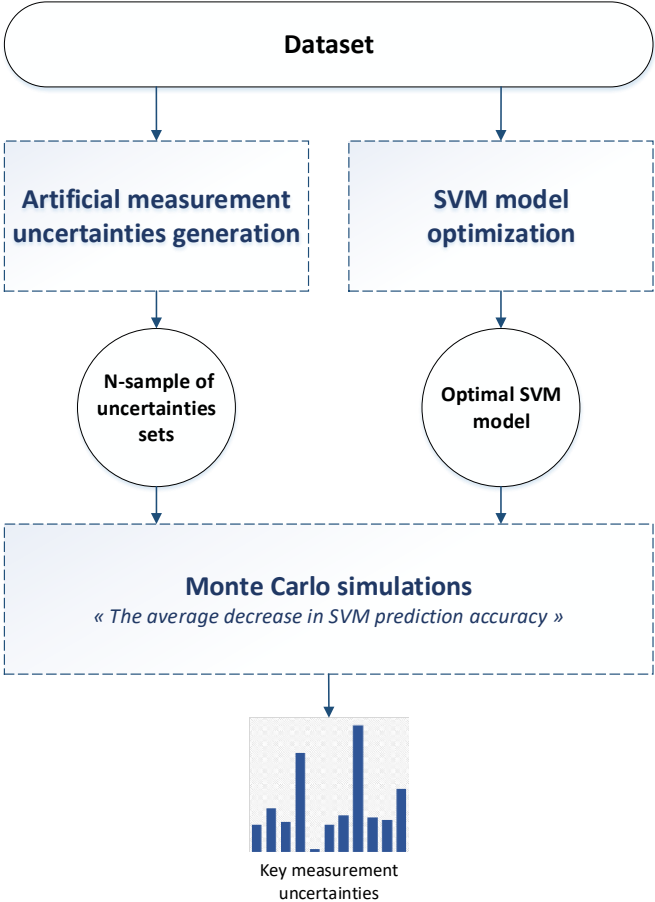
Figure 2.6: Identification of key measurement uncertainties by Monte Carlo simulations
