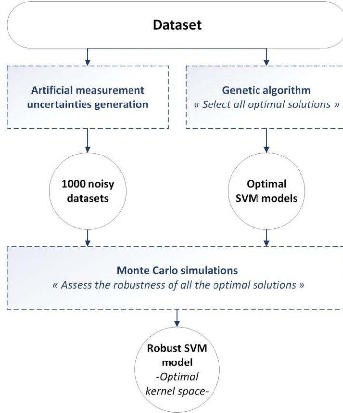
Figure 3.6: Bi-level optimization approach for the selection of robust SVM models
