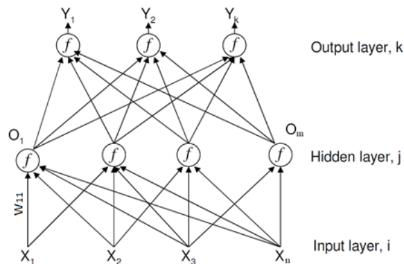
Figure 1.3: A multilayer perceptron with one hidden layer
