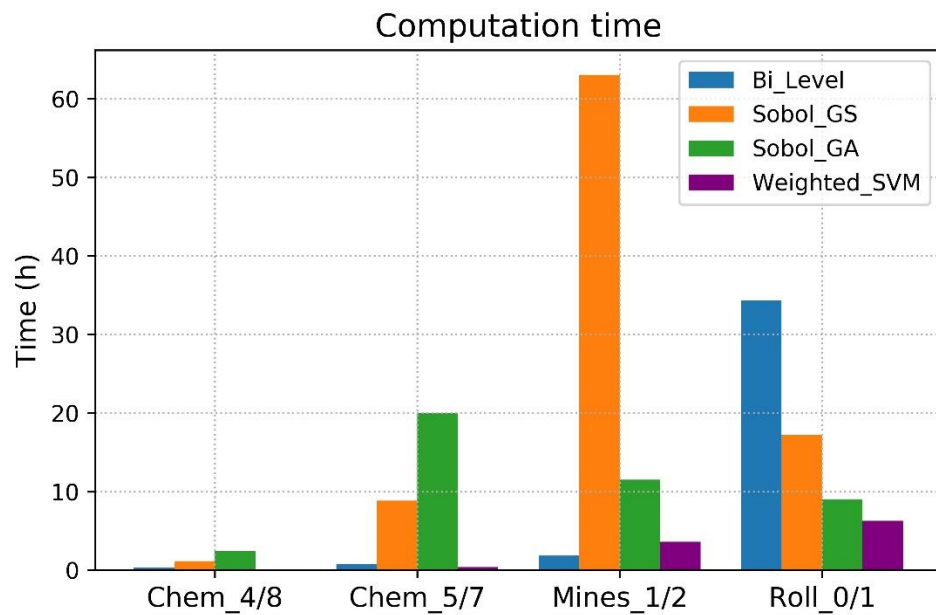
Figure 3.13 (b): Computation times (Bi-Objective results excluded)
