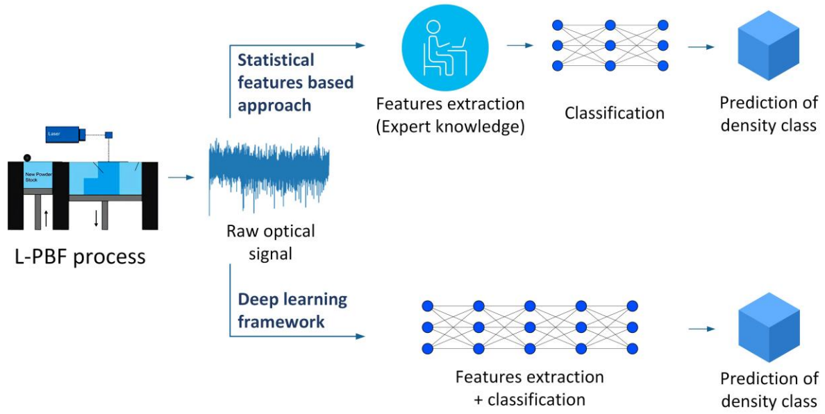
Figure 1.7: Optical quality monitoring approaches for L-PBF process
