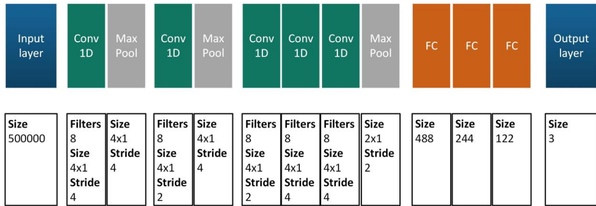
Figure 1.10: Optimal 1D-CNN model
