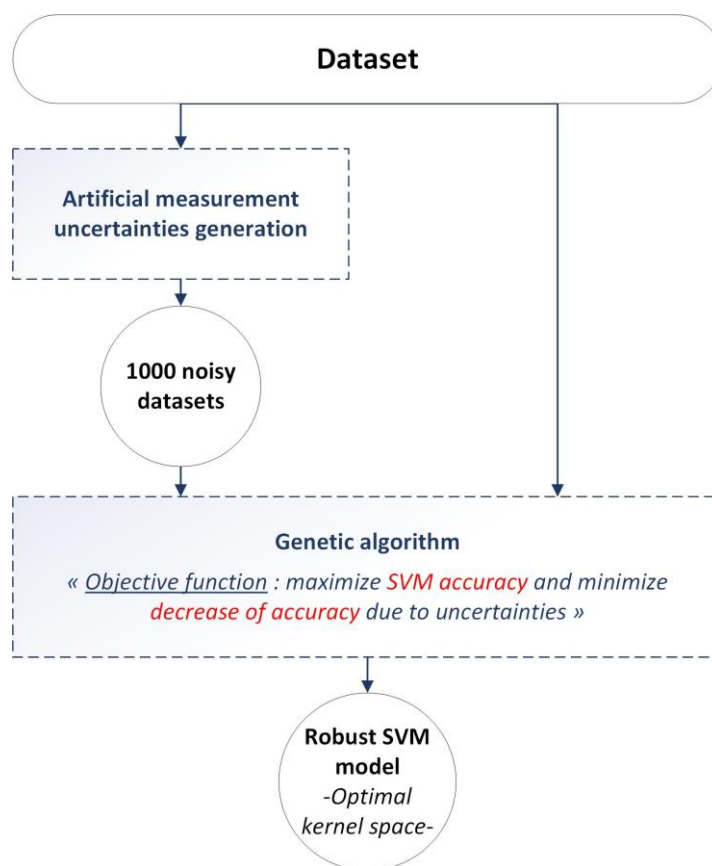
Figure 3.4: Bi-objective optimization approach for the selection of robust SVM models
