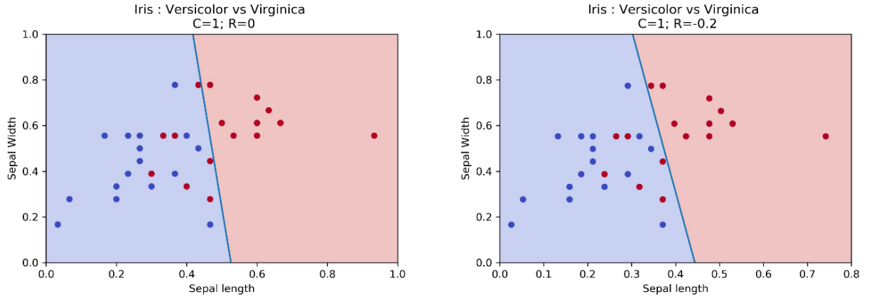
Figure 3.7: Impact of the parameter R on the linear SVM decision boundary
