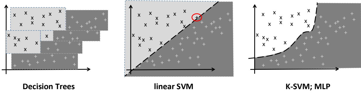
Figure 1.12: Illustration of the classification performed by the studied classifiers
