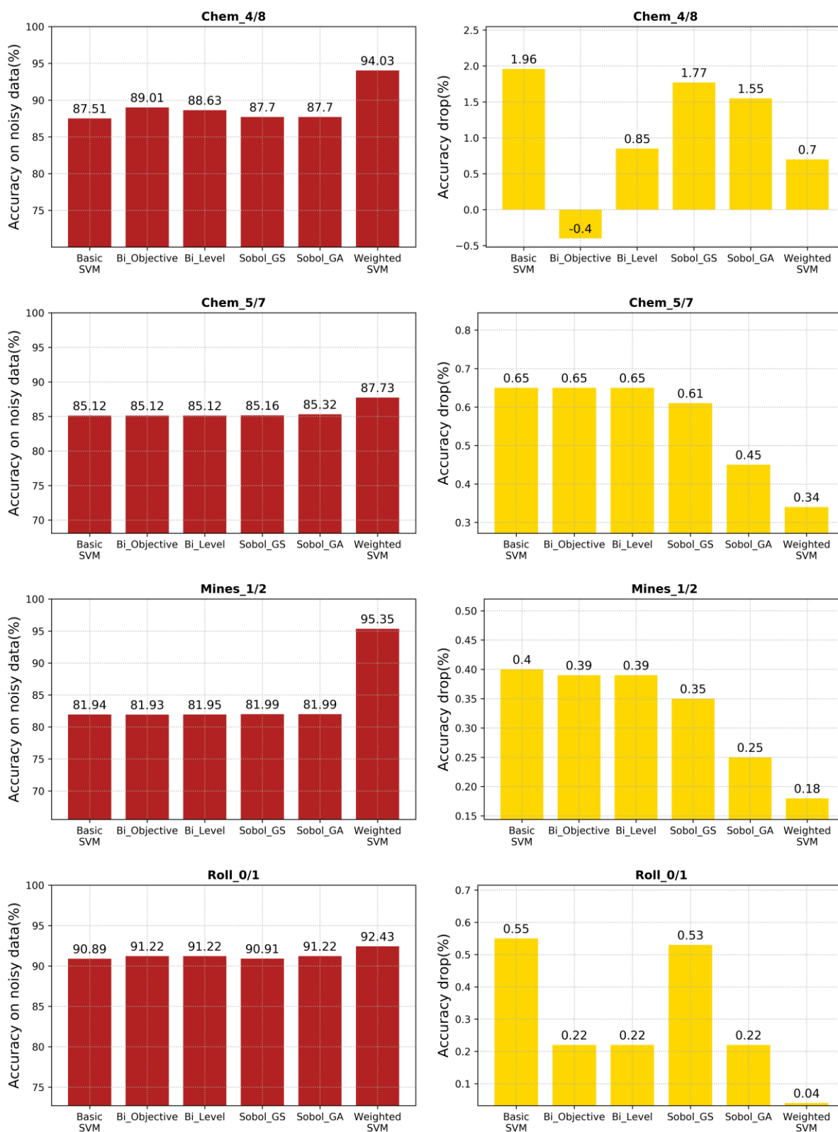
Figure 3.12: Prediction robustness of the proposed approaches
