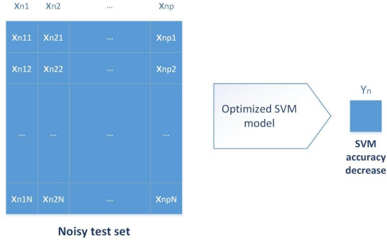
Figure 2.10: Sobol method for analyzing the sensitivity of SVM accuracy
