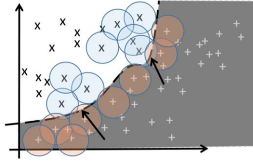
Figure 2.3: Non-linear SVM decision boundary
