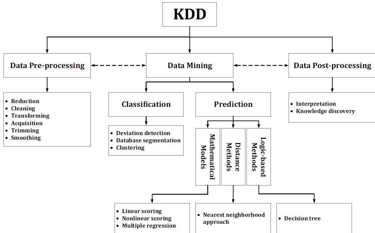
Figure 0.1: KDD main process and sub activities
