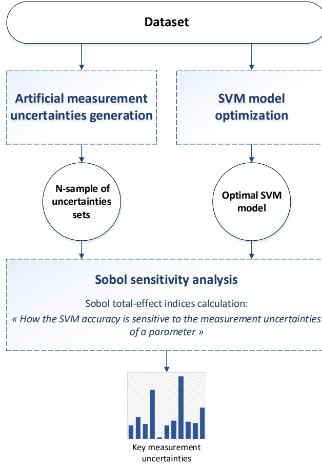
Figure 2.9: Identification of key measurement uncertainties by Sobol sensitivity analysis
