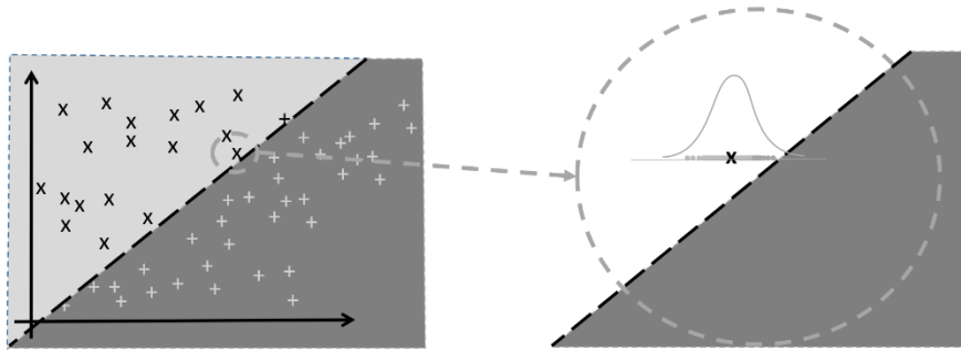
Figure 2.4: Impact of the uncertainties of the first parameter
