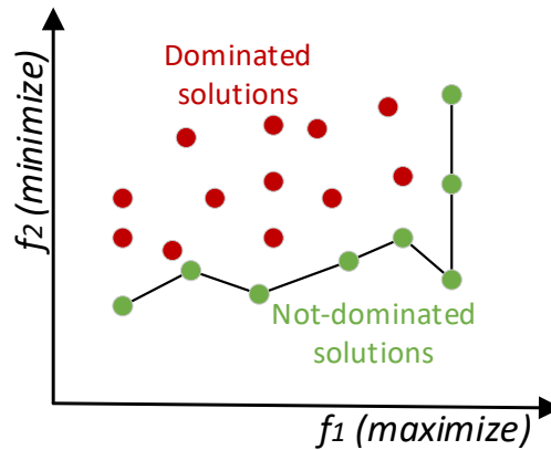
Figure 3.3: Illustration of Pareto optimal solutions
