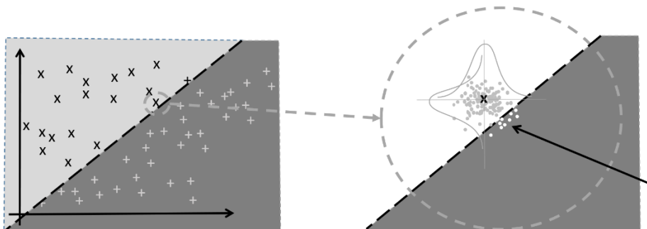
Figure 2.2: Illustration of a datapoint subject to measurement uncertainties
