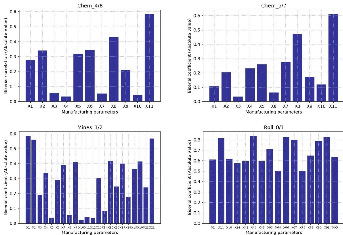
Figure 2.13: Point-biserial correlation coefficients of the manufacturing datasets
