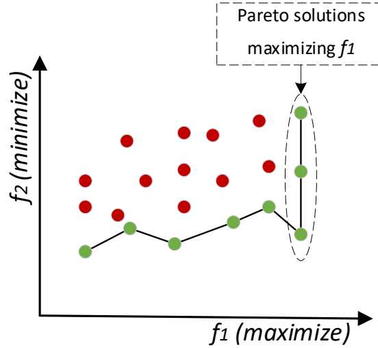
Figure 3.5: Illustration of bi-level optimization solutions
