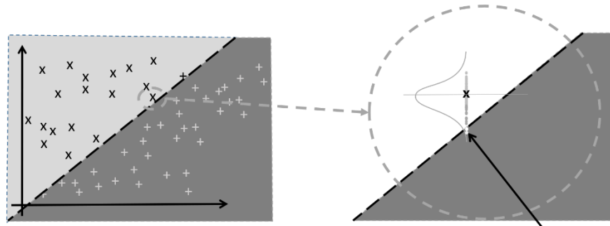
Figure 2.5: Impact of the uncertainties of the second parameter
