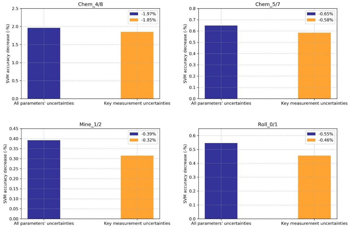
Figure 2.14: Decrease of SVM accuracies due to the key measurement uncertainties
