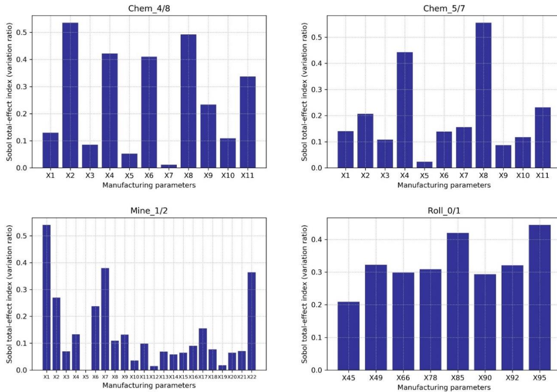
Figure 2.11: Sobol total effect indices of the manufacturing datasets
