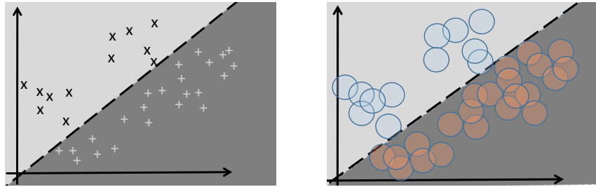
Figure 3.1: Probability of uncertain datapoints to be well classified
