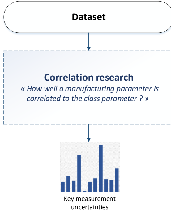
Figure 2.12: Estimation of the key measurement uncertainties by correlation research
