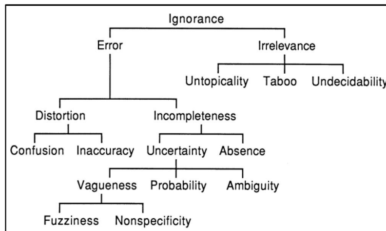
Figure 1.11: Taxonomy of ignorance (Smithson 1989)
