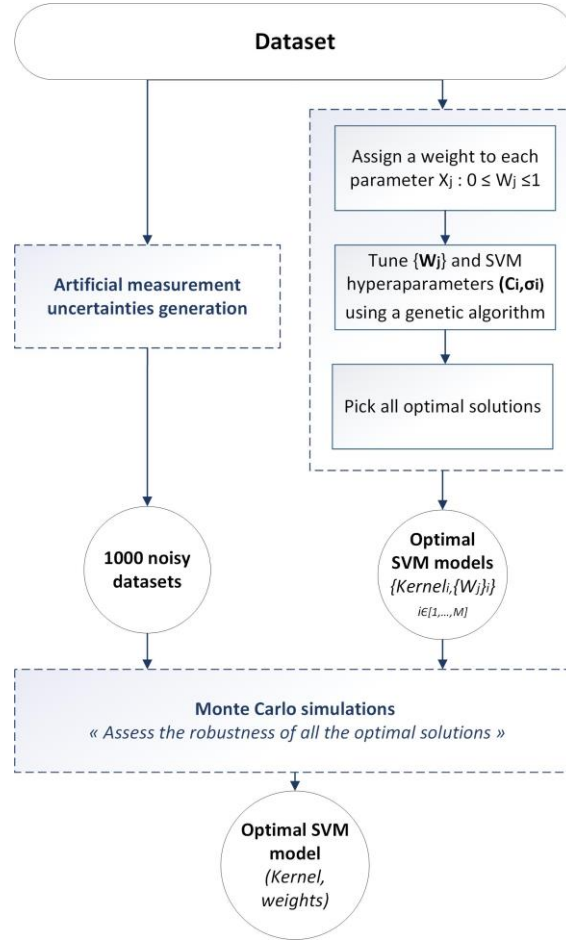
3.10: Robust optimization of feature weights and SVM hyperparameters
