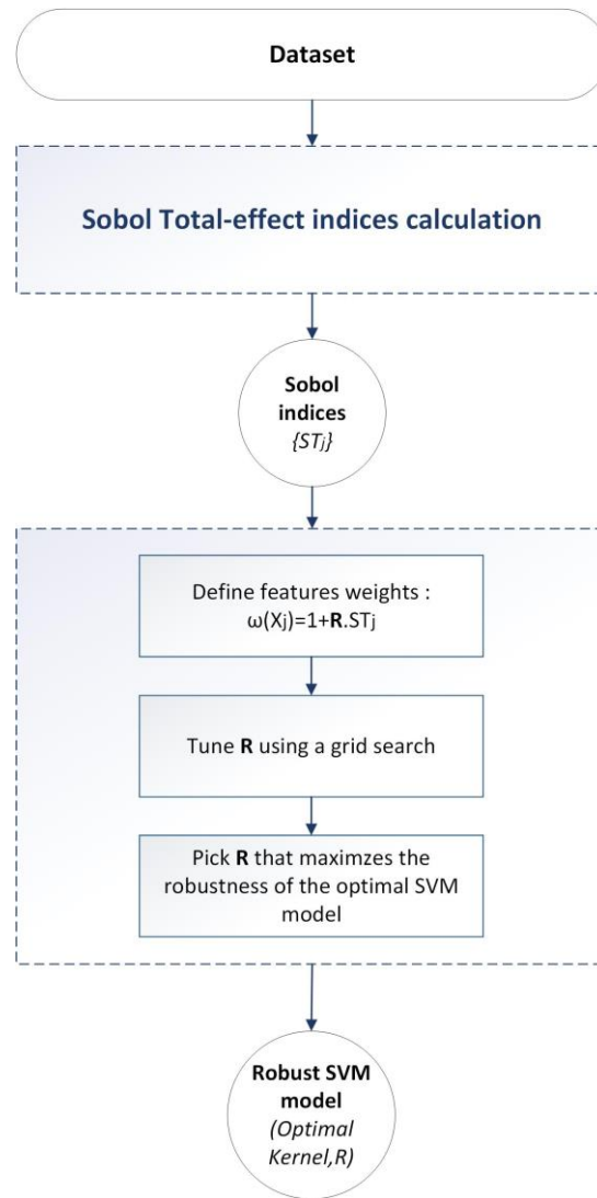
Figure 3.8: A grid search algorithm for tuning the parameter R
