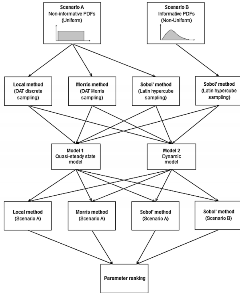
Figure 2.8: Methodical approach for the selection of a SA method (Kristensen et al. 2016)
