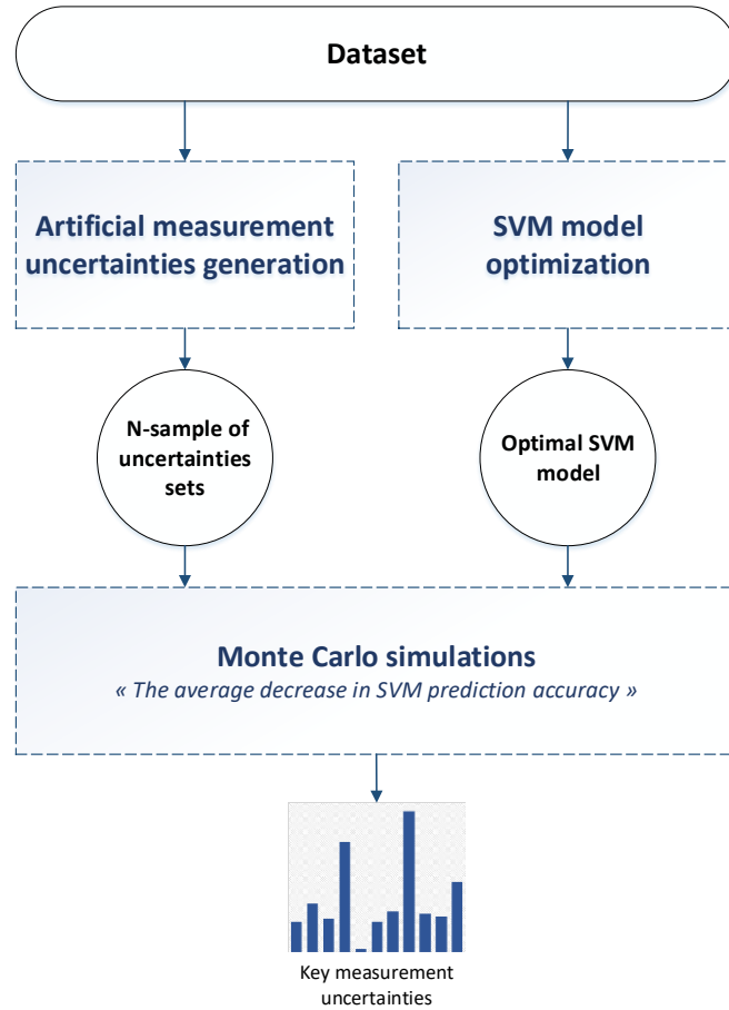
Figure 2.6: Identification of key measurement uncertainties by Monte Carlo simulations
