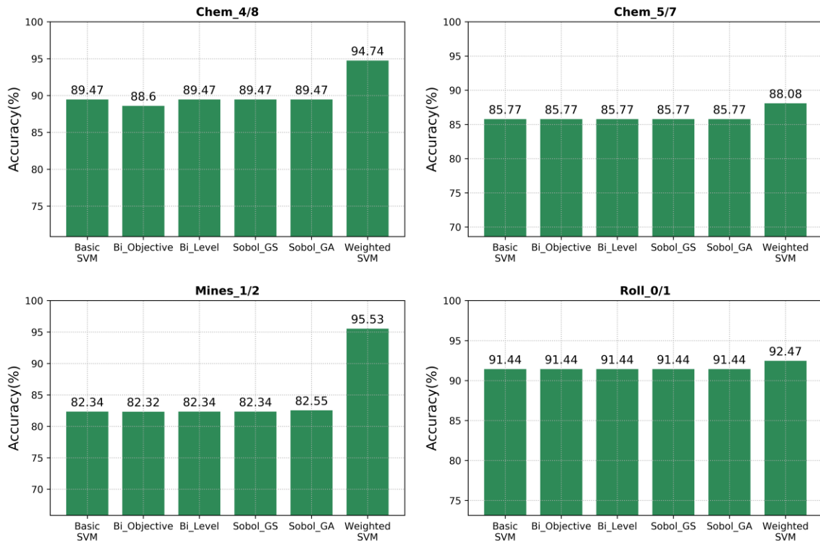
Figure 3.11: Prediction accuracies of the proposed approaches for the four datasets
