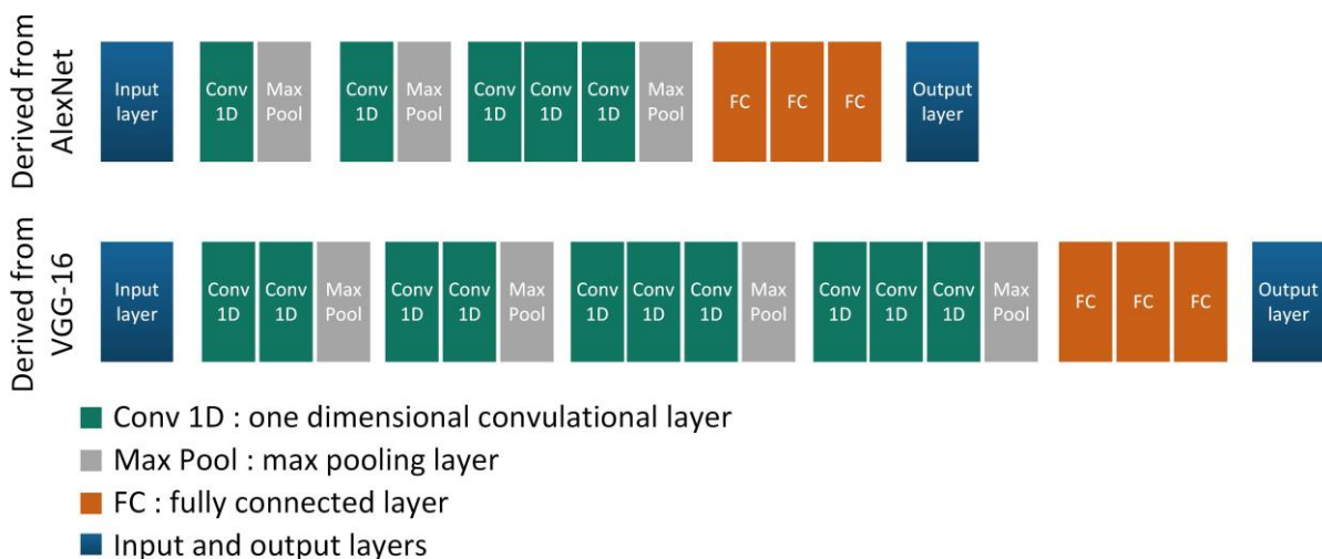
Figure 1.9: 1D-CNN architectures tested
