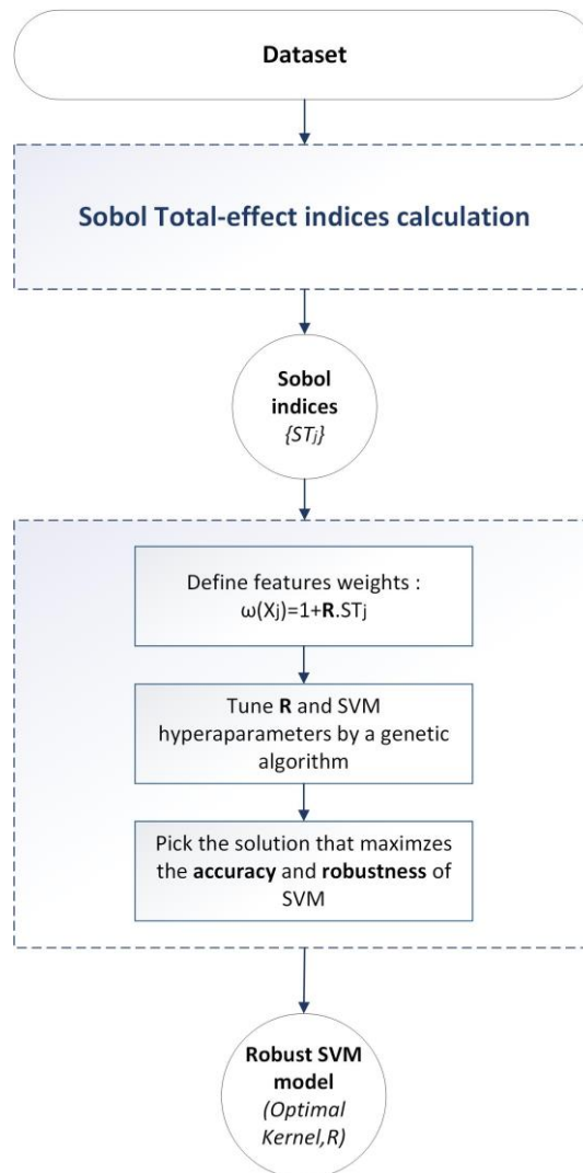
Figure 3.9: Optimization of the parameter R and the SVM hyperparameters
