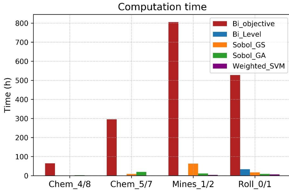
Figure 3.13 (a): Computation times of the proposed approaches
