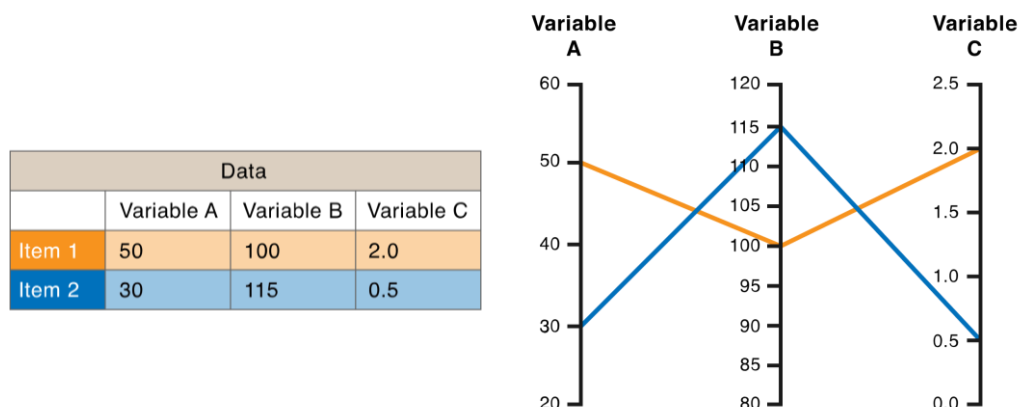
Figure 1.5: Illustration of a data visualization by parallel coordinates
