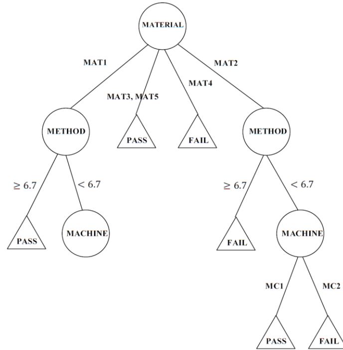
Figure 1.2: C4.5 decision tree for HGA failure identification (Taetragool et al., 2009)
