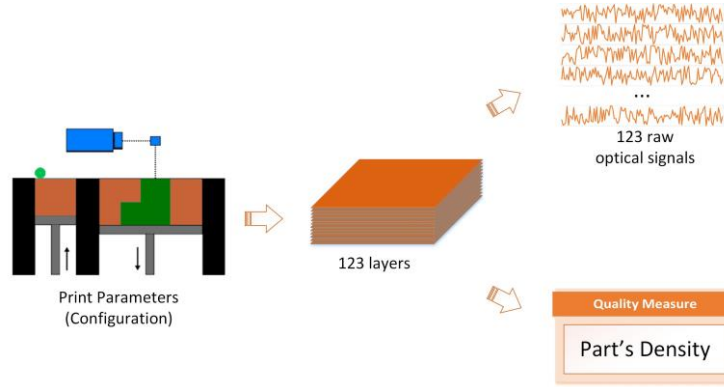
Figure 1.8: Illustration of the L-PBF optical monitoring approach
