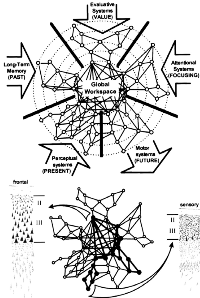
Fig 6. (From Dehaene & Changeux 1998), a cytoarchitectural model (inspired from Mesulam 1998) of the Global Cognitive Workspace. This is one of the best models of the neural correlates of noems (objects of intentional thought) and their fluid multisensory, representational network. The interaction between long term and working memory is very interesting for the neuroergonomics of hyperwriting (ex ante). The model also gives a sound basis to represent the general neuroergonomics of noems, some of the transformations they can undergo and the metrics of their span. All in all, this model is one of the most useful to represent the span of a "mindful" (ie. "a handful of the human mind") or what the human mind can grasp mentally. It is very precious in neuroergonomics.
