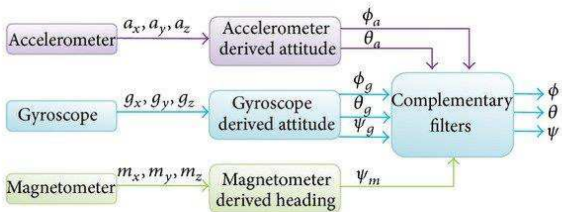
Figure 13: Working principle of complementary filters. Estimation of MIMU local frame orientation (roll \phi , pitch \theta , yaw \psi ) in a global Earth-fixed reference frame from triaxial accelerometer ( a_x, a_y, a_z ), gyroscope ( g_x, g_y, g_z ) and magnetometer ( m_x, m_y, m_z ) readings. Taken from (Amin et al. , 2014)
