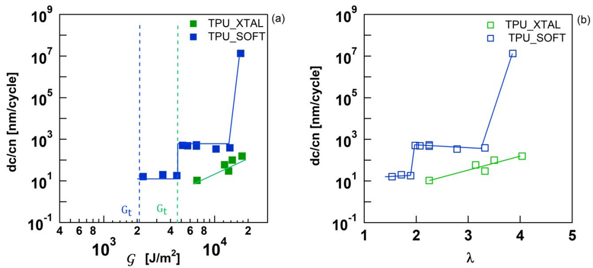
Figure 9-5 Crack growth rate per cycle as function of applied release rate G (a) and applied stretch \lambda (b) for TPU_XTAL and TPU_SOFT at 60°
