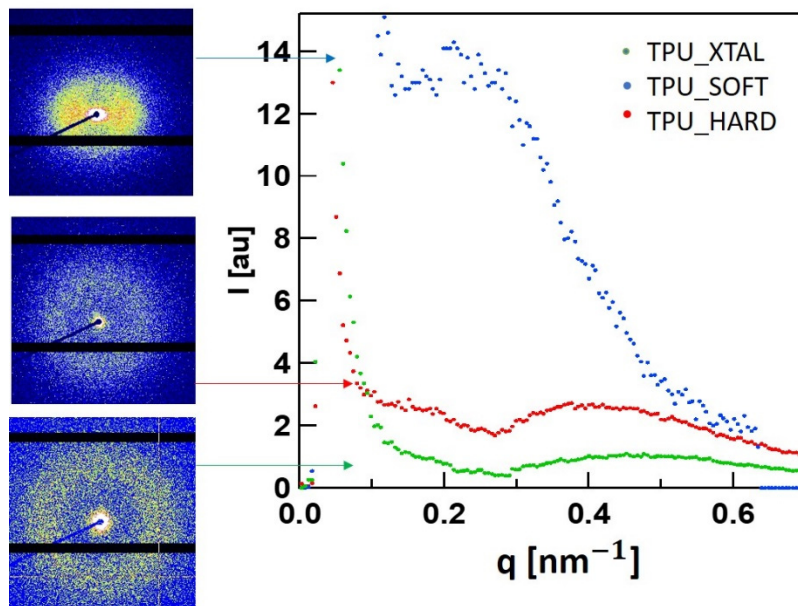
Figure 8-6 2D Pattern and 1D integrating profile for all TPUs.
