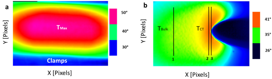
Figure 6-4 Example of temperature map for the un-notched 20CB_8XL strained at \lambda=1.28\% (a) and the notched 20CB_19XL strained at \lambda=1.23 . Data from Mzabi 21
