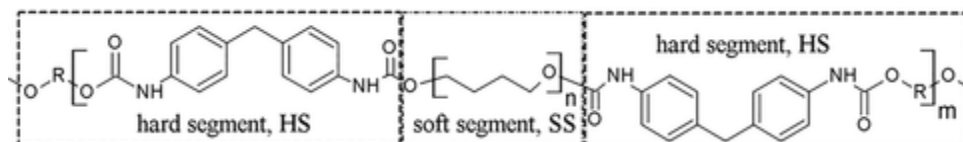
Figure 4-3 Schematic structure of TPU. Image from 6
