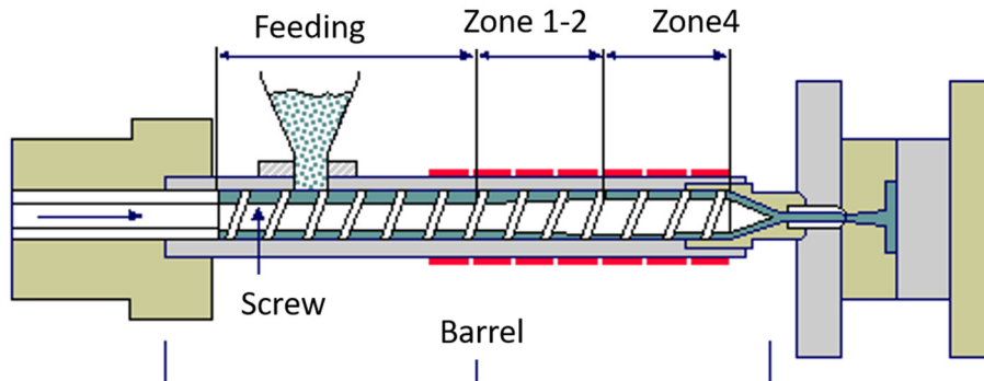
Figure 7-5 Schematic of injection process with the different zones of the barrel
