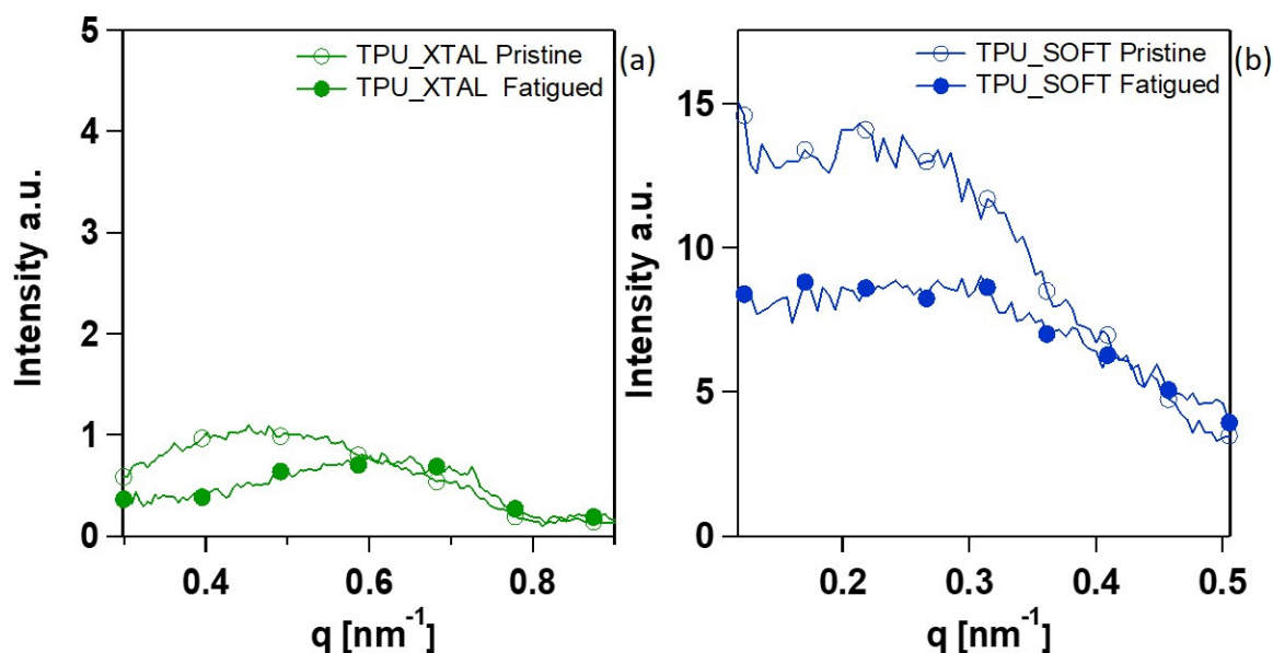
Figure S 9-2 1D integrated SAXS profile for TPU_XTAL (a) and TPU_SOFT (b) both in pristine and fatigued conditions.
