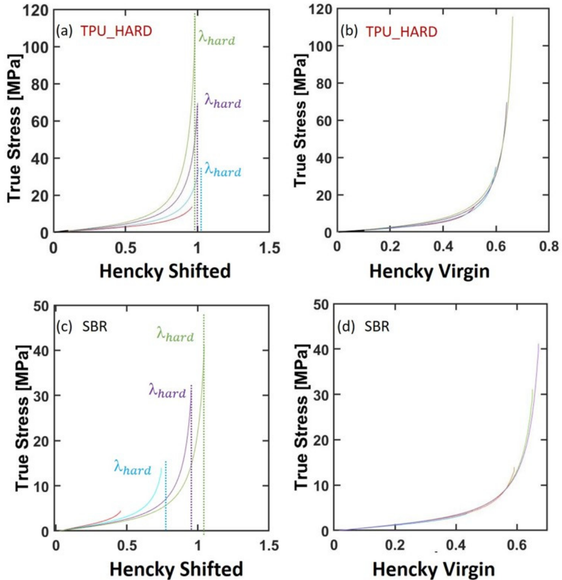
Figure 8-11 Example of True stress VS Hencky Shifted (a-c) and True Stress VS Hencky Virgin (b-d) respectively for TPU_HARD and SBR. The line represent an estimation of the onset of strain hardening and are used for guiding the eyes.
