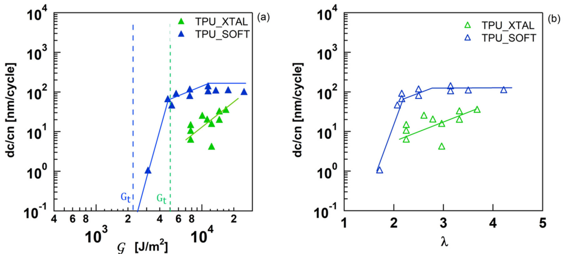
Figure 9-3 Crack growth rate per cycle as function of the applied release rate G (a) and of applied stretch \lambda (b) for TPU_XTAL and TPU_SOFT at 23°C.
