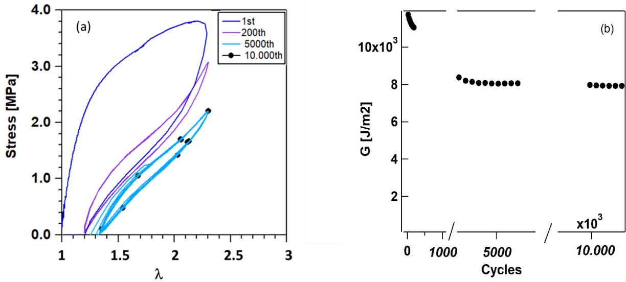
Figure 7-11 Stress-stretch curve of TPU strained at \lambda = 2.3 and evolution of G with cycles.
