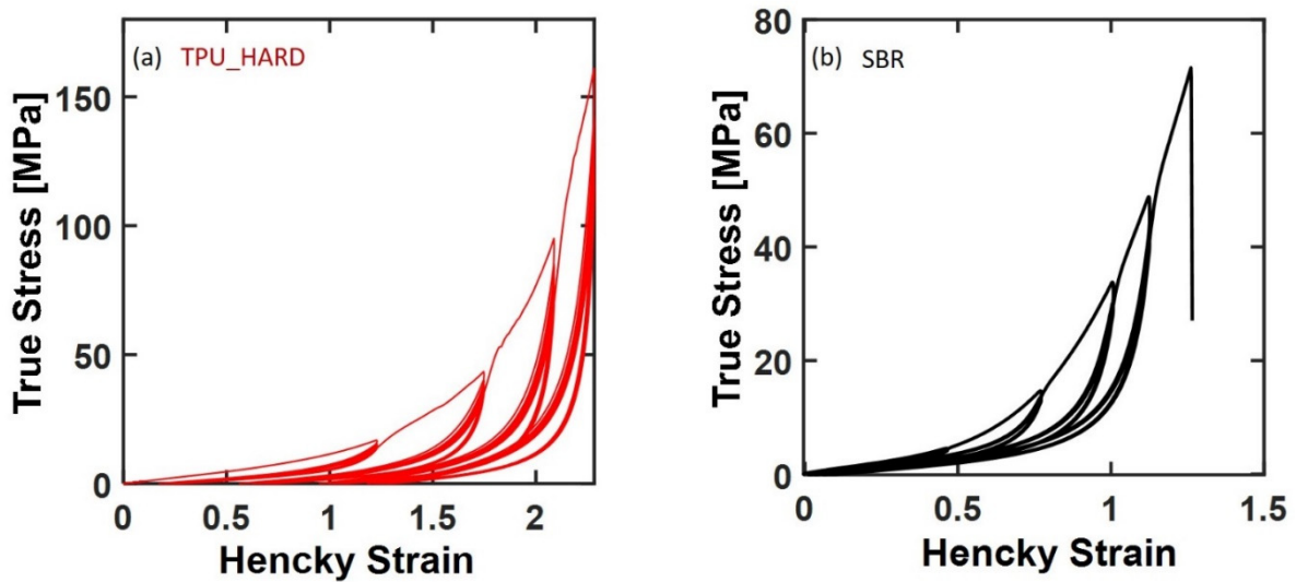
Figure 8-9 True Stress-Hencky strain representation of Cyclic experiment for TPU_XTAL (a) and SBR(b).
