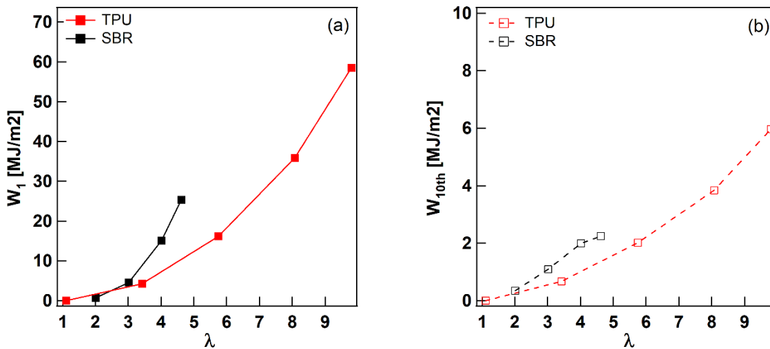
Figure 7-9 Dissipated energy during the first (a) and the 10 th (b) cycle of the uniaxial cyclic experiments
