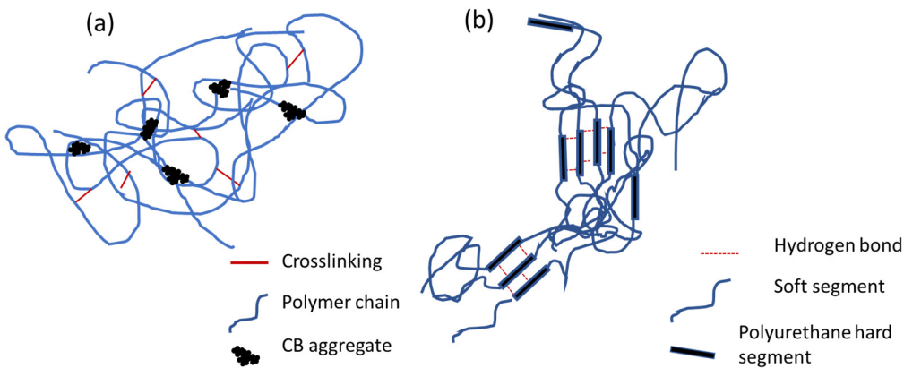
Figure 7-1 Example of network organization for filled crosslinked rubbers (a) and TPUs where the hard domains act as physical crosslinks (b).
