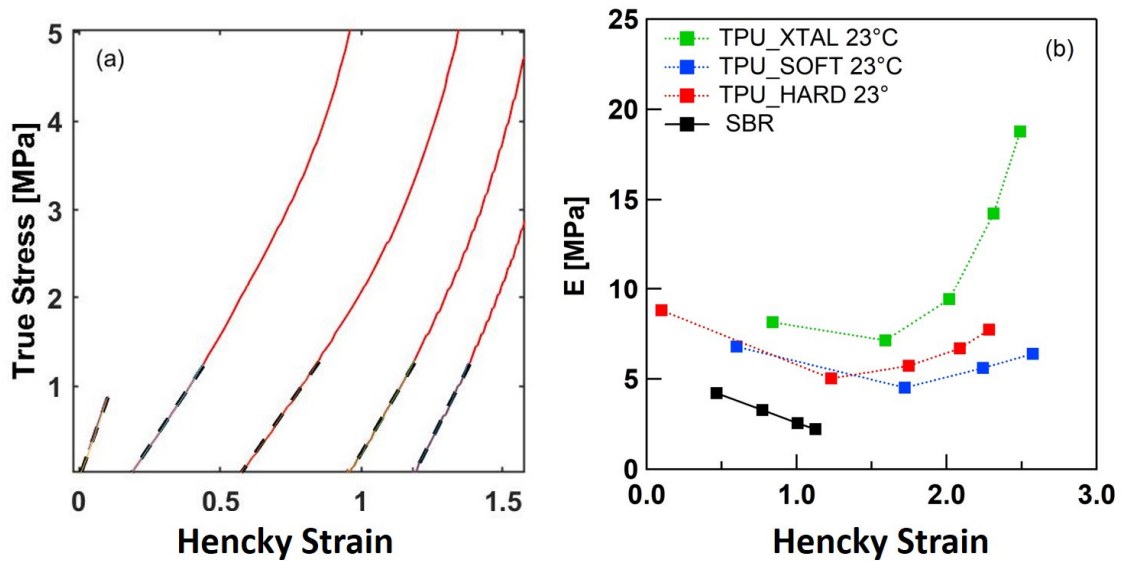
Figure 8-10 Example of linear fitting of calculated E for TPU_HARD(a). E vs Hencky strain for all TPUs and SBR (b)
