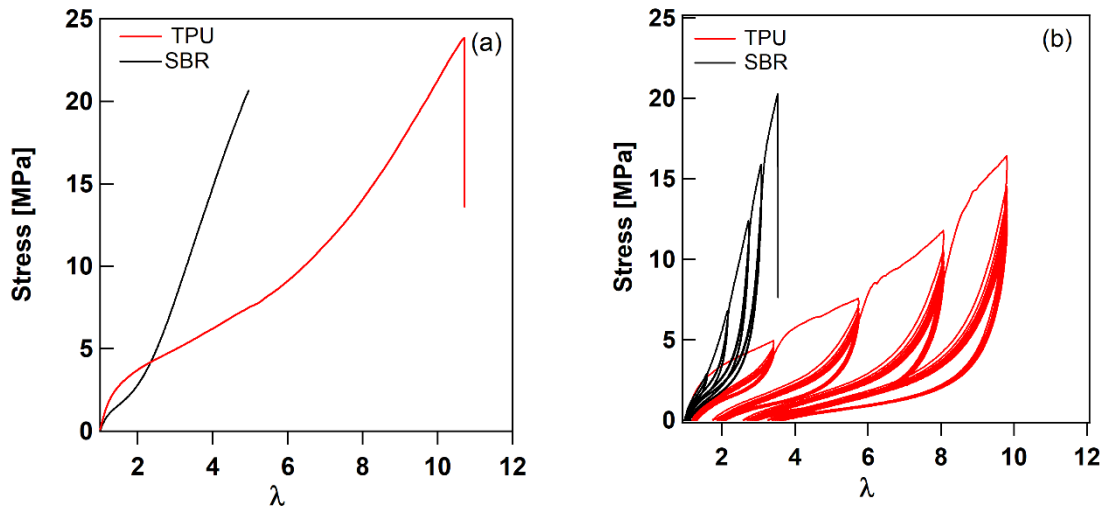
Figure 7-8 Uniaxial nominal tensile test at 23°C for TPU (red) and SBR (black) up to failure (a) and in cyclic experiments (b)
