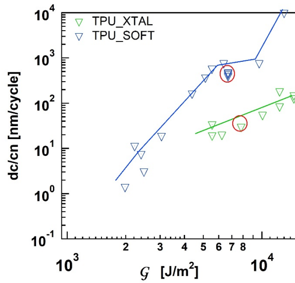
Figure S 9-6 Crack propagation per cycle as function of applied G , method B (allows buckling) for both TPU. The red circles indicate the sample used in X-Ray in situ experiment.
