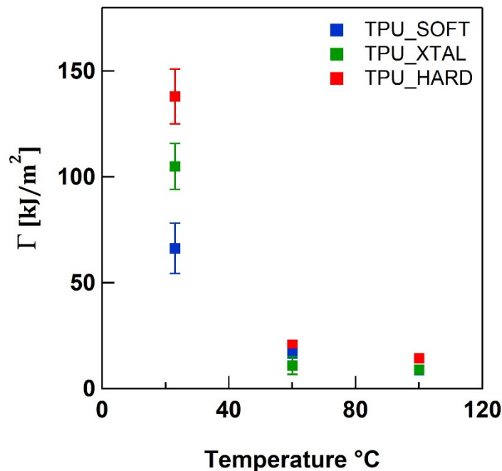
Figure 4 Monotonic toughness for all three TPUs as a function of temperature at 4 \text{ s}^{-1} .
