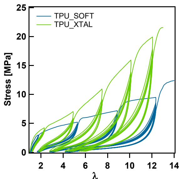
Figure 9-6 Cyclic stress-stretch curve for TPU_XTAL and TPU_SOFT at 23°C and 60°C.
