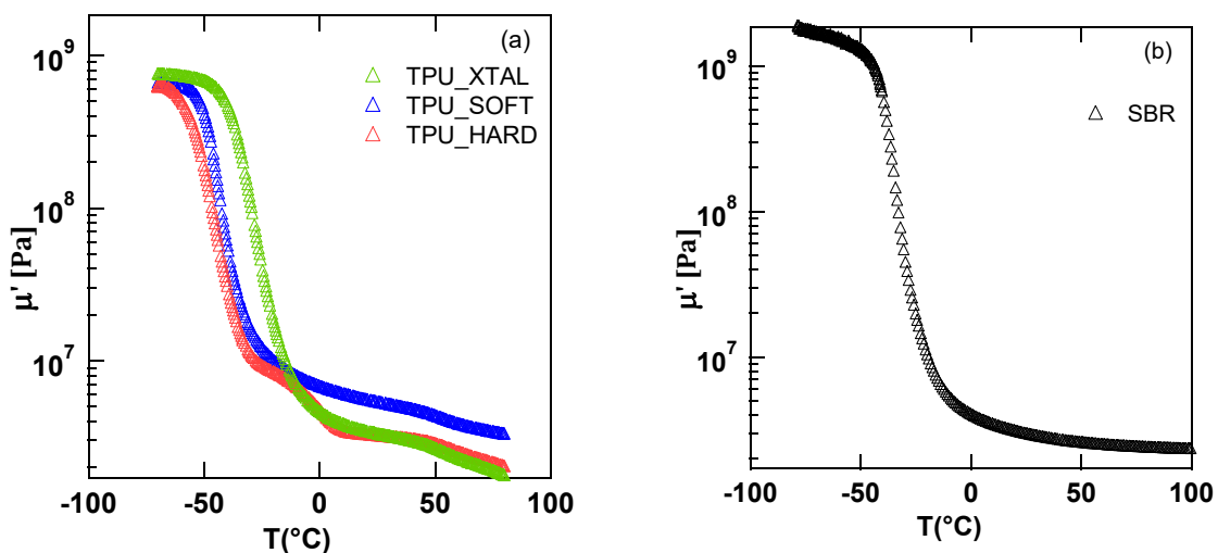
Figure 8-2 Storage modulus VS temperature for three TPUs (A) and for a SBR (B)
