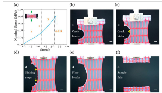
Figure 5-6 Example of composite elastomers. The crack is deflected by the hard network fibres.
