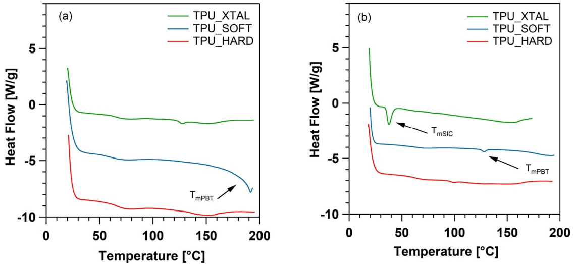
Figure 8-8 DSC thermogram for all TPU pristine (a) and after being strained to rupture (b)
