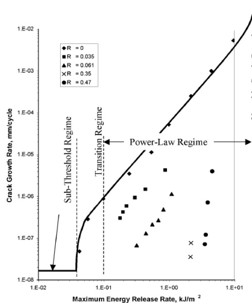
Figure 5-4 Typical regimes of crack propagation dc/dn of natural rubber. Reprinted from Mars 15
