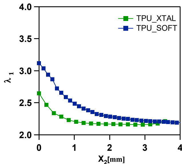
Figure 9-11 Maximum stretch in the vertical direction \lambda_1 as a function of the distance from the open crack tip for samples fatigued at \lambda_{\max} = 2.25
