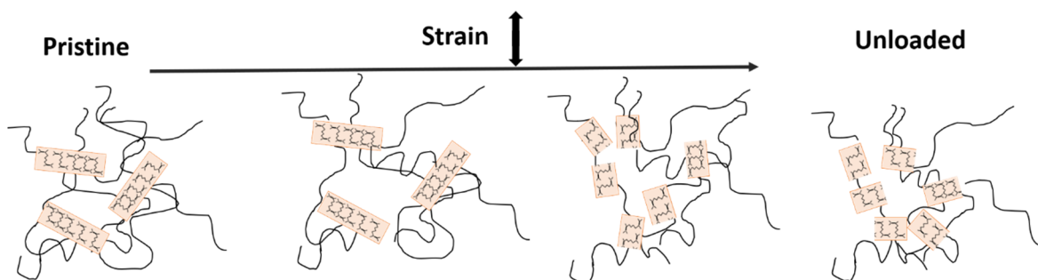
Figure 9-14 Sketch of the effect of elongation on HD restructuring
