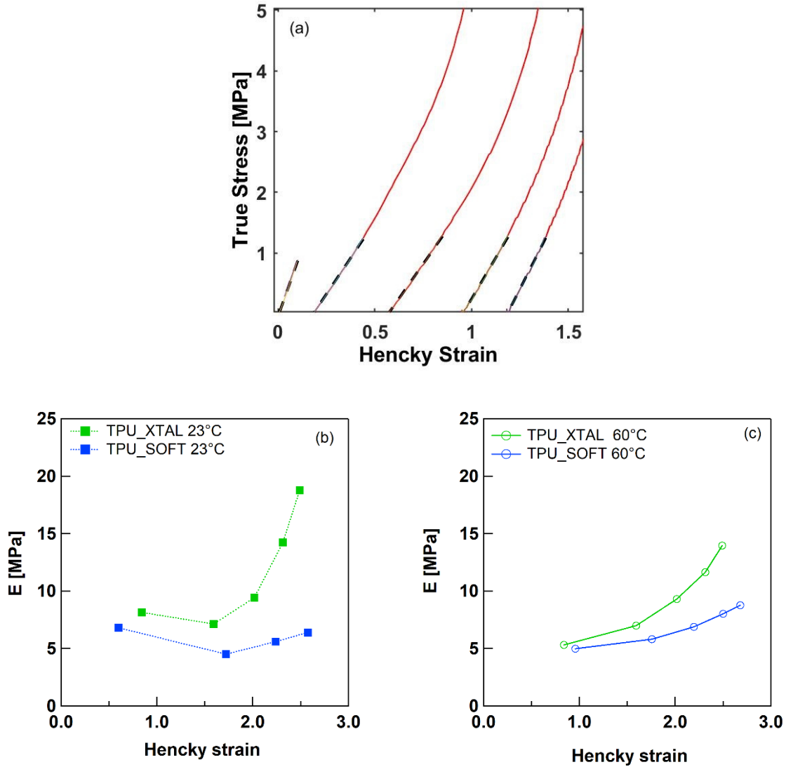
Figure 9-7 Representative true-stress VS Hencky strain unloading curve in cyclic experiment for TPU_XTAL, the inset shows the linear approximation used to calculate E (a). E vs maximum Hencky strain for both TPUs at 23°C (b) and 60°C (c)
