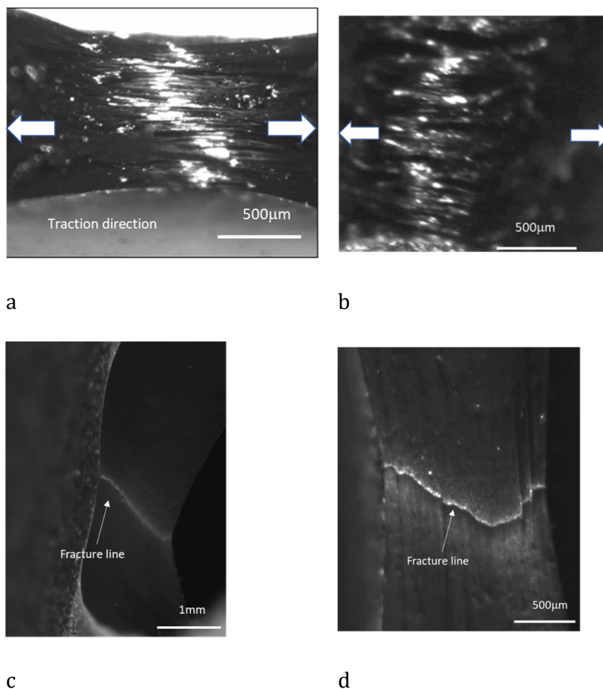
Figure 6-9 Optical images of crack front for the sample 3CB_8XL strained at \lambda = 1.18 in cyclic (a) and at \lambda = 1.67 in static (b) conditions. 20CB_19XL at \lambda = 1.30 (c) and 20CB_8XL at \lambda = 1.80 in static conditions.
