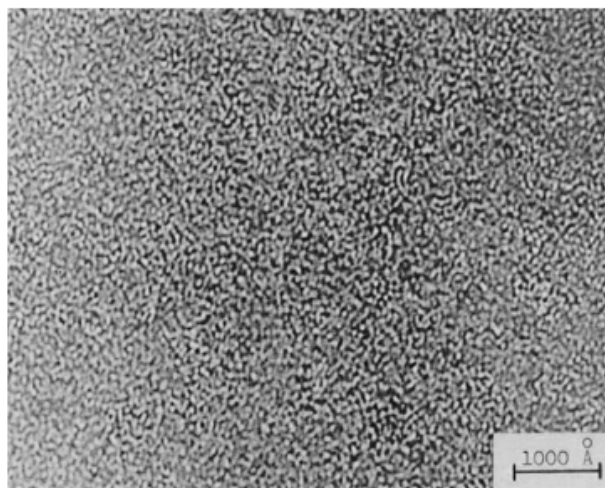
Figure 4-6 TEM image showing the 2-phase structure in polyester-urethane block copolymer. Reprinted from 22
