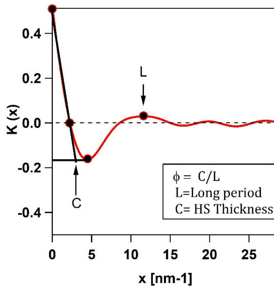
Figure 8-1 Example of correlation function and interpretation of its features for TPU_HARD based on the analysis of Strobl and Schneider 22
