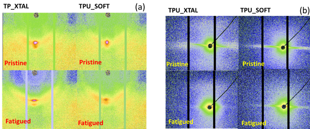
Figure 9-12 WAXD (a) and SAXS (b) representative 2D patterns taken close to the crack tip for pristine and fatigued TPU monotonically strained at \lambda_{\max}=2.25
