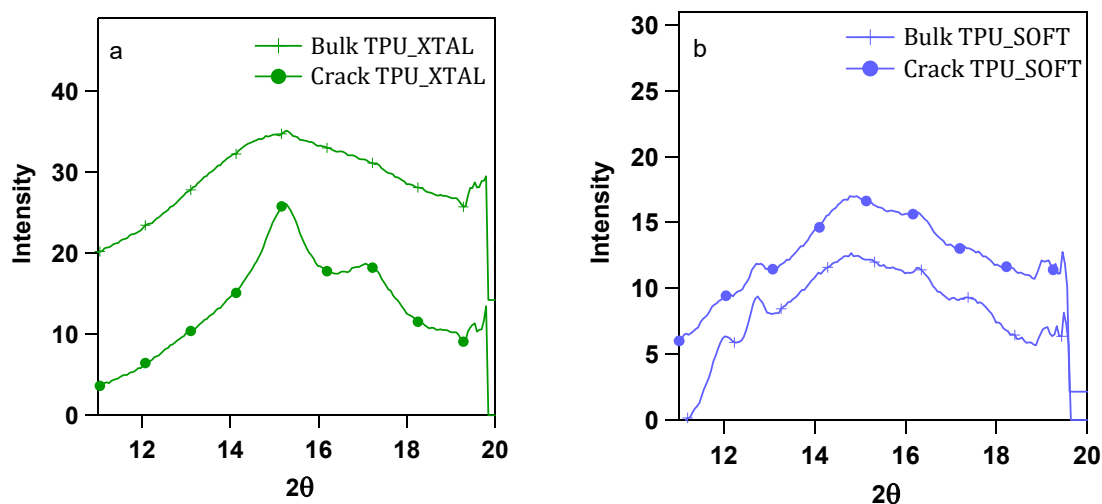
Figure 9-10 Integrated 1D profile of WAXD crystalline peak in TPU_XTAL (a) and TPU_SOFT (b) representative of the crack tip and bulk area.
