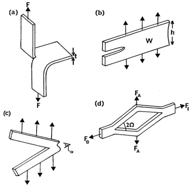
Figure 5-2 : Some geometries used in fracture experiment for rubber (a) “trousers”; (b) pure shear; (c) “angled” ; (d) “split” tear. Reprinted from 5 .
