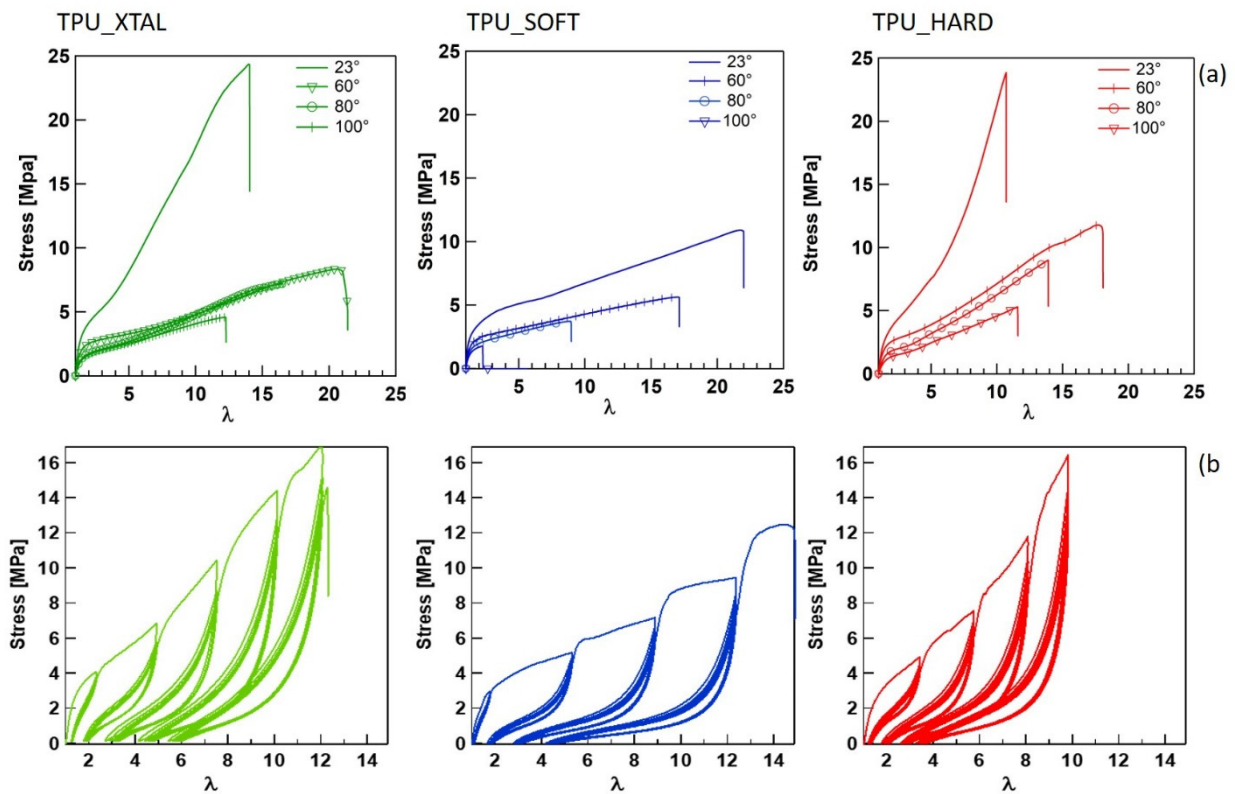
Figure 8-3 Uniaxial stress-strain curves at different temperatures (a) and cyclic stretch-stress curve at 23° (b) for three TPUs.
