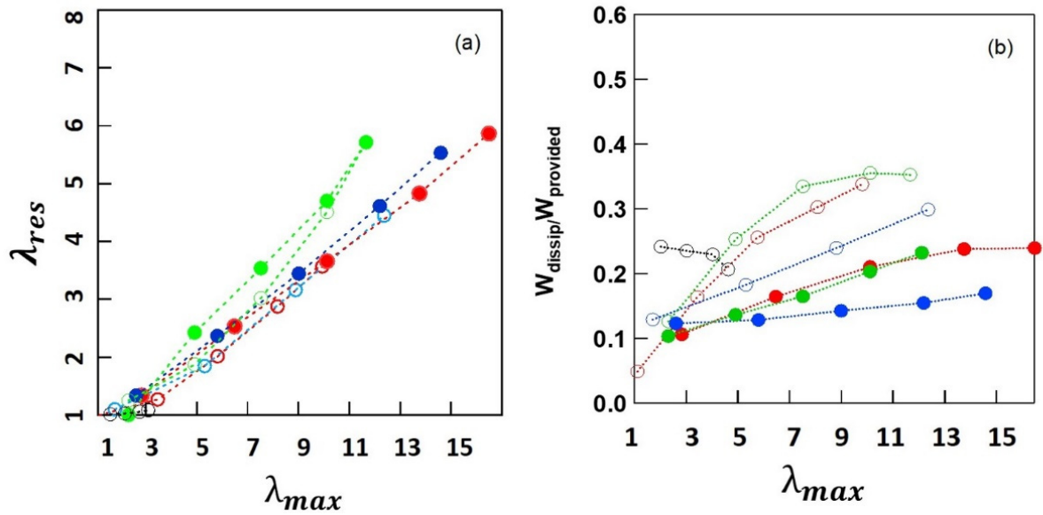
Figure 8-4: (a) Residual VS applied deformation and (b) ratio between dissipated and provided energy during the 10th cycle for all materials. At 23° for: TPU_XTAL \cdots\textcircled{\text{green}}\cdots , TPU_SOFT \cdots\textcircled{\text{blue}}\cdots , TPU_HARD \cdots\textcircled{\text{red}}\cdots , SBR \cdots\textcircled{\text{grey}}\cdots and at 60° for: \cdots\textcircled{\text{green}}\cdots TPU_XTAL \cdots\textcircled{\text{blue}}\cdots TPU_SOFT \cdots\textcircled{\text{red}}\cdots TPU_HARD.
