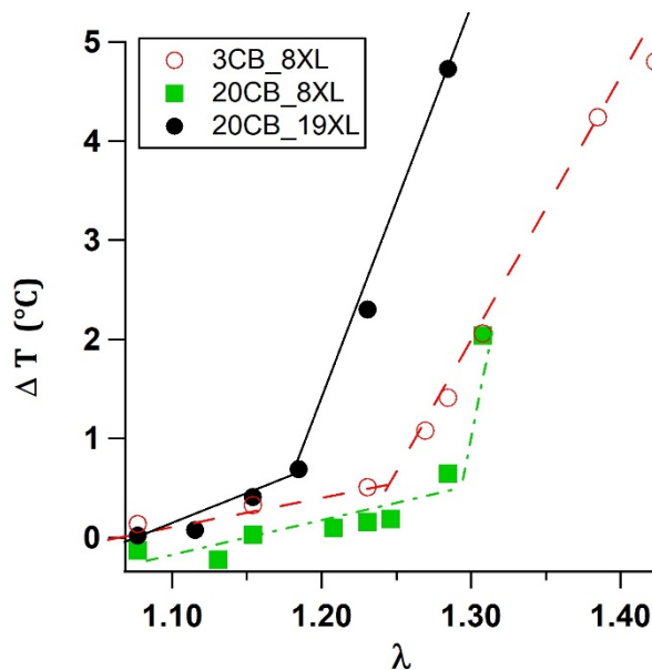
Figure 6-6 Temperature difference between bulk and crack tip ( \Delta T ) as function of applied strain. Data from Mzabi 21
