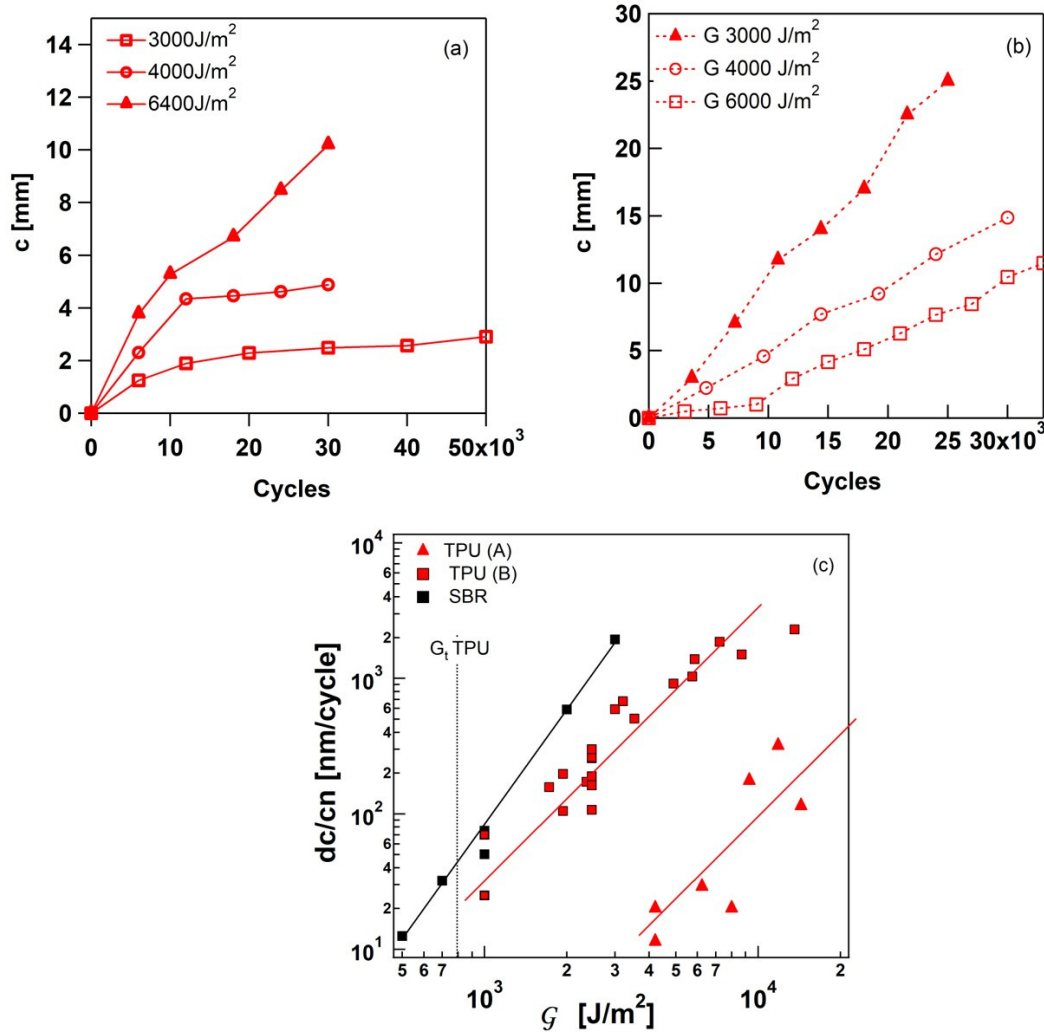
Figure 7-15 Crack length vs cycles for TPU with protocol A (a) and protocol B (b) for different values of the applied G . Crack propagation per cycle for TPU (protocol A and B) and SBR (c).
