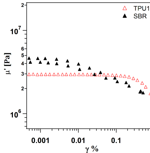
Figure 7-7 Storage modulus vs. dynamic strain amplitude for TPU and SBR at 23°C and 10Hz.
