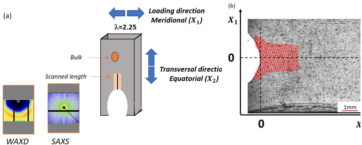
Figure 9-8 Sketch of experimental set-up for WAXD and SAXS experiments (a). Example of open crack profile and deformed mesh obtained from DIC analysis. X_1 indicates the direction parallel direction (meridional) and X_2 the perpendicular direction (equatorial) to the applied load (b).
