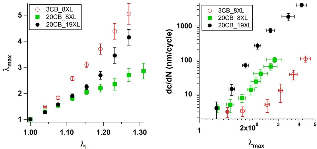
Figure 6-11 Maximum \lambda_{max} at the crack tip as function of applied macroscopic \lambda (a) and dc/dn as function of \lambda_{max} (b) for all SBR.
