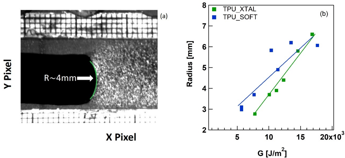
Figure 9-4 Example of crack opening profile in TPU_XTAL at G = 12,000 \text{ J/m}^2 (a) and fitted radius as a function of the energy release rate for both TPUs (b)
