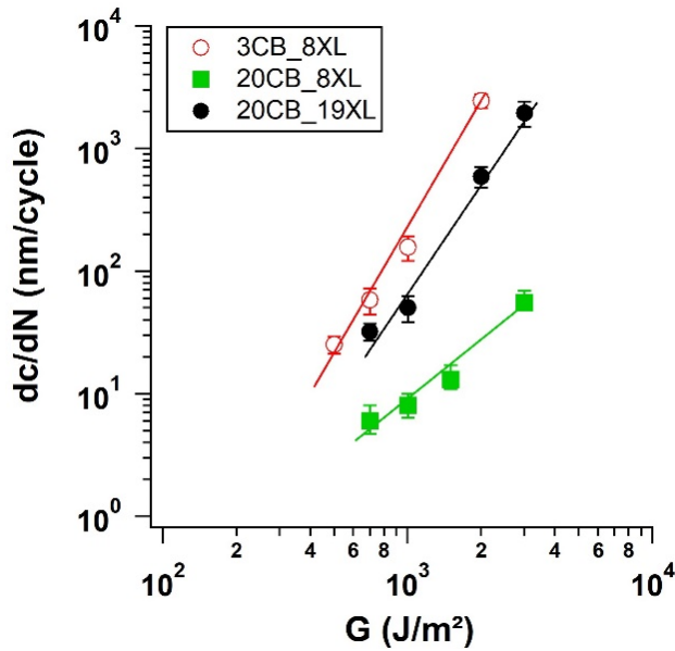
Figure 6-3 Crack propagation rate dc/dN as function of G for all tested materials. Data from Mzabi 21
