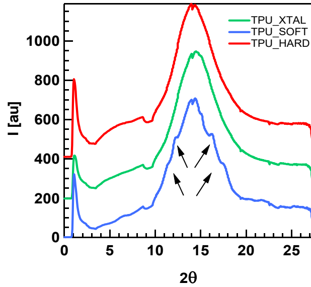
Figure 8-5 WAXS pattern for pristine TPU_XTAL, TPU_SOFT and TPU_HARD
