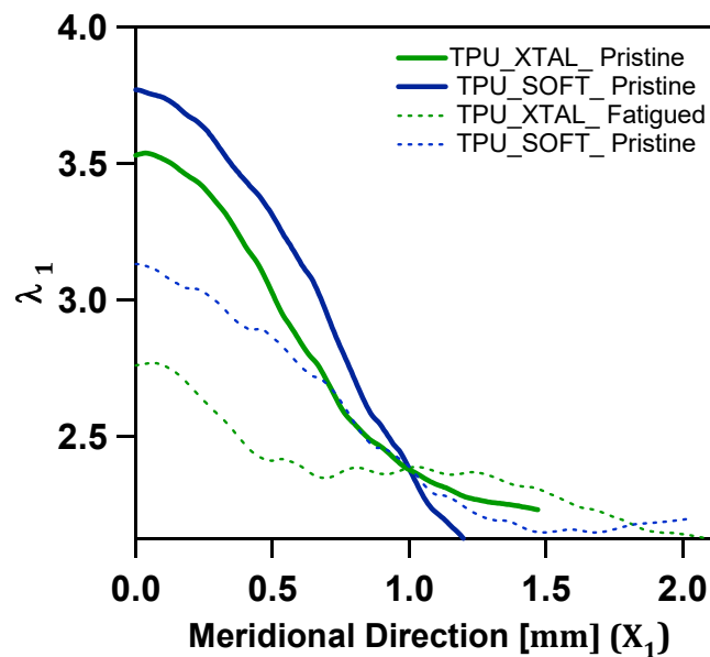
Figure 9-15 Distribution of the maximum \lambda_1 at the crack tip along the loading direction X_1 for pristine and fatigued samples.
