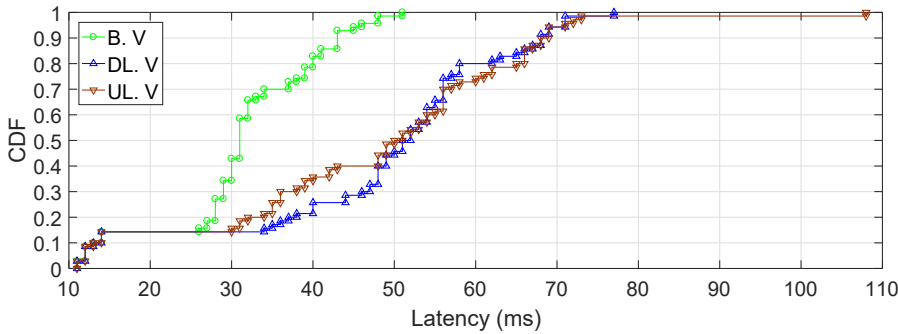
Figure 28 – Hexagonal topology with 7 e2NBs and 70 UEs using 10MHz in FDD mode.
