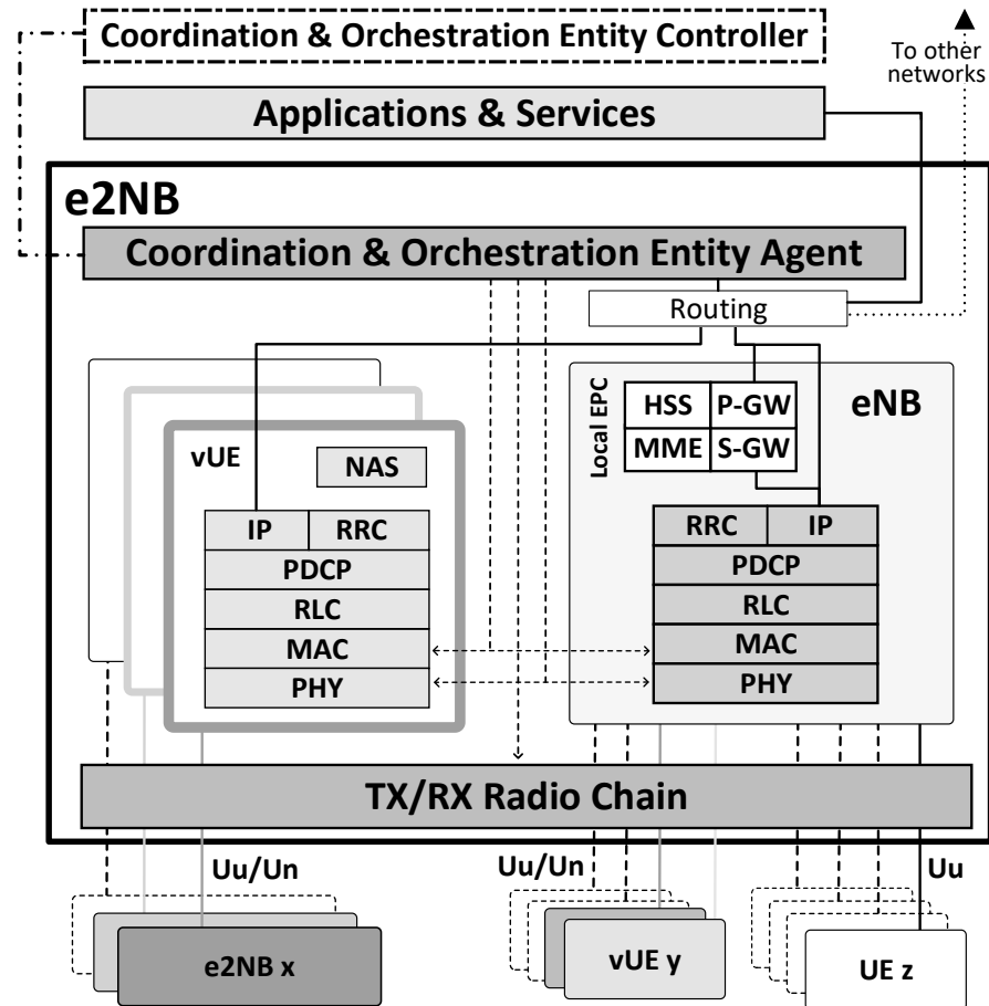
Figure 10 – e2NB stack.
