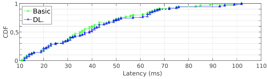
(c) CDF plot of the 95-th percentile of packet latency among real-time flows. 7 → 5 elastic flow scenario without VoIP hop limitation.
