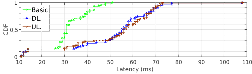
(b) CDF plot of the 95-th percentile of packet latency among real-time flows. 4 \rightarrow 6 elastic flow scenario.
