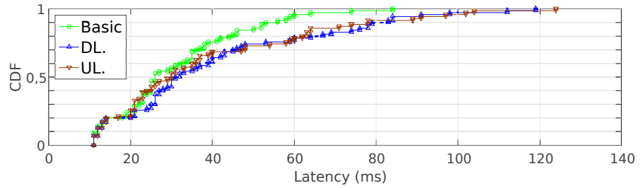
(a) CDF plot of the 95-th percentile of packet latency among real-time flows. 2 \rightarrow 6 elastic flow scenario.
