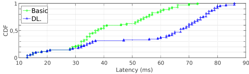
(b) CDF plot of the 95-th percentile of packet latency among real-time flows. 4 \rightarrow 6 elastic flow scenario.
