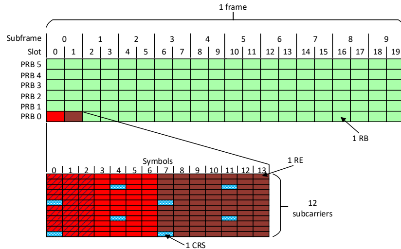
Figure 13 – LTE resource grid for a 1.4MHz (6 PRBs) channel width.
