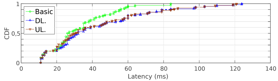
(b) CDF plot of the 95-th percentile of packet latency among real-time flows. 7 \rightarrow 5 elastic flow scenario.
