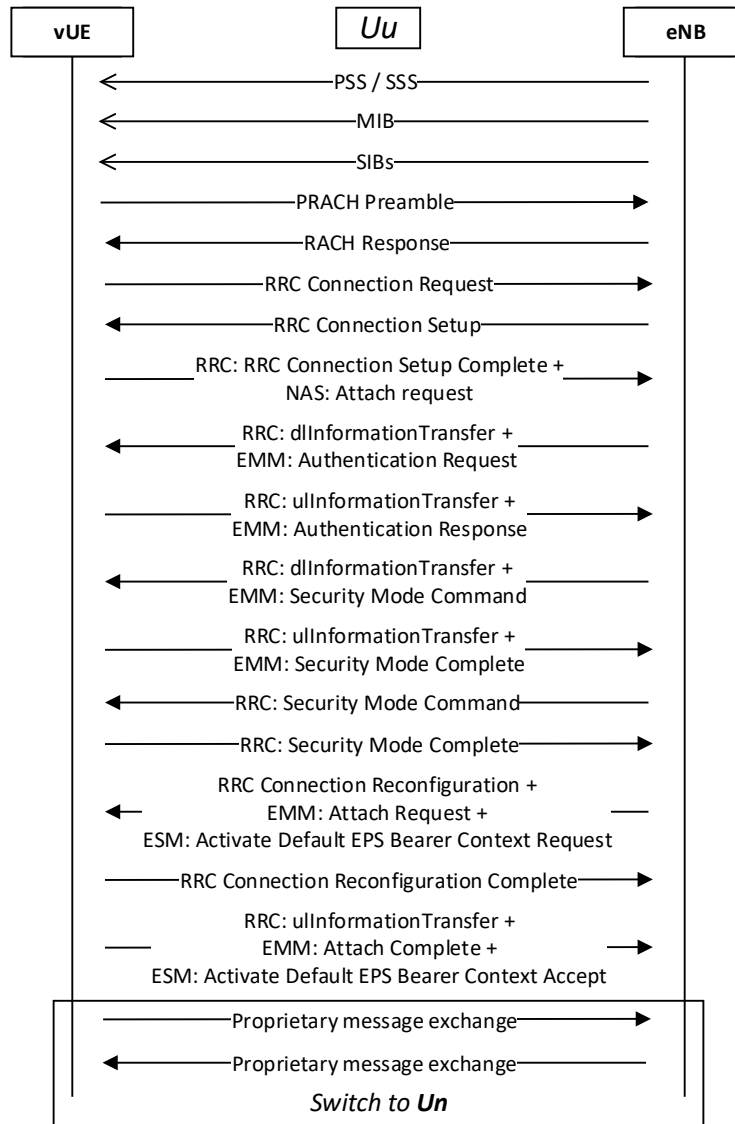
Figure 17 – Connection procedure.
