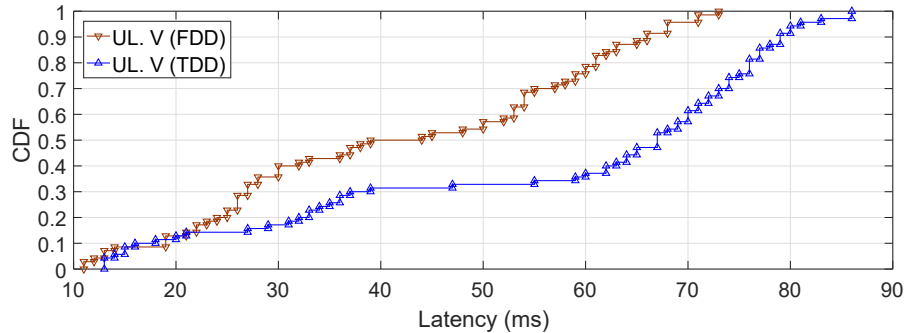
Figure 30 – Hexagonal topology with 7 e2NBs and 70 UEs using 10MHz in TDD mode or 5MHz in FDD mode.
