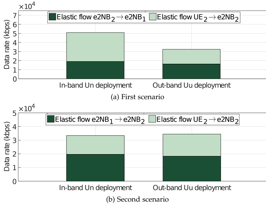
Figure 40 – Cumulated data rate of two traffic flows.
