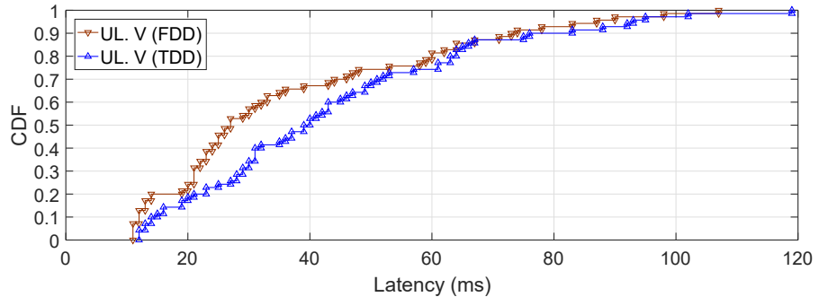
Figure 33 – Line topology with 7 e2NBs and 70 UEs using 10MHz in TDD mode or 5MHz in FDD mode.
