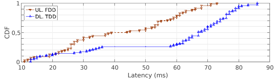
(a) CDF plot of the 95-th percentile of packet latency among real-time flows. 1 \rightarrow 2 elastic flow scenario.
