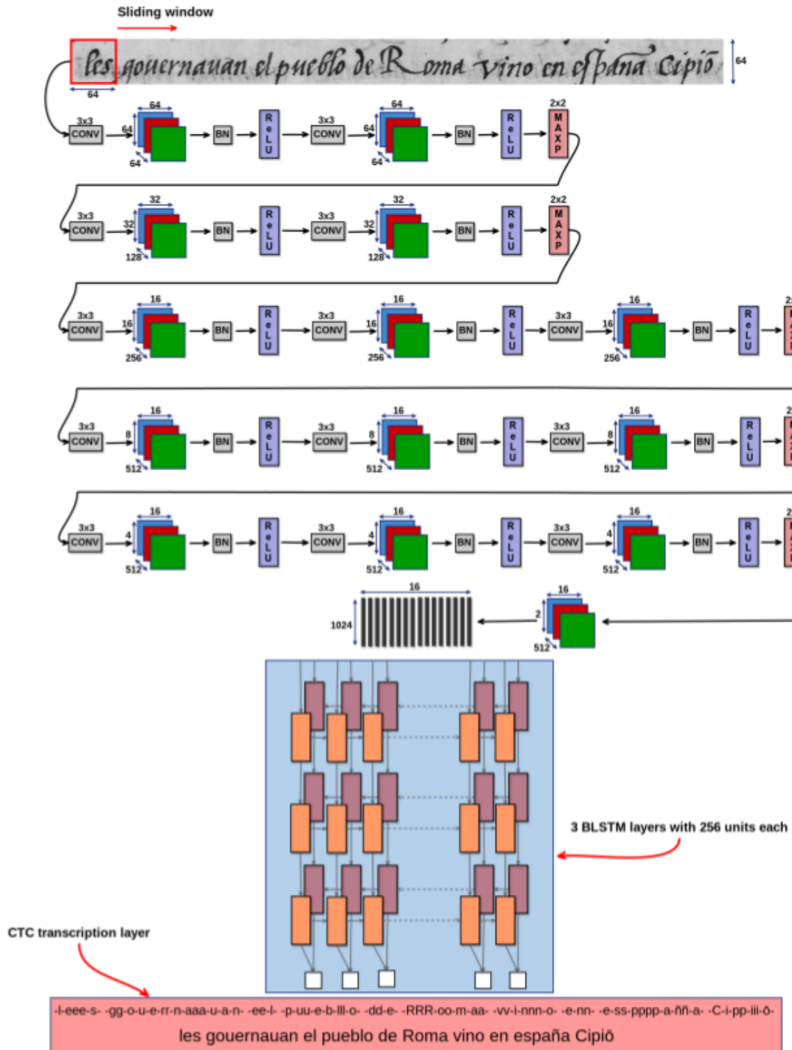
Figure 2.1 – Architecture from [54]. CONV denotes convolutional layers. BN denotes Batch Normalization. MAXP denotes max-pooling.
