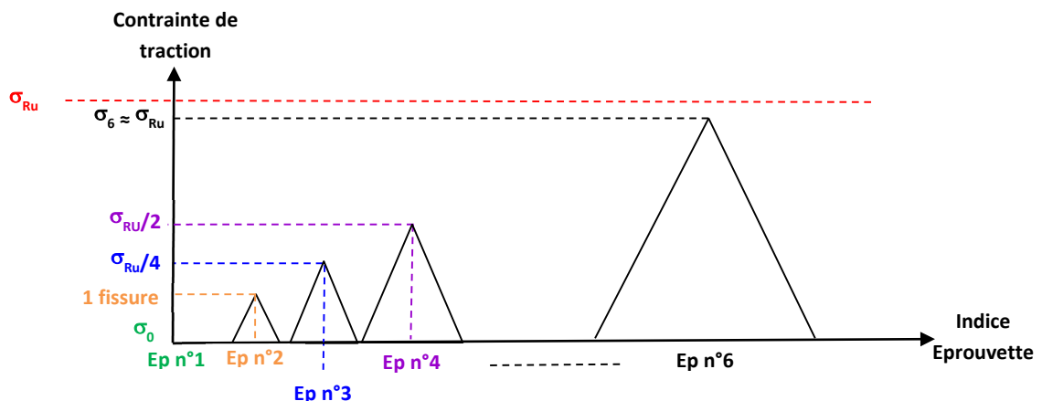
Figure 2.24 – Illustration du protocole de qualification des conditions aux limites.
