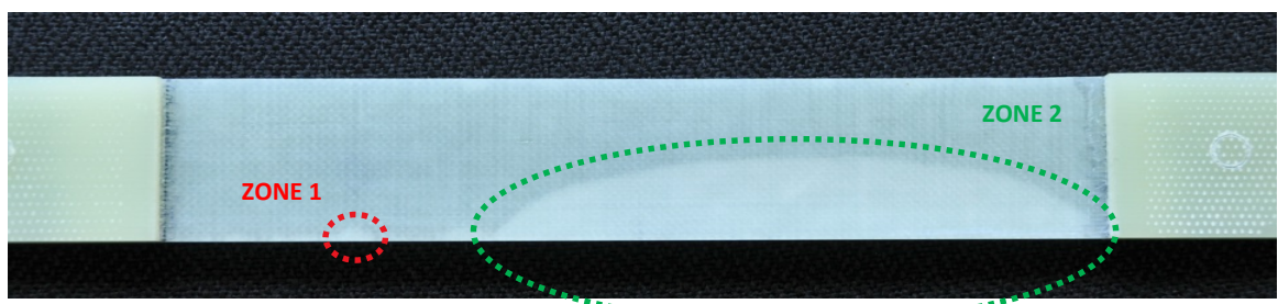
Figure 4.25 – Illustration de délaminages.
