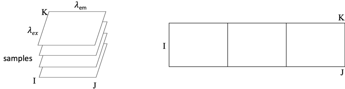
Figure 24. Graphical representation of unfolding a three-way array
