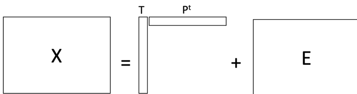
Figure 12. PCA decomposition principle
