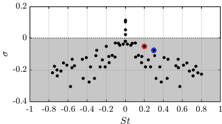
Figure 5.22: Nozzle Flow at NPR = 9 . Eigenspectrum for Global Stability Analysis around the RANS base flow. Two stable modes are visible at St \approx 0.2 and St \approx 0.3 , denoted with a red and a blue empty circle, respectively.
