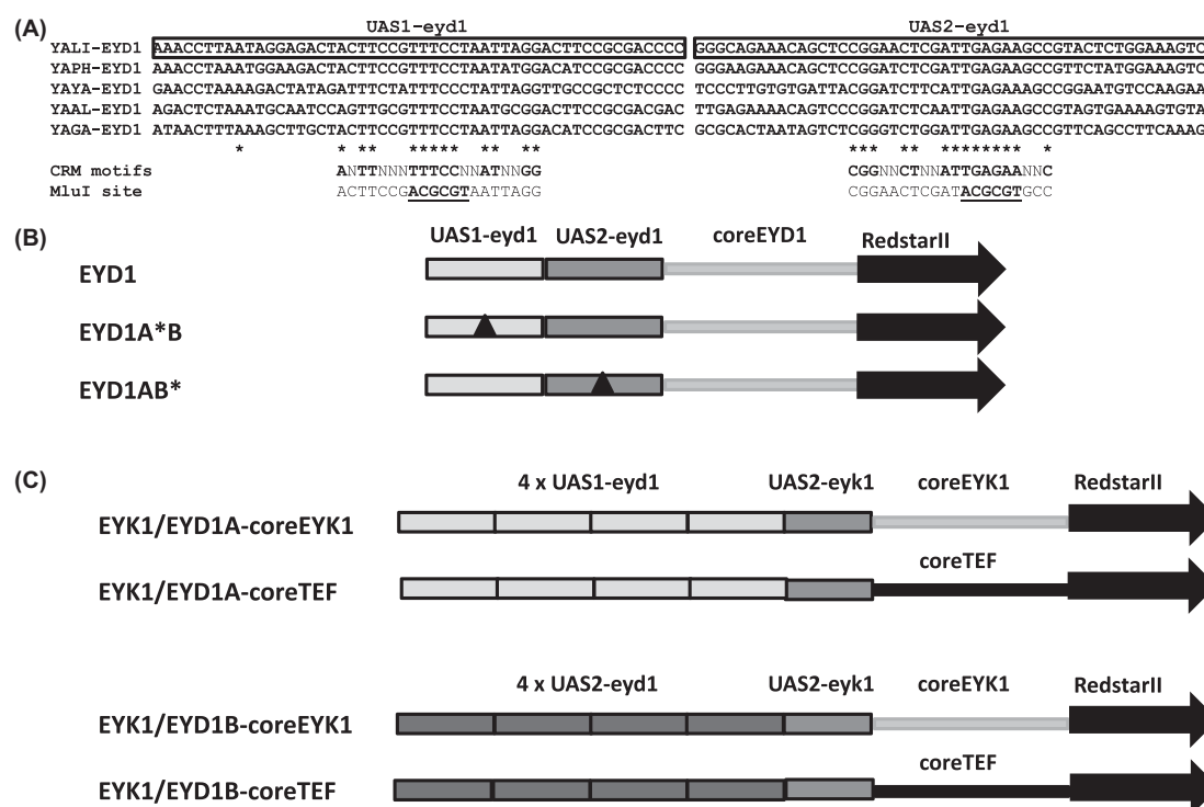
Figure 6. Multiple alignment of the EYD1 UAS and a schematic representation of the mutated and hybrid promoters used in this study. A, Multiple alignment of the UAS1-eyd1 and UAS2-eyd1 motifs of the EYD1 promoter for Y. lipolytica and strains in the Yarrowia clade. The CRMs are indicated with asterisks, and the corresponding CRM consensus sequences are provided. The region containing the UAS1-eyd1 and UAS2-eyd1 motifs used in tandem repeat construction is boxed. B, Schematic representation of the wild-type EYD1 promoter (EYD1) and the mutated EYD1 promoters within the UAS1-eyd1 (EYD1A*B) and the UAS2-eyd1 (EYD1AB*) motifs that controlled the expression of RedStarII. The MluI site used in the mutation of the CRM is shown in panel A. C, Schematic representation of the hybrid EYD1/EYK1 promoters containing either the EYK1 or the TEF core promoter; EYK1/EYD1A-EYK1, four tandem repeats of UAS1-eyd1 + UAS2-eyk1 + coreEYK1; EYK1/EYD1A-TEF, four tandem repeats of UAS1-eyd1 + UAS2-eyk1 + coreTEF; EYK1/EYD2-EYK1, four tandem repeats of UAS2-eyd1 + UAS2-eyk1 + coreEYK1; or EYK1/EYD1B-TEF, four tandem repeats of UAS2-eyd1 + UAS2-eyk1 + coreTEF.
