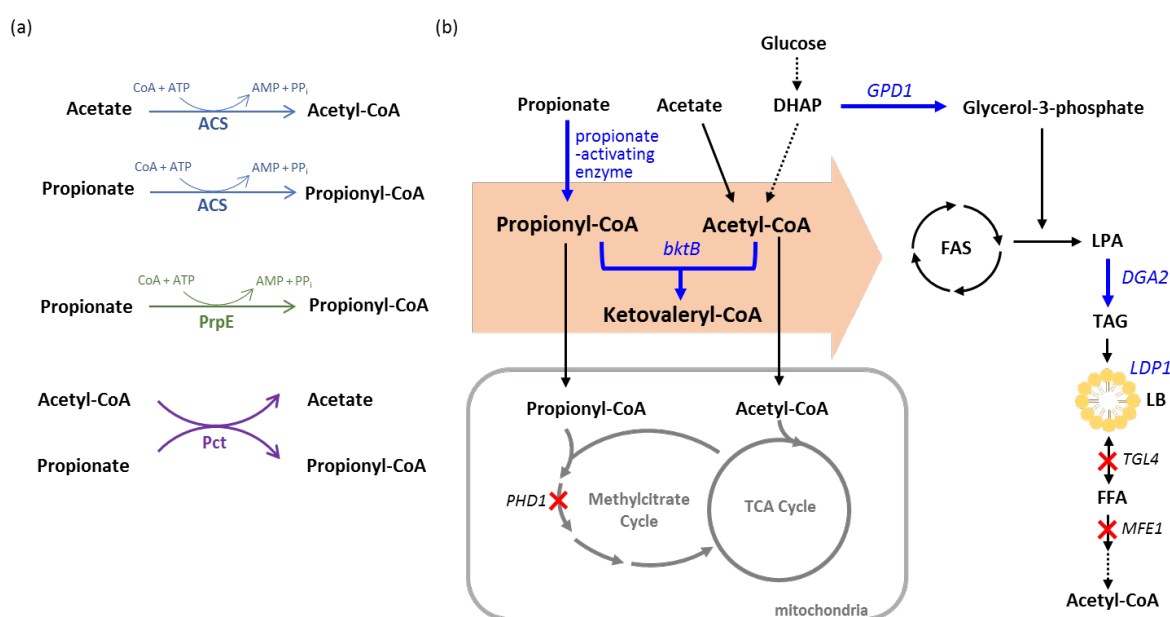
Figure 5.7. Overview of synthesis of lipids including OCFAs in Y. lipolytica . (A) Reaction of propionate activating enzymes used in this study. (B) Overall engineering for OCFa production in this study.
