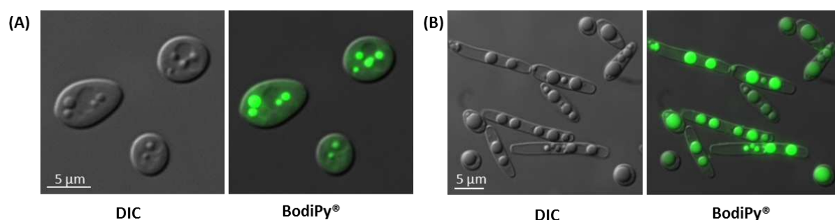
Figure 1.1. The morphology of Y. lipolytica .
