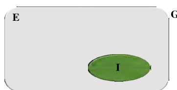
FIGURE 1.4 – Schematic representation of the sub-systems within a QM/MM (or QM/QM') approach. G is the global system, E is the global environment (treated at the MM or QM' level) of I , the part we are interested in (treated at a QM level).
