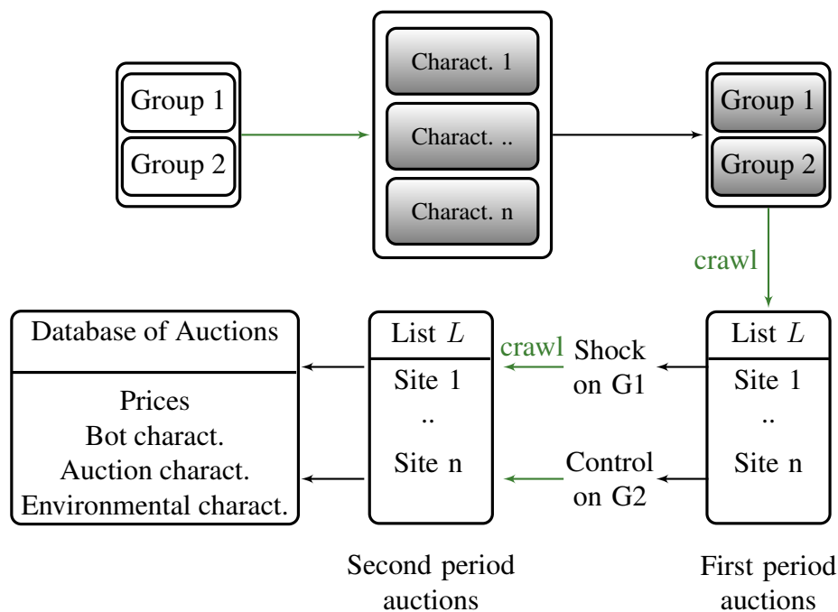
Figure 4.3: Computational process
