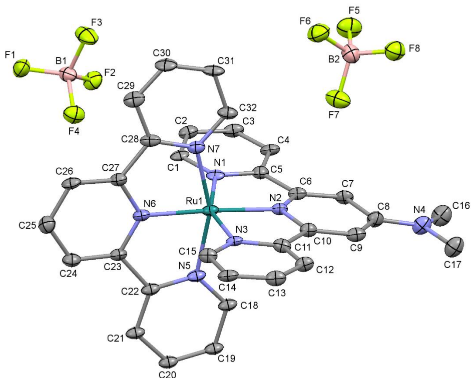
Figure S17. Molecular structures of 6_BPh 4 (top; only one BPh 4 - counterion is presented in the figure) and 7_BF 4 (bottom). Thermal ellipsoids were drawn at the 30 % probability level.
