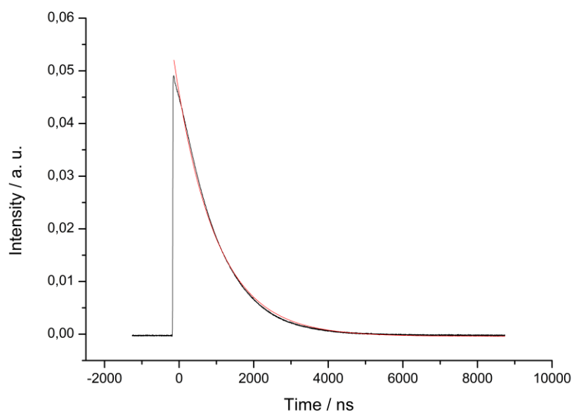
Figure S26. Lifetime spectra of the complexes 6 in aerated (above) and degassed (below) CH 3 CN.
