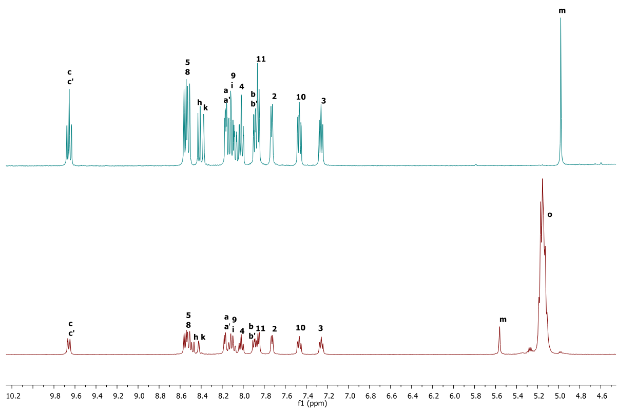
Figure S3. An overlay of 1 H NMR spectra of RuOH (green) and Ru-PLA (red).
