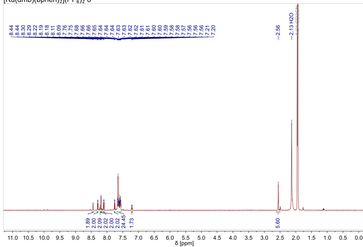
Figure S11. 1 H NMR spectrum of 6 in CD 3 CN, 400 MHz.
