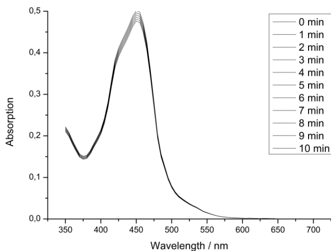
Figure S32. Temporal change of the UV/Vis spectra of [\text{Ru}(\text{bipy})_3]\text{Cl}_2 by irradiation at 450 nm in \text{CH}_3\text{CN} .
