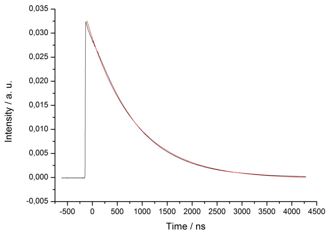
Figure S10. Lifetime spectra of the complex NPs-3 in aerated (above) and degassed (below) H 2 O.
