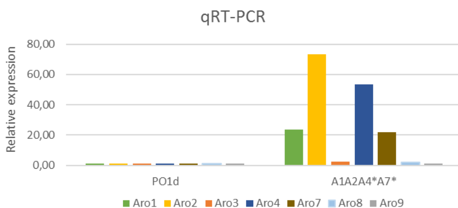
Figure 28. qRT-PCR analysis
