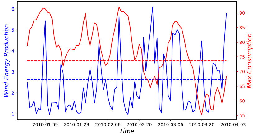
Figure 4.7: Time series of the wind energy production (in blue) and the temperature driven consumption (in red) during winter 2010. Dashed lines show the winter mean climatological value of the wind energy production (in blue) and of the consumption (in red).
