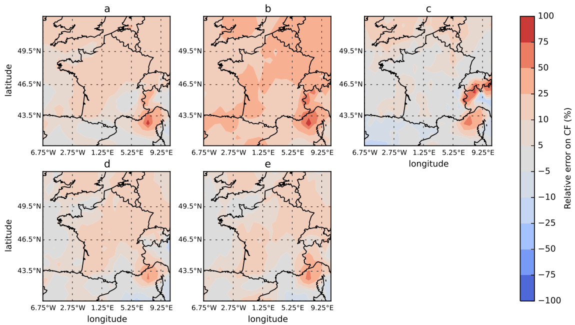
Figure 2.8: Reconstruction of the capacity factor : Relative error on the capacity factor (%) for monthly distributions given by: non parametric climatology (a), parametric climatology (b), Wasp (c), Perc (d), and KCrete (e)
