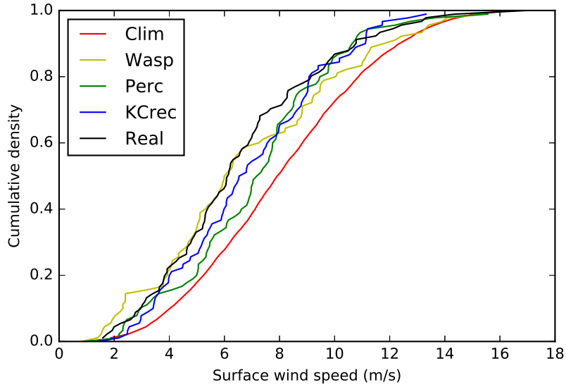
Figure 2.3: CDFs example : ERA-I, ERA-I climatological, and reconstructed seasonal CDFs for winter 2012 at 48.5^{\circ}\text{N} 3.0^{\circ}\text{W}
