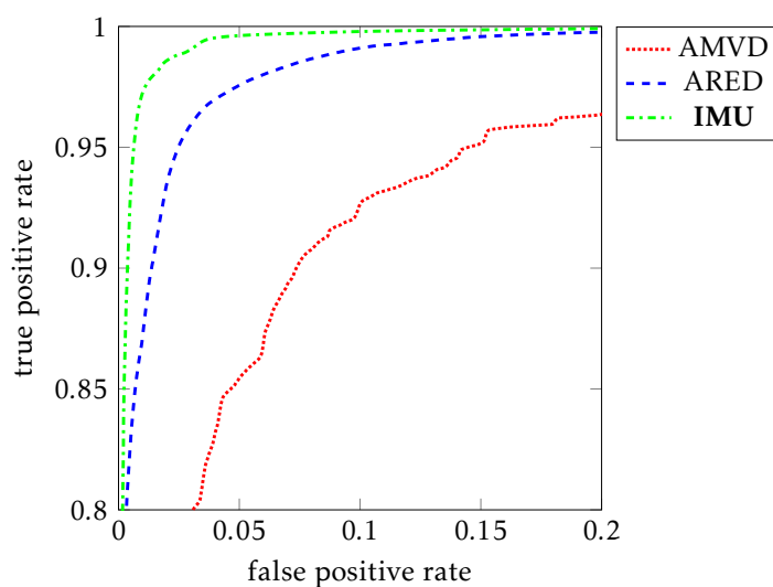
Figure 13.23: Detector results in term of ROC curve for classifying non zero-motion ( z_n^{\text{vel}} = 1 ) from zero-motion ( z_n^{\text{vel}} = 0 ). More the curve approaches the point (0, 1) , better is the classifier. The proposed detectors outperform the conventional classifiers and provide high true positive rate at very low false positive rate.
