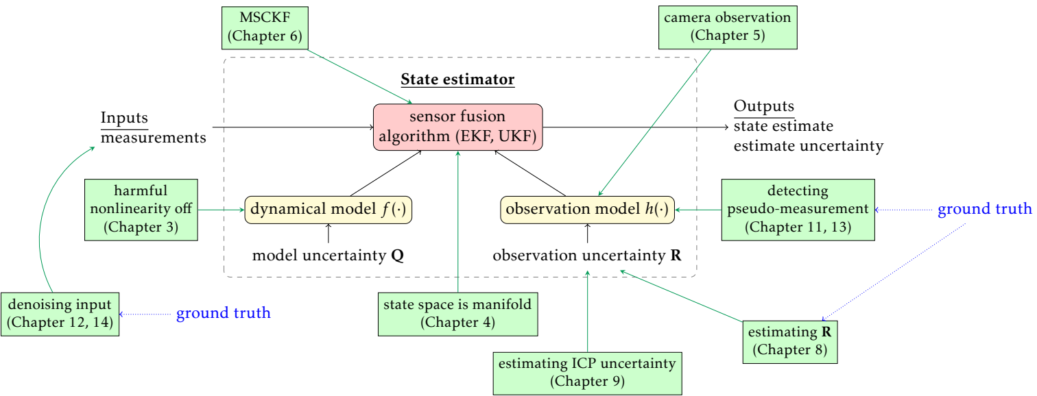
Figure 1.1: Schema of a general state estimation system, along with the contributions of the present thesis (green rectangles). The state estimator computes state estimates along with their uncertainty in function of measurement inputs. The state estimator is divided into a sensor fusion algorithm (red), and models (yellow), where models are parametrized by uncertainty (noise covariance matrices) \mathbf{Q} and \mathbf{R} .
