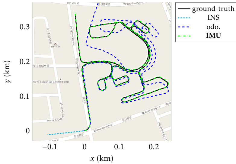
Figure 13.17: Trajectory estimates on the sequence urban07 of the KAIST dataset (2 km, 9 min). IMU is especially accurate on smooth trajectories like in this apartment complex area.
