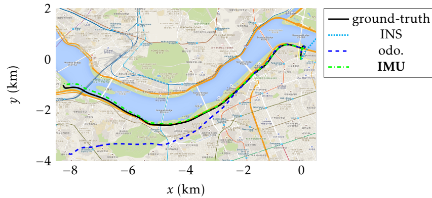
Figure 13.19: Trajectory results on the sequence urban31 of the KAIST dataset (11 km, 15 min). IMU ' results are already impressive on this fast highway sequence, see the slight differences between the proposed methods and the ground-truth at the end of the trajectory.
