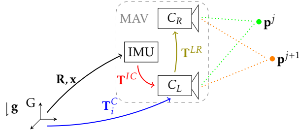
Figure 6.1: The coordinate systems that are used in the chapter. The IMU pose (\mathbf{R}, \mathbf{x}) maps vectors expressed in the IMU frame to the global frame (G). The transformations \mathbf{T}^{IC} and \mathbf{T}^{LR} pass, respectively, from the IMU frame to the left camera ( C_L ) frame, and from the left camera frame to the right camera ( C_R ) frame. The pose \mathbf{T}_i^C consists of the position of C_L in the global frame and the rotation mapping vectors expressed in the C_L frame to vectors expressed in the global frame. Unknown 3D features \mathbf{p}^j (expressed in the global frame) are tracked across a stereo camera system.
