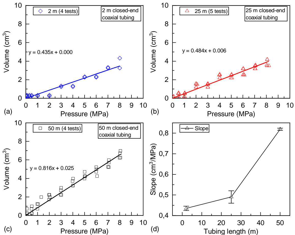
Figure B.2 – Results of tubing self-compressibility tests. (a) 2-meter-long tubing, (b) 25-meter-long tubing, (c) 50-meter-long tubing, (d) synthesis of the compressibility coefficient of all tubes.
