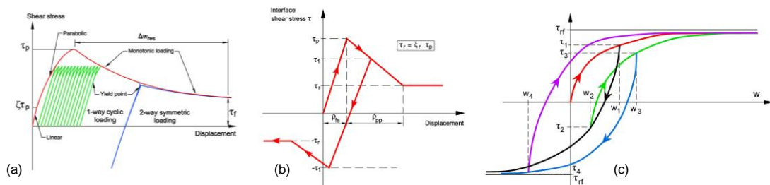
Figure 1.10 – (a) Example of cyclic “ t-z ” load transfer curve from the RATZ method; (b) interface model used in SCARP program; (c) principle of cyclic “ t-z ” curves according to TZC model (adapted from Puech and Garnier (2017))
