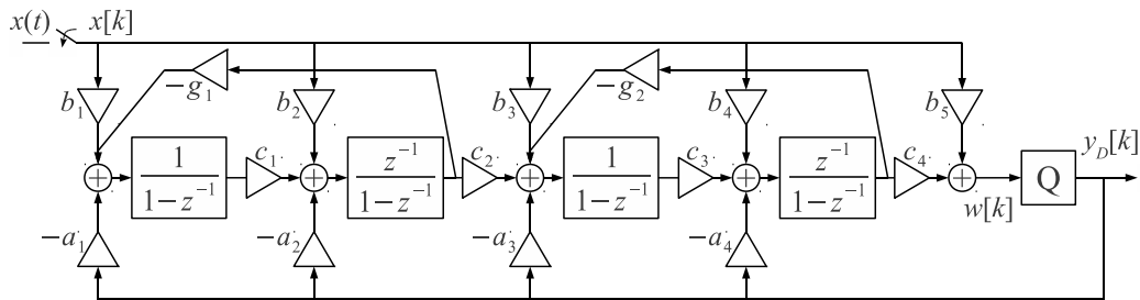
Figure II.10: CRFB architecture
