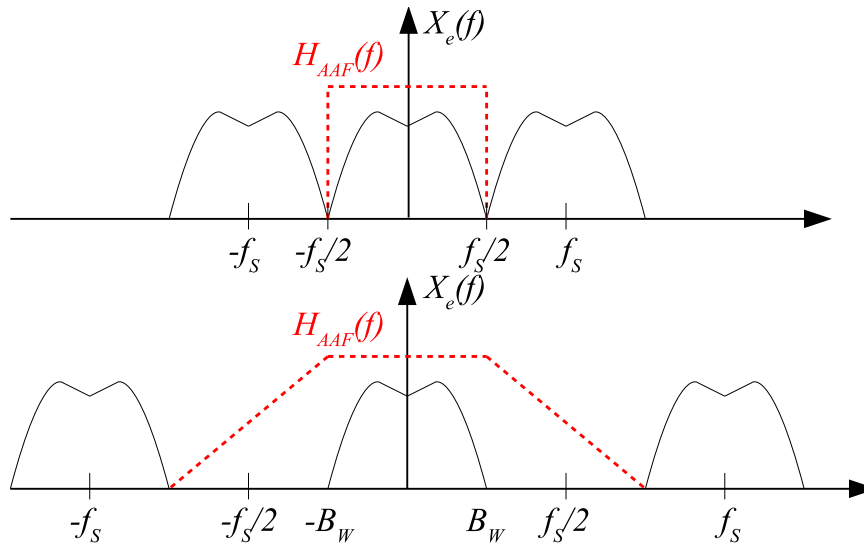
Figure II.1: AAF requirements
