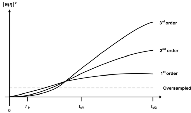
Figure II.7: NTFs obtained with 1 st , 2 nd and 3 rd order loop filters
