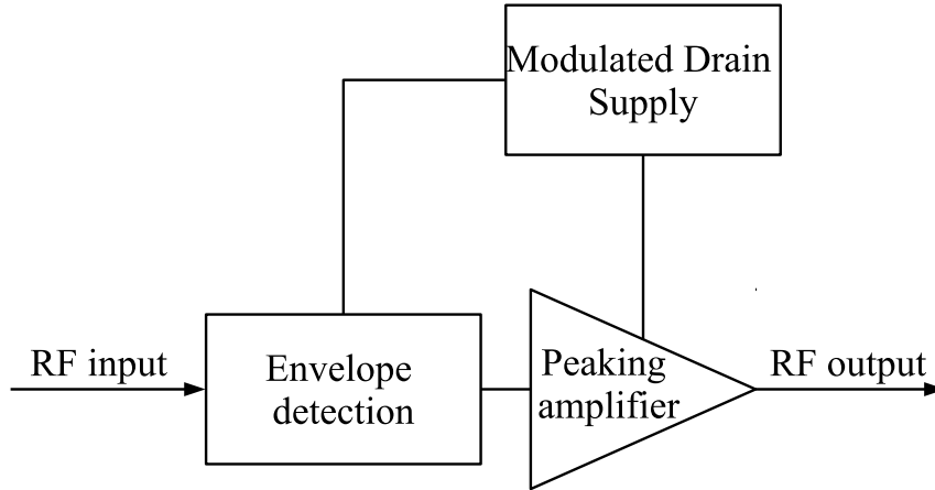
Figure I.2: Enveloppe Tracking PA
