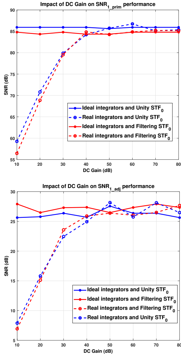
Figure III.3: Effects of finite DC gain on SNR
