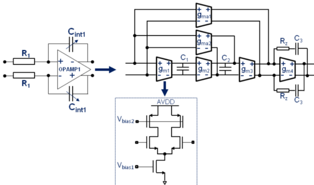
Figure IV.2: OTA schematic [94]
