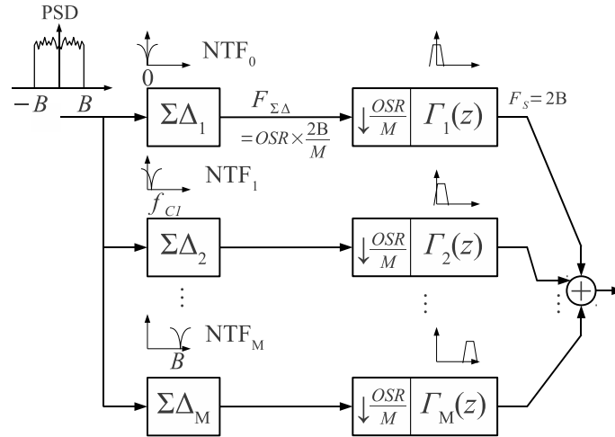
Figure II.13: FBD ADC
