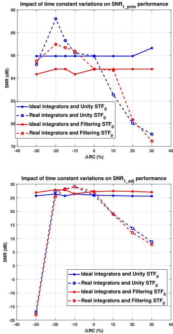
Figure III.5: Effects of RC variations on SNR
