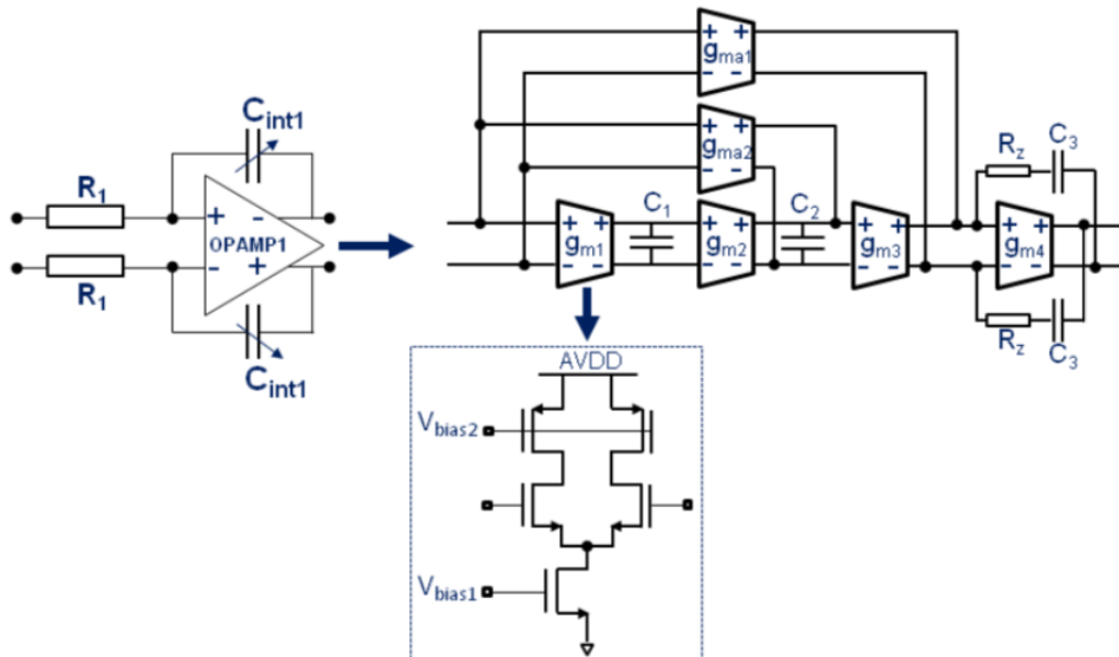
Figure IV.2: OTA schematic [94]
