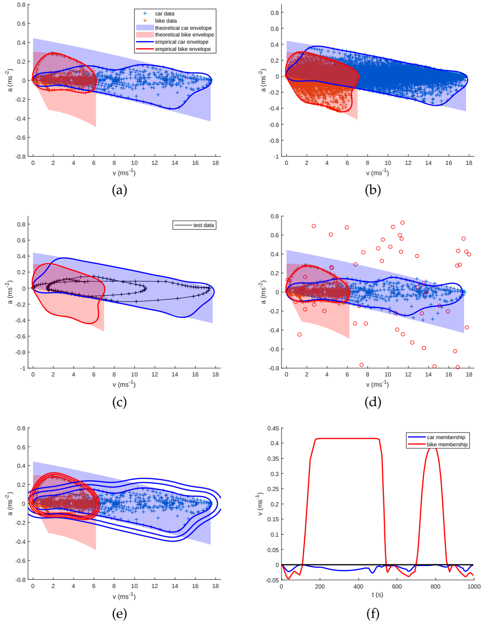
Figure 7.2 – Estimate sets K_{\sigma}^{\text{SVDD}} of theoretical dynamical limits (filled areas) by the SVDD algorithm on simulation data. (a): noiseless case with a small number of data ( \sim 500 pts). (b): noiseless case with a large number of data ( \sim 15\text{k} pts) (c): a test trajectory is compared to the SVDD boundaries. (d): case with noise on the small data and 10% uniformly distributed outliers. The boundaries are mildly altered. (e): applying \sigma -concentric SVDD on the noiseless small data with varying \sigma (100%, 102%, 104% of the previous \sigma ). (f): the indicator functions show that the test trajectory of (c) is a car as the car values are negative while some bike values are positive.
