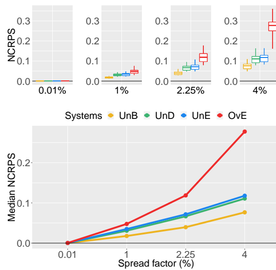
Figure 4.7 – NCRPS score for 1-day ahead synthetically generated forecasts of different quality: unbiased system (UnB, yellow), under-dispersed system (UnD, green), under-estimating system (UnE, blue) and over-estimating system (OvE, red). Systems are based on ensembles generated with four different spread factors (0,01 %, 1 %, 2,25 %, 4 %). Top: boxplots represent the maximum value, percentiles 75, 50 and 25, and minimum value over 10 studied catchments. Bottom: median score value.
