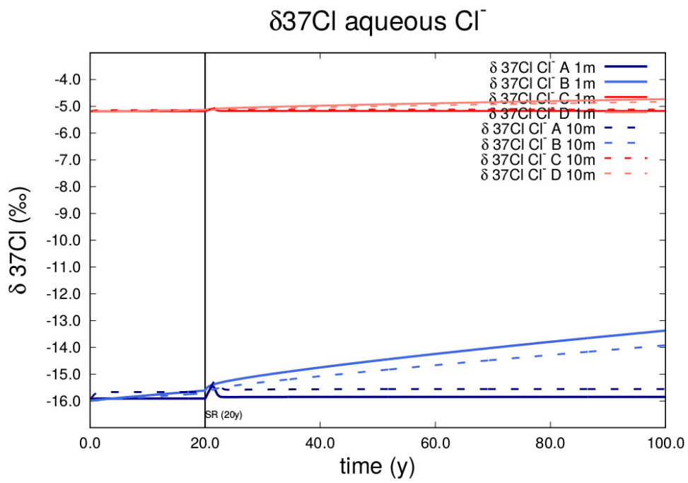
Figure 10: δ 37 Cl of Cl - during reactive transport simulations
