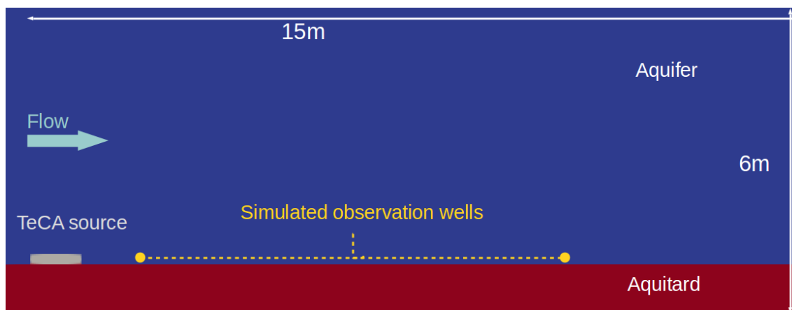
Figure 1: Simulated domain
