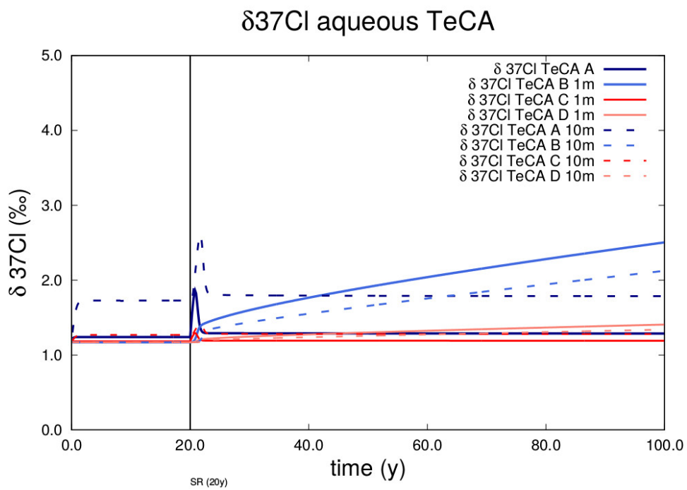
Figure 9: δ 37 Cl of TeCA during reactive transport simulations
