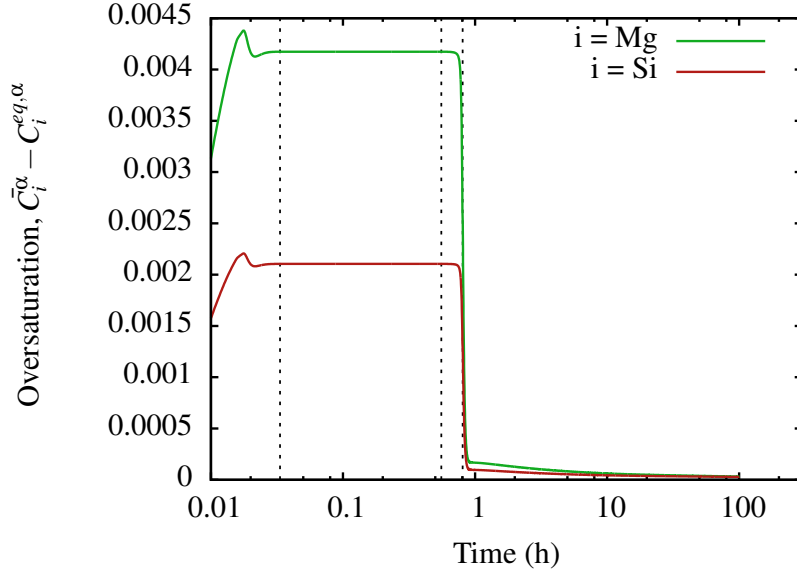
Figure 3.20 – Simulated evolution of the matrix oversaturation for solute elements Mg and Si.
