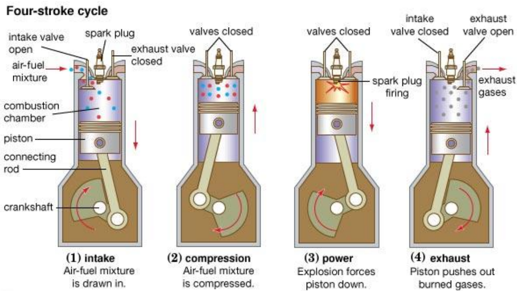
Figure 1.1 – Schematic of the 4 strokes that make up a thermodynamic cycle of a petrol internal combustion engine [14].
