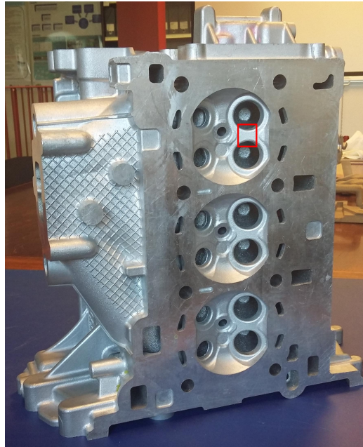
Figure 1.2 – Firedeck side of the cylinder head for the Ford 1.0L 3 cylinder engine with the integrated exhaust manifold (the red square shows the sensitive interval area).
