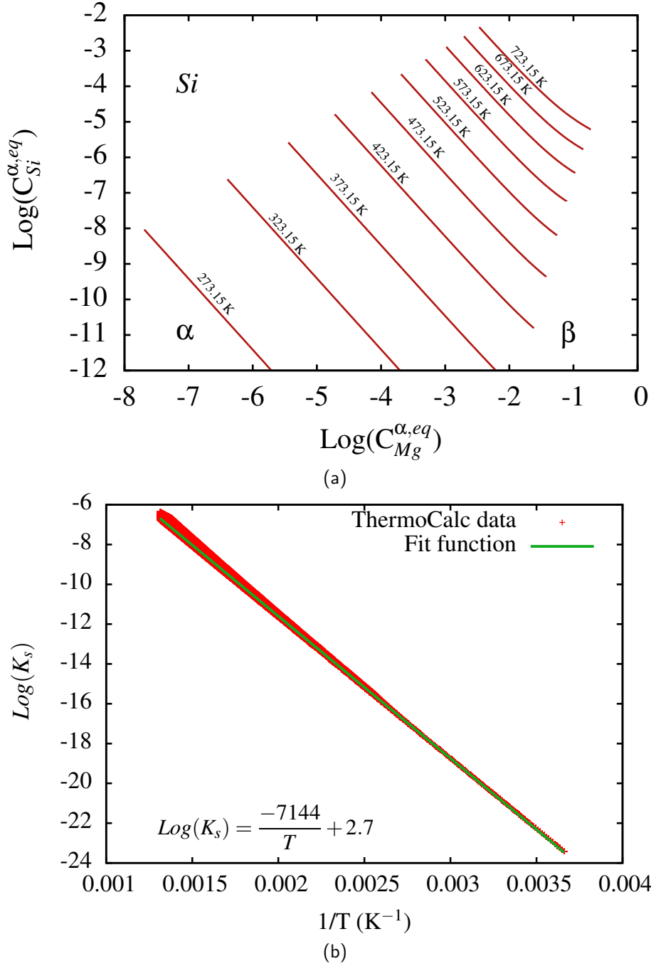
Figure 3.4 – Determination of the solubility product for \beta - \text{Mg}_2\text{Si} using ThermoCalc/TCAL5: (a) Mg and Si concentrations in the matrix for different temperatures representing the phase diagram tie-lines and (b) logarithm of the solubility product K_s as a function of the temperature inverse with the corresponding fit function implemented in the model.
