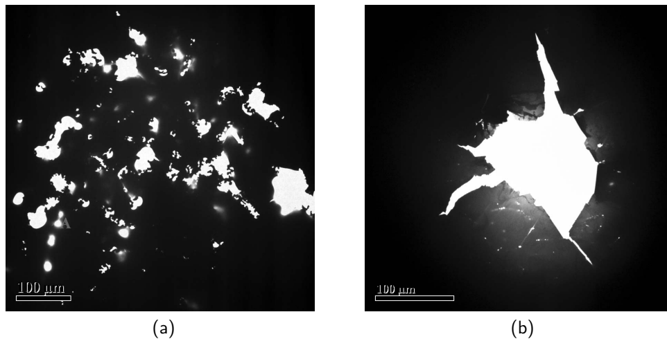
Figure 2.4 – Micrographs showing the result of electrolytic jet polishing : (a) in the studied A356+0.5Cu alloy and (b) in a typical 6xxx series wrought alloy containing less Si.
