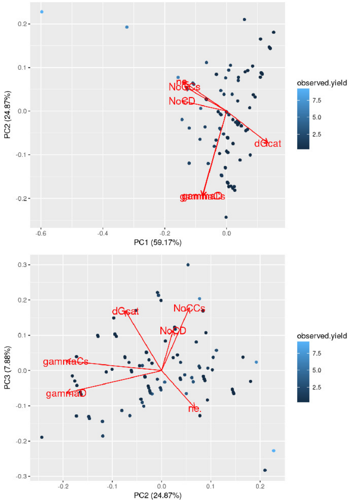
167 Figure 3: PCA plot of the candidate explanatory variables \Delta G_{cat} , ne. , \gamma_D , \gamma_{Cs} , NoC_D and NoC_{Cs} . The upper panel shows PCA axis one (59% of the variance) vs PCA axis two (25% of the variance), and the lower
