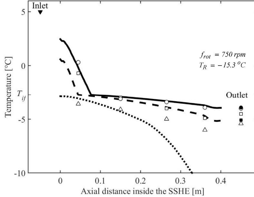
Figure 59. Effect of the mix mass flow rate on the temperature profile along the exchanger: (▼) prescribed value at the inlet, for all the operating conditions (5 °C); measured values for (Δ) \dot{m}_{mix} = 25 kg/h, (□) \dot{m}_{mix} = 50 kg/h, and (○) \dot{m}_{mix} = 75 kg/h; predicted profiles for (....) \dot{m}_{mix} = 25 kg/h, (- -) \dot{m}_{mix} = 50 kg/h, and (—) \dot{m}_{mix} = 75 kg/h; and surface-averaged values at the exit for (■) \dot{m}_{mix} = 50 kg/h and (●) \dot{m}_{mix} = 75 kg/h.
