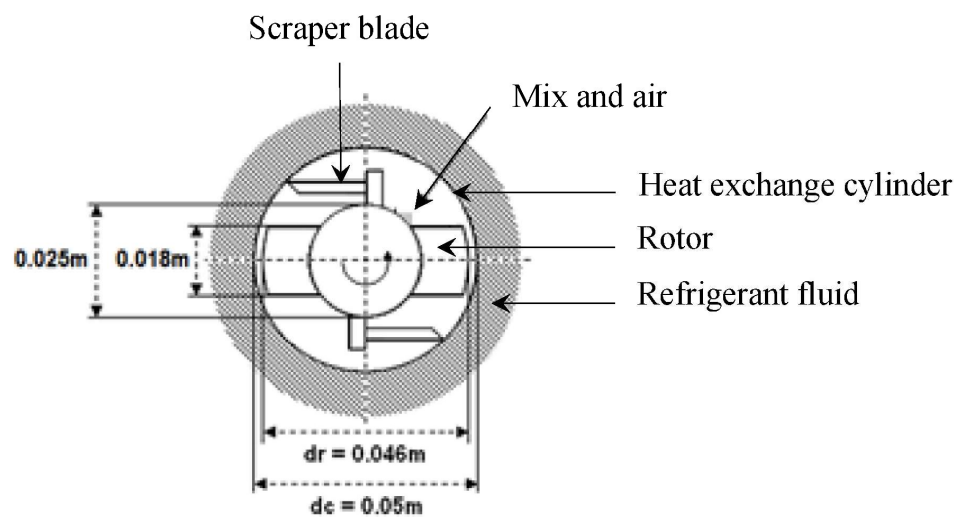
Figure 41. Schematic representation of the pilot Freezer WCB MF 50: (a) side view (b) cross section.
