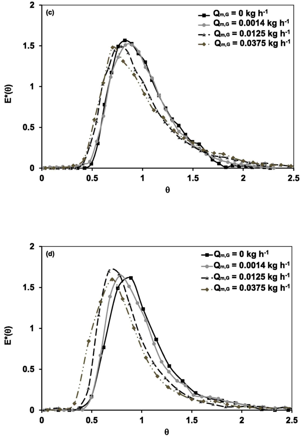
Figure 42. Effect of mix and air flowrate on the liquid phase RTD inside the SSHE – T_{\text{refrigerant}} \approx -15^\circ\text{C} : (a) 25 \text{ kg h}^{-1} of mix; (b) 50 \text{ kg h}^{-1} of mix; (c) Dimensionless E -curve for 25 \text{ kg h}^{-1} of mix; (d) Dimensionless E -curve for 50 \text{ kg h}^{-1}
