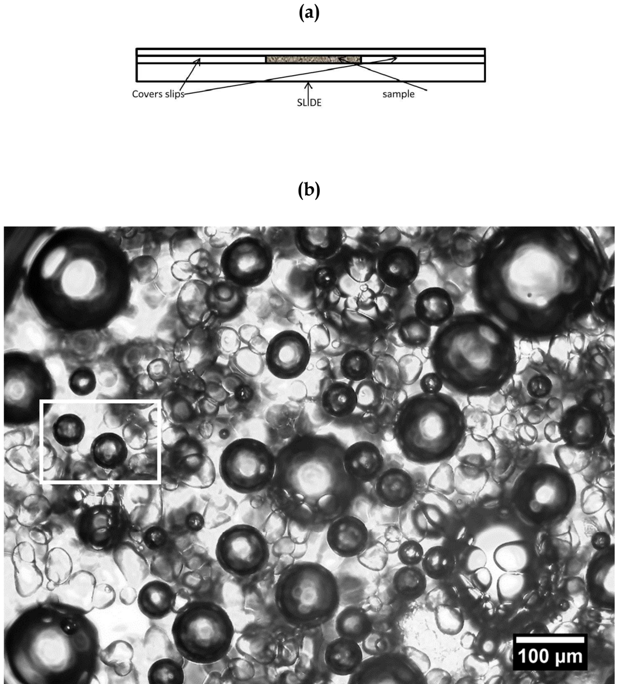
Figure 33. Example of sorbet CSD and BSD measurement procedure obtained at \dot{m}_{air} = 0.0116 \text{ kg h}^{-1} , T_R = -19.3^\circ\text{C} , f_{rot} = 500 \text{ rpm} and P = 5 \text{ bar} . (a) Slides with two glued slips pieces; (b) Sample of image; (c) illustration of bubble and crystal measurement, top: bubble identification and diameter outline, bottom: crystal identification and drawing; (d) cumulative distributions; (e) frequency plot.
