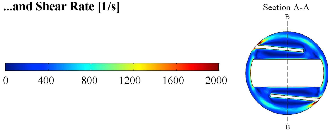
Figure 54. Views of the profiles in the SSHE as predicted by the numerical model under reference operating conditions: \dot{m}_{mix} = 50 \text{ kg/h} , T_R = -15.3 \text{ }^\circ\text{C} and f_{rot} = 750 \text{ rpm} : A) velocity magnitude (top) and shear rate (bottom), B) pressure, C) temperature, D) enthalpy and ice fraction, and E) viscous dissipation rate.
