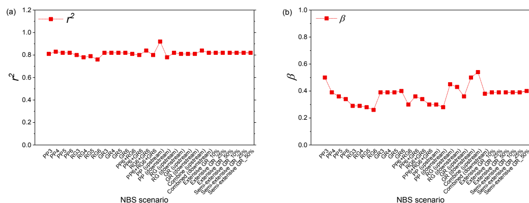
Figure 5.12: r^2 (a) and \beta (b) of spectral analysis of the last time step of the simulated overland flow of NBS scenarios under the EV14S.
