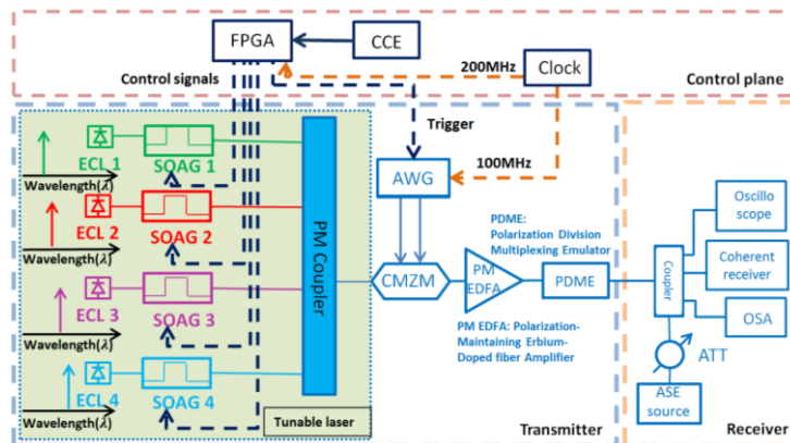
Figure 3-25: Experimental set-up for the back-to-back evaluation of the transmitter and receiver
