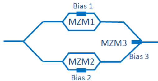
Figure 3-14: CMZM structure
