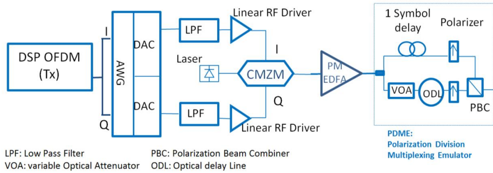
Figure 3-13: Transmitter experimental set-up.
