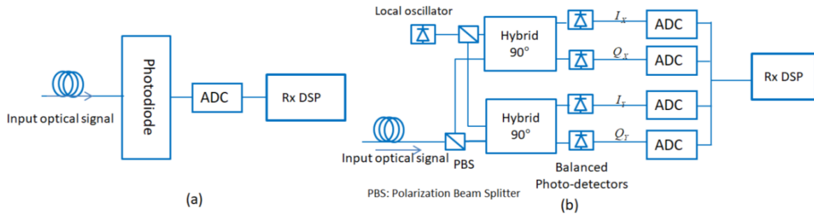
Figure 1-3: The architecture of (a) direct detection and (b) coherent detection technologies.
