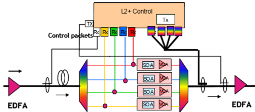
Figure 1-14: POADM node structure [74].
