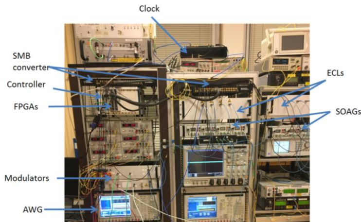
Figure 4-2: Experimental test-bed.
