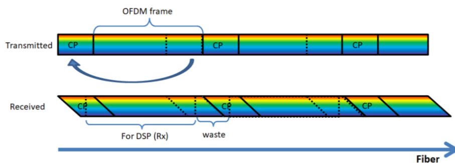
Figure 3-18: OFDM symbol with cyclic prefix in the time domain
