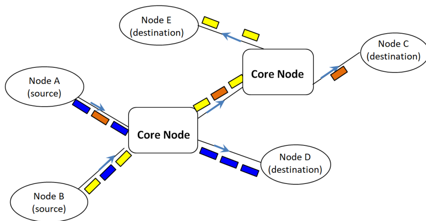
Figure 1-16: TWIN basic architecture
