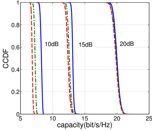
Figure 2.6: Capacity CCDF with CSI (solid), \overline{C_{Si}} (dash-dot) and e_p (dashed) for SNR=10,15,20 dB and MDL = 15dB
