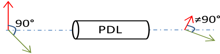
Figure 1.15: Loss of orthogonality and power imbalance due to PDL.
