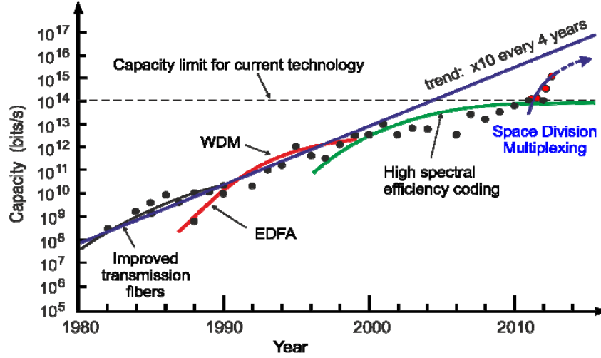
Figure 1.3: The evolution of transmission capacity of optical fibers over the years. Figure taken from [2].
