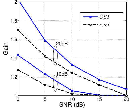
Figure 2.7: C_{Si} gain (solid), \overline{C_{Si}} gain (dashed) as a function of SNR for MDL = 10, 20 dB for a 6-mode fiber.
