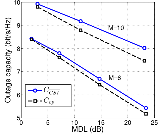
Figure 2.9: Outage capacities vs MDL for M = 6, 10 modes. \overline{C_{CSI}} (solid) and C_{ep} (dashed) for SNR = 10dB.
