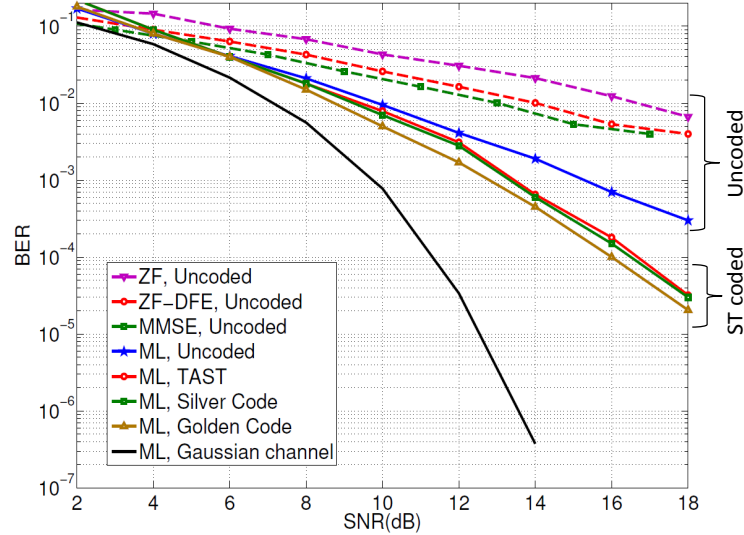
Figure 3.2: BER performance for different decoders for an uncoded and ST coded 2 \times 2 Rayleigh fading channel.
