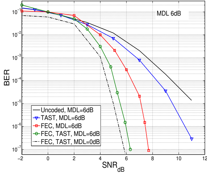
Figure 3.7: Performance of a 3-mode fiber in term of BER for the uncoded scheme and with TAST code, LDPC code, and the concatenation of both codes for MDL = 6 dB.
