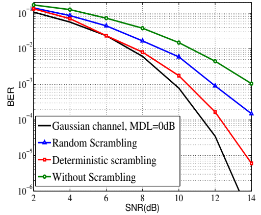
Figure 2.17: BER performance of 6-mode fiber, \sigma_{x,y} = 4\%r_c
