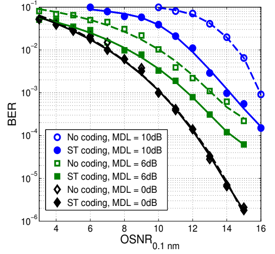
Figure 4.14: BER vs OSNR for ST coded and uncoded systems, MDL= 0, 6, 10 dB
