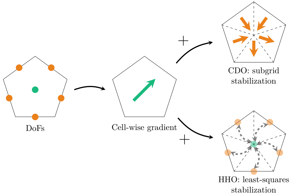
Figure 1.5 – Comparison between gradient reconstructions of a scalar function in 2D for CDO and HHO( k = 0 ). Face- and cell-based quantities are shown, respectively, in orange and green. The two reconstructions share a common consistent (exact for affine functions) gradient. However, in CDO the gradient is enriched with a piecewise constant stabilization, constant on a subdivision of the cell. In HHO( k = 0 ), the gradient is constant on the whole cell and it is sought among the gradients of affine functions, and a penalty is added to the bilinear formulation.
