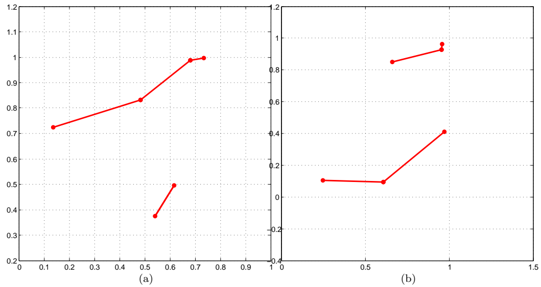
Figure 7.2: Two different sets of K = 6 atoms, for which the property (1) does not hold. (a) None of the atoms from the pair in MNMR are the nearest neighbor of the remaining atoms. Hence, this pair is not connected to the rest. (b) The atoms of each triplet have their nearest neighbor within the same group. Hence, the atoms of one triplet are not connected with those from the other triplet.
