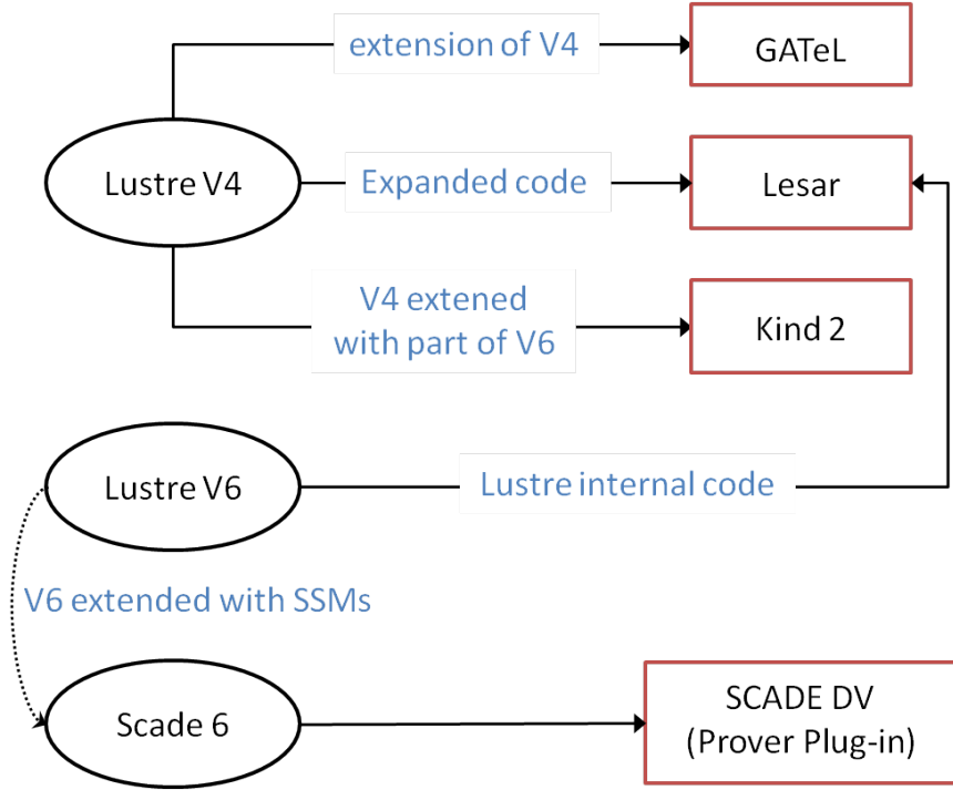
Figure 2.11: Model checking tools for Lustre and Scade
