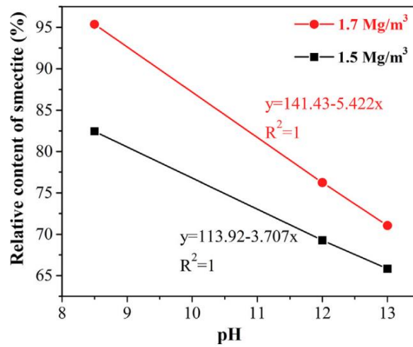
Figure 1-27. Variation of dissolved montmorillonite with pH of GMZ bentonite (Sun et al., 2019b).
