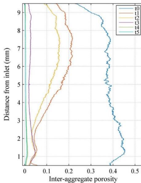
Figure 1-9. Profile of inter-aggregate porosity deduced from \mu\text{CT} images at different times ( t_1=7.1 days, t_2=8.8 days, t_3=15.8 days, t_4=19.7 days, and t_5=39.8 days) (Massat et al., 2016).
