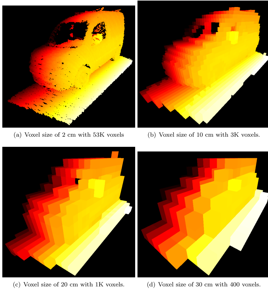
Figure 2.16: Voxelization of a car varying voxel size. Color scale corresponds to x coordinate of voxels center.
