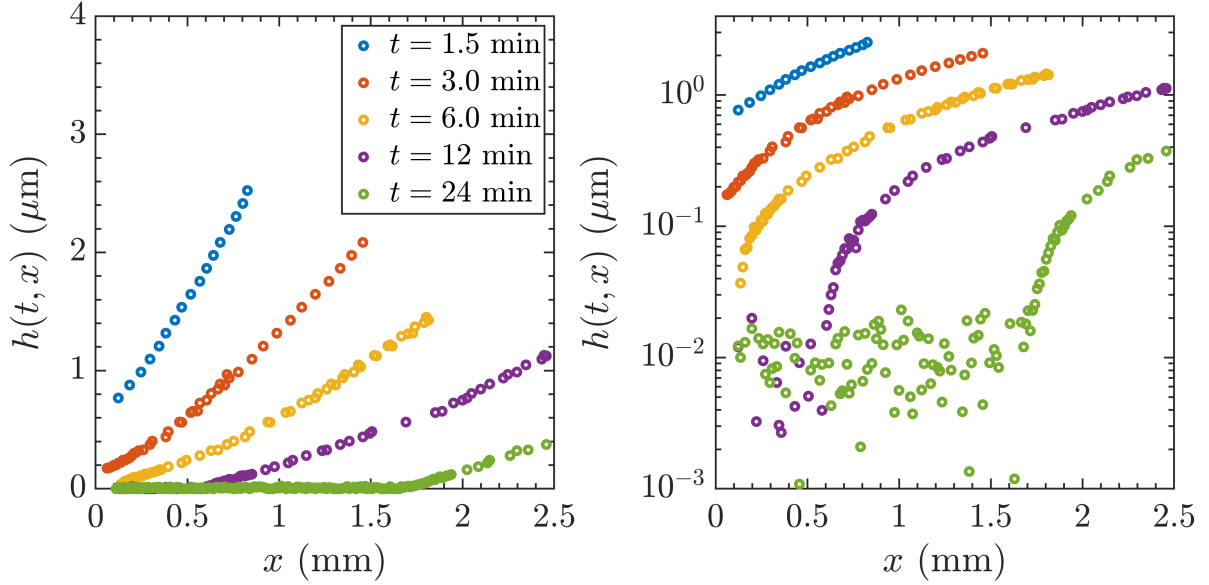
Figure 4.7: Left panel: experimental thickness profiles of HMN in an experiment of initial thickness h_0 = 19(1)\mu\text{m} and dissipated power P = 1.18(1)\text{mW} . Right panel: same profiles in a semilogarithmic plot.
