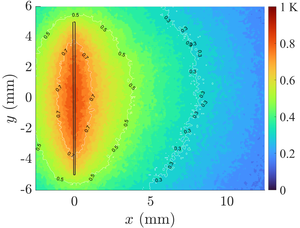
Figure 2.3: Example of thermal field \theta(\mathbf{x}) obtained with the infrared camera. In this case, the dissipated power is P = 2.56(3) mW. The rectangle indicates the position and size of the heating line. The maximum temperature attained is \theta_{max} \simeq 0.82 K.
