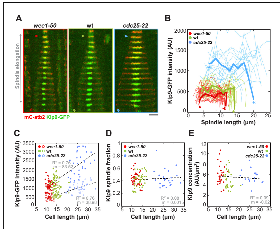
Figure 4. The total number of Klp9 molecules and the number of motors on anaphase spindles increase with cell size. (A) Time-lapse images of wee1-50 , wild-type (wt) and cdc25-22 cells expressing mCherry-Atb2 (tubulin) and Klp9-GFP from anaphase onset (arrowhead) to spindle breakdown (asterisk). Each frame corresponds to 1 min interval. Scale bar, 5 \mu\text{m} . (B) Comparative plot of Klp9-GFP intensity over spindle length. Each line corresponds to the Klp9-GFP intensity values of one cell throughout progressing spindle elongation in anaphase. Bold curves correspond to a representative cell of each cell type. (C) Total Klp9-GFP intensity and Klp9-GFP intensity at anaphase spindles (O, unfilled dots) plotted against cell length ( wee1-50 : n = 48 , wt: n = 46 , cdc25-22 : n = 30 ). Shown values of Klp9-GFP intensity of anaphase spindles correspond to the mean intensity values of late anaphase. (D) Ratio between Klp9-GFP intensity at the anaphase spindle and the total Klp9-GFP intensity, referred to as Klp9 spindle fraction, plotted against cell length ( wee1-50 : n = 48 , wt: n = 46 , cdc25-22 : n = 30 ). (E) Ratio of total Klp9-GFP intensity and cell volume plotted against cell length ( wee1-50 : n = 30 , wt: n = 29 , cdc25-22 : n = 17 ). Data in (C–E) was fitted by linear regression (dashed lines), showing the regression coefficient R^2 and the slope m . Data obtained from n cells was collected from three independent experiments.
