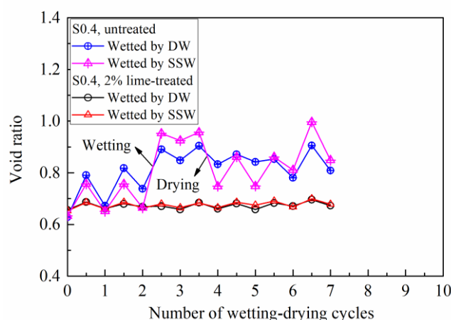
Fig. 3. Void ratio variations during wetting-drying cycles.
