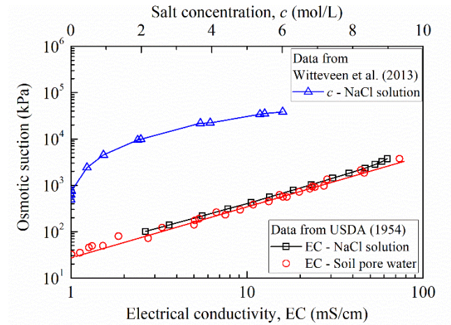
Figure 1-9. Relationship between osmotic suction and electrical conductivity/salt concentration.
