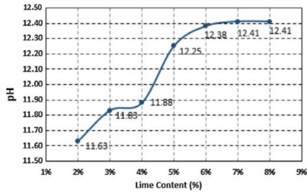
Figure 1-4. pH variations with seawater-lime mixtures (Emarah and Seleem, 2018).
