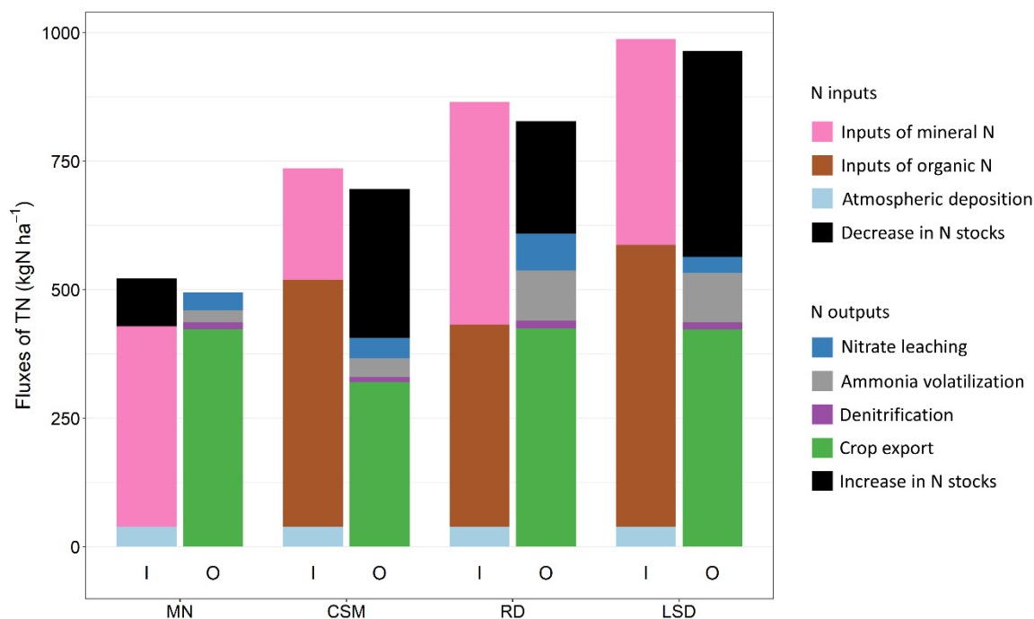
Figure 4.6 – Simulated fluxes of N in the field, during the 3-year crop rotation. Inputs of total N are on the the left (I), and output of N in the right (O). The variation of N stocks include soil organic N, SMN, and N in fresh crop residues. We observed a decrease in N stocks in MN treatment, and an increase in N stocks in CSM, RD, and LSD treatments (higher inputs than outputs).
