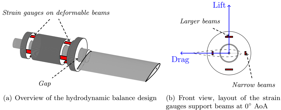
Figure 2.17: Hydrodynamic balance
