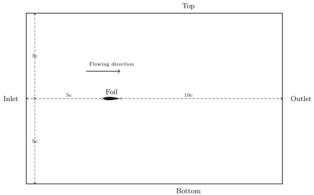
(a) Dom1 , unconfined
