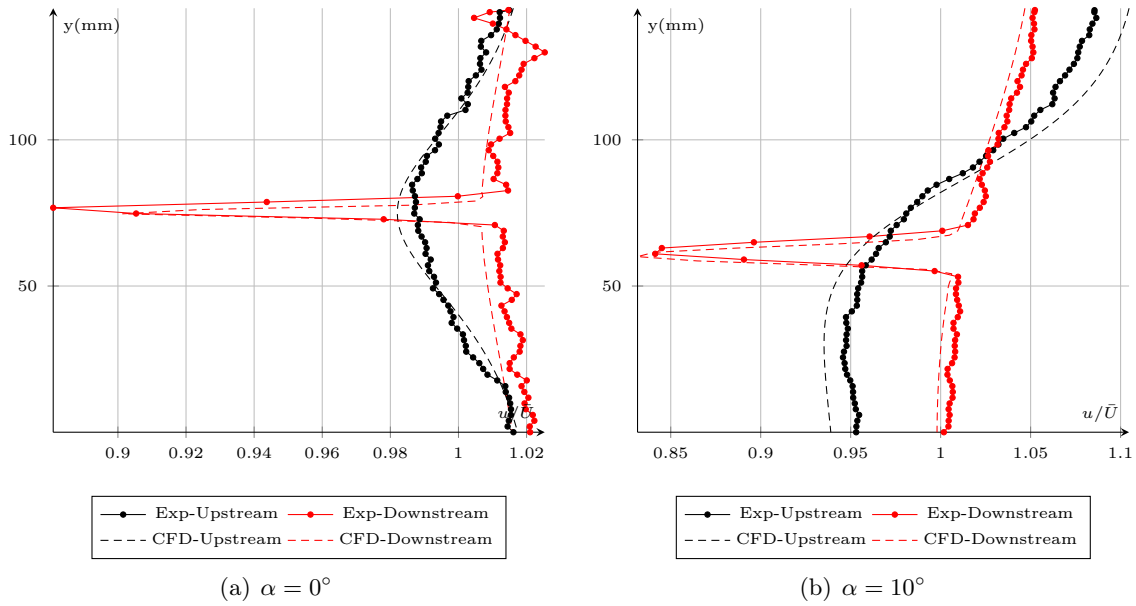
Figure 3.16: Comparison of the upstream and downstream velocity profiles for the NACA 0015, obtained through calculation and PIV measurements, Re_c \simeq 5 \times 10^5 .
