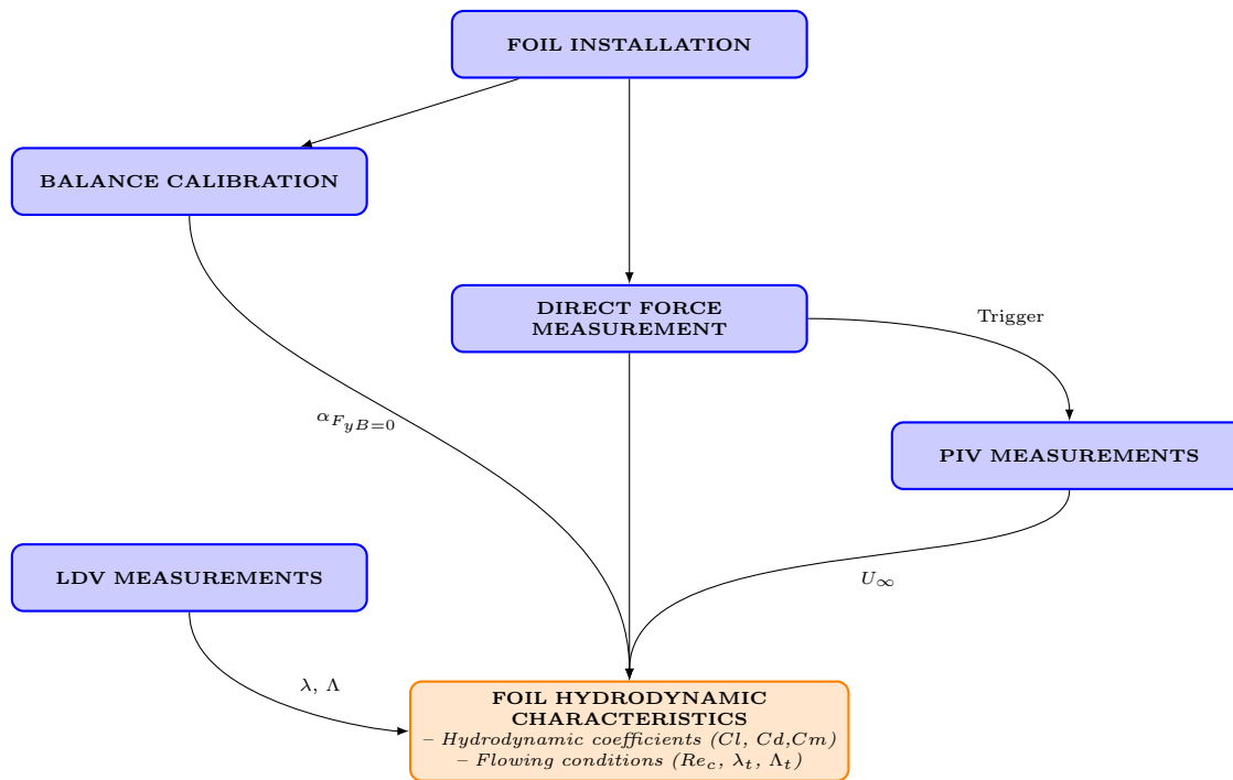
Figure 2.39: General measurement protocol
