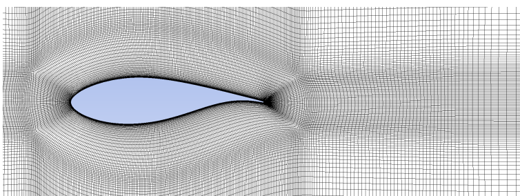
(b) Foil section and close wake
