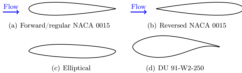
Figure 1: Foil configurations
