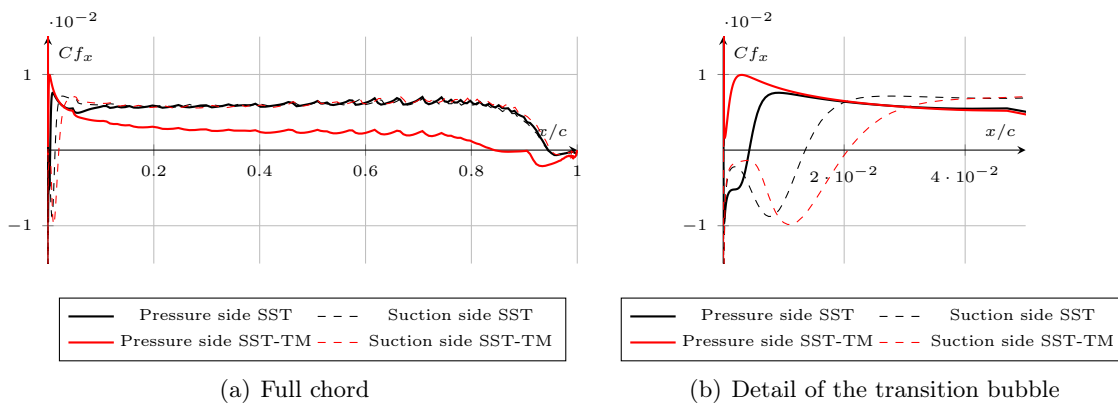
Figure 4.13: Evolution of the friction coefficient (x axis – flow axis) along the foil chord, numerical results 2-D, \alpha = 0.5^\circ and Re_c = 5 \times 10^5 .
