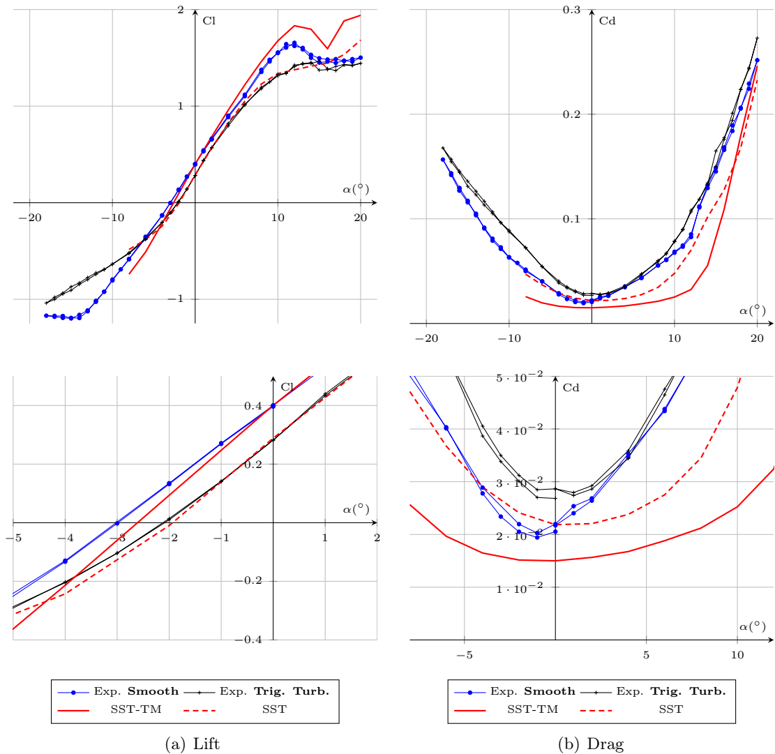
Figure 5.2: Experimental and numerical data for lift and drag coefficients. DU foil section at Re_c = 5 \times 10^5 .
