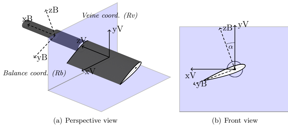
Figure 2.19: Relative positioning of Veine and Balance coordinate frames.
