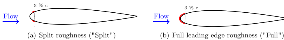
Figure 2.10: Turbulence-triggering roughness strategies.
