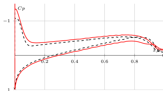
(a) \alpha = 0.5^\circ
