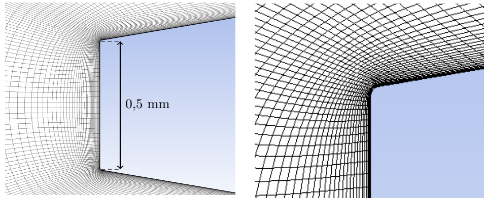
(a) Close leading edge mesh. Front face is 0.5 mm in height. (b) Focus on the leading edge mesh, geometry sharpness.
