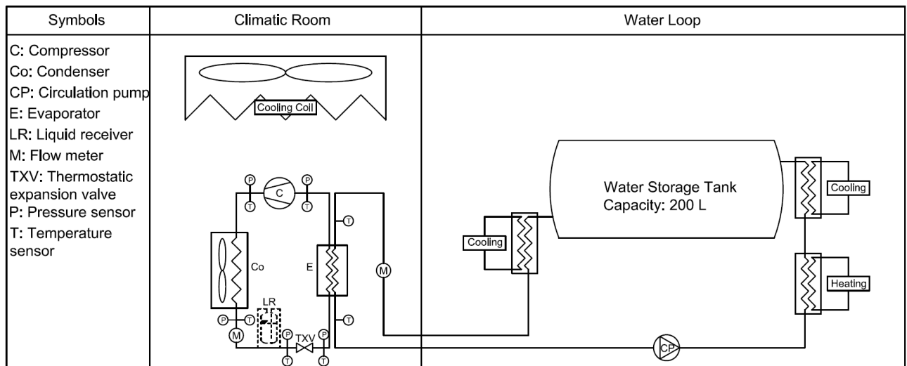
Figure 1: Experimental setup for the climatic room, the water loop and water chiller.
