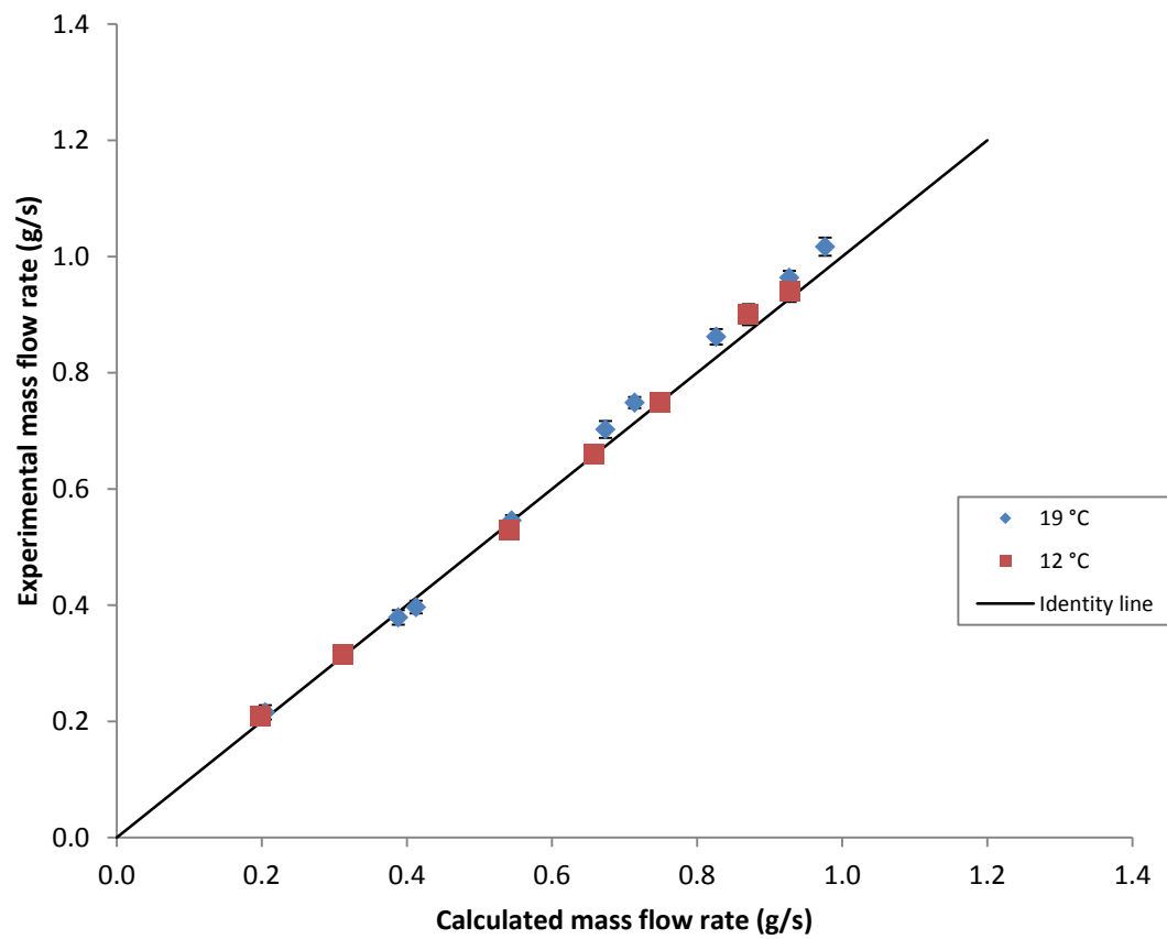
Figure 35: Experimental and calculated mass flow rate according to equation (70) for the atomizer of 410 μm orifice diameter.
