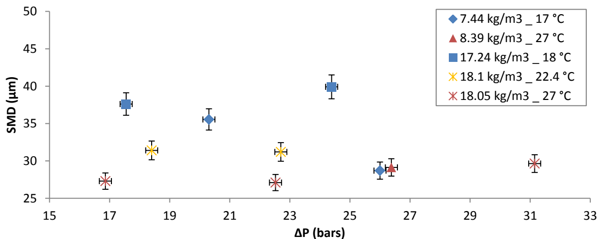
Figure 45: D_{32} diameters measured under different experimental conditions for the atomizer of 100 \mu\text{m} orifice diameter.
