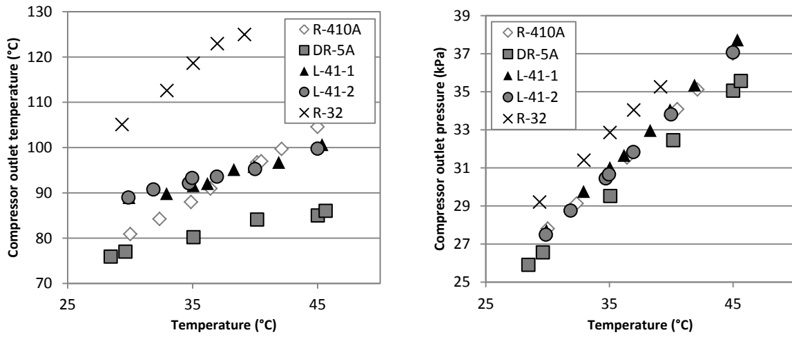
Figure 3: Compressor outlet temperature (°C) and relative pressure (x100 kPa) comparison for the chiller without liquid receiver.
