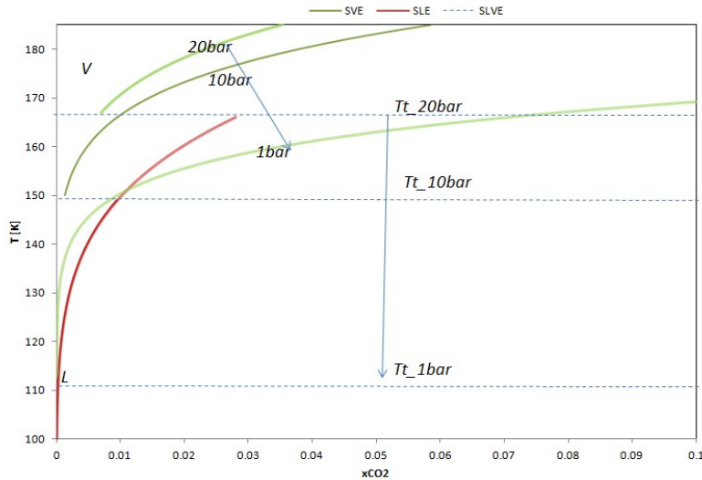
Figure 7.5: Variation of - SVE line, - SLE line and - - Triple Point temperature with pressure.
