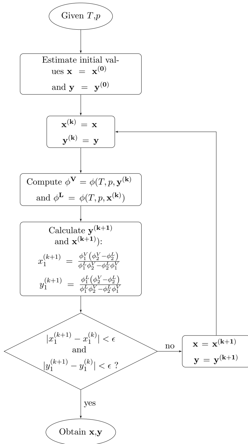
Figure 4.12: Flow diagram for petit flash algorithm
