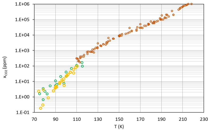
Figure 3.14: Comparison between the CO_2 solubility in liquid methane ( \circ ), nitrogen ( \circ ) and oxygen ( \circ ) according to SLE data available in literature (see tab. 3.2,3.4, 3.6 )
