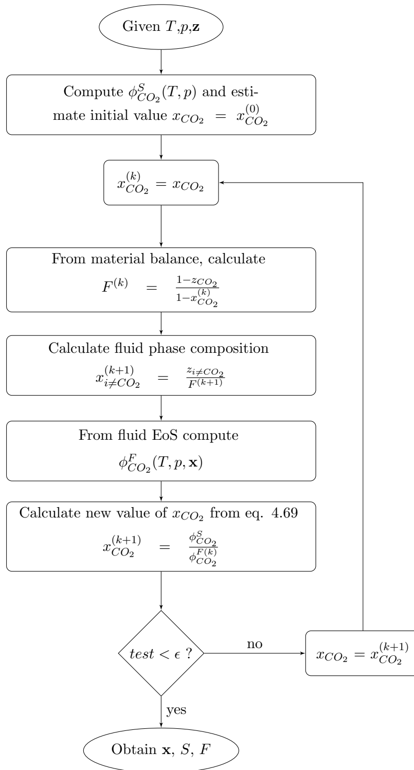
Figure 4.6: Flow diagram for SFE solving algorithm
