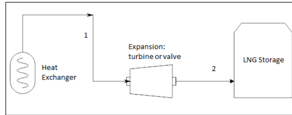
Figure 7.2: Scheme of a liquefaction process including the heat exchanger, the expansion valve or turbine and the storage tank.
