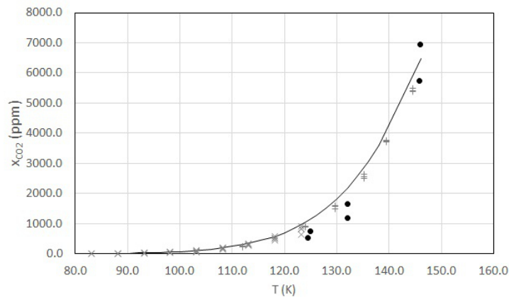
Figure 5.6: Comparison between CO_2 solubility in liquid phase for the ternary N_2-CH_4-CO_2 mixture obtained in this work ( \bullet ), data from Shen et al. (2012) (+) and Gao et al. (2012) ( \times ), and model results ( - ) obtained at constant pressure (10 bar) with the PR EoS+Zabaloy equation model
