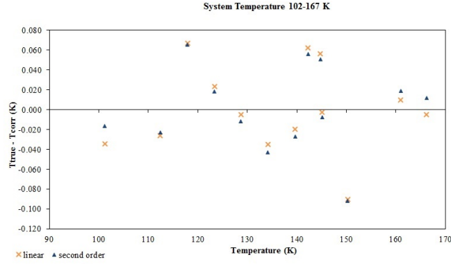
Figure B.2: Deviation between average temperature in the cell and temperature obtained by applying the calibration correlation in the range 102-167 K using a linear and a second order correlation for temperature calibration.
