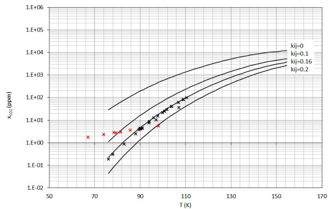
(b) SLE data used (×) and not used (×) for the regression; (—) results from model with different k_{ij} values;
