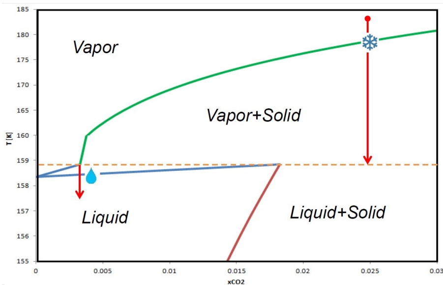
Figure 7.1: CO_2-CH_4 phase diagram at 15 bar. - SVE line, - VLE line, - SLE line, - - Triple Point temperature. Temperature scale on the y -axis is modified from 160 K for allowing the visualization of the freezing and the liquefaction points
