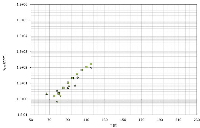
Figure 3.7: SLE data for the N_2 - CO_2 system in the xT diagram: (▲) data from Fedorova (1940), (◆) data from Rest et al. (1990), (■) data from Yakimenko et al. (1975)
