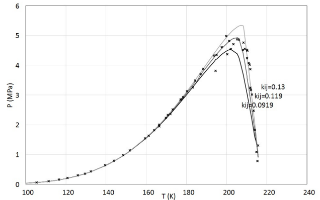
(b) Triple point locus obtained with different k_{ij} values (—) and experimental values (×)
