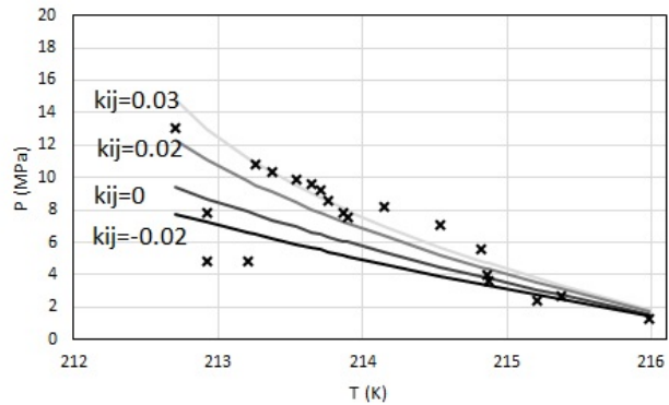
(b) Triple point locus obtained with different k_{ij} values — and experimental values ×
