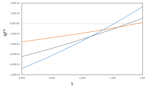
Figure 4.9: Difference between solid and liquid fugacity \Delta f^{SL} as function of solid molar fraction S for a mixture of 20% N_2 , 78% CH_4 , 2% CO_2 . T = 144.5 K , p = 1.4 MPa ; T = 135 K , p = 1 MPa ; T = 124 K , p = 0.6 MPa
