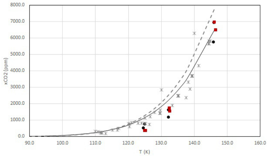
Figure 5.10: Comparison between CO_2 solubility in liquid phase for the ternary N_2-CH_4-CO_2 mixture obtained in this work ( \bullet ), model results ( - ), for the quaternary N_2-O_2-CH_4-CO_2 mixture obtained in this work ( \blacksquare ) and binary CH_4-CO_2 data from literature, see sec. 3.3 ( * ) and model results ( -- ). Results from model are obtained using the PR EoS+Zabaloy equation model.
