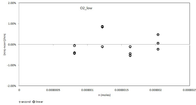
Figure B.6: Deviation between the number of moles injected in the GC and the number of moles obtained using a linear and a second order correlation for the Perichrom PR2100 GC TCD calibration for O_2 at lower injected volumes.
