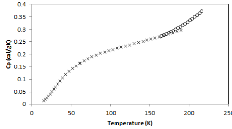
Figure A.2: Heat Capacity c_P versus temperature T for carbon dioxide: o Maass and Barnes (1926), x Giauque and Egan (1937)
