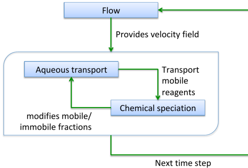
Figure 5: Reactive transport simulation software HYTEC functioning scheme [24]. This is the simplified diagram of actions within one time step
