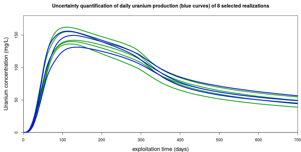
Figure 9: Approximated uranium uncertainty quantification using scenario reduction. The uranium recovery variability of the whole realization set is sampled by eight realizations. Using the computed weight of each selected realization, the P_{10} , P_{50} and P_{90} curves (blue) are selected to quantify the uncertainty
