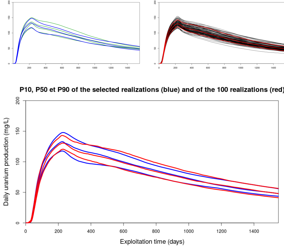
Figure 19: Uranium production UQ of selected realizations compared to uranium production UQ of the reference realization set. The top left graph shows the UQ of the sampled realizations and the top right graph the uranium production UQ of the whole realization set. The third graph compares the UQ of the whole set of realizations (red) and the sampled set of realizations (blue)
