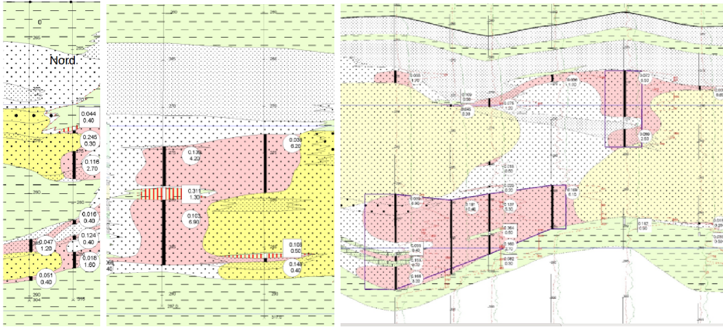
Figure 10: Three parallel vertical cross section of PB01 showing lithotype and mineralization distribution. Green corresponds to impermeable shale rocks. Yellow and white are barren sandrocks. Red is uranium ore sandrocks
