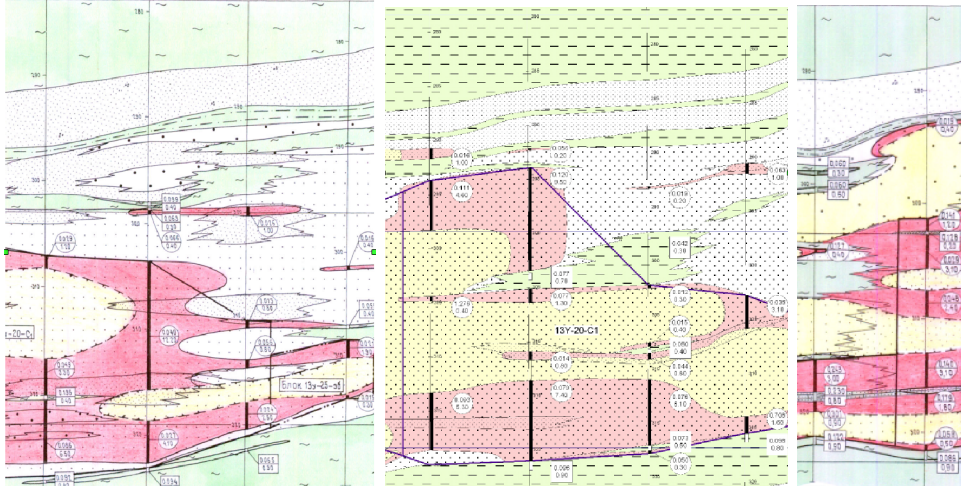
Figure 15: Three parallel vertical cross section of PB02 showing lithotype and mineralization distribution. Green are impermeable shale rocks. Yellow and white are barren sandrocks. Red is uranium ore sandrocks
