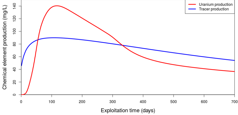
Figure 7: Comparison of daily uranium and tracer production. The blue curve is the tracer production in a realization during 700 days, and the red one is the ISR uranium production in the same realization
