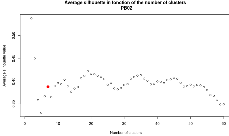
Figure 18: Value of the average silhouette in PB02 as a function of the number of cluster
