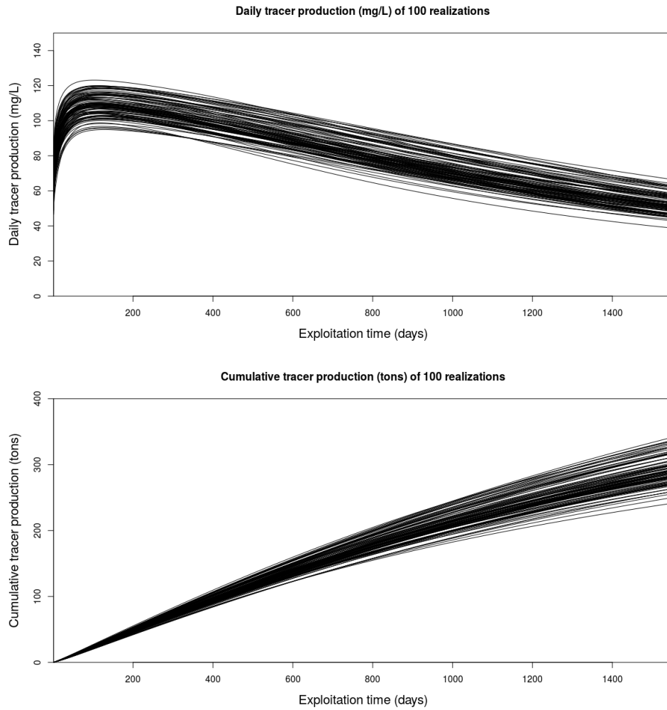
Figure 16: Daily and cumulative mineral tracer production for 100 realizations - validation block
