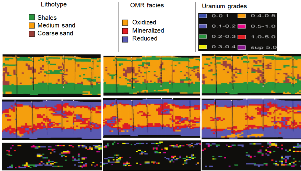
Figure 4: Same vertical cross section of three different realizations for the three properties: lithotype, OMR facies, and uranium grade distribution [17]. They are identical along drill holes. It is a transverse cross section of the deposit. Undefined uranium grades are black
