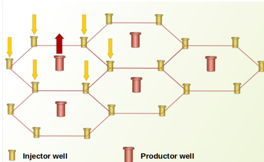
Figure 6: Well field mesh scheme with injectors and producers of a production block. A typical production cell is a hexagon of injector wells with a producer in the center of the cell. A production block is a group of a dozen production cells
