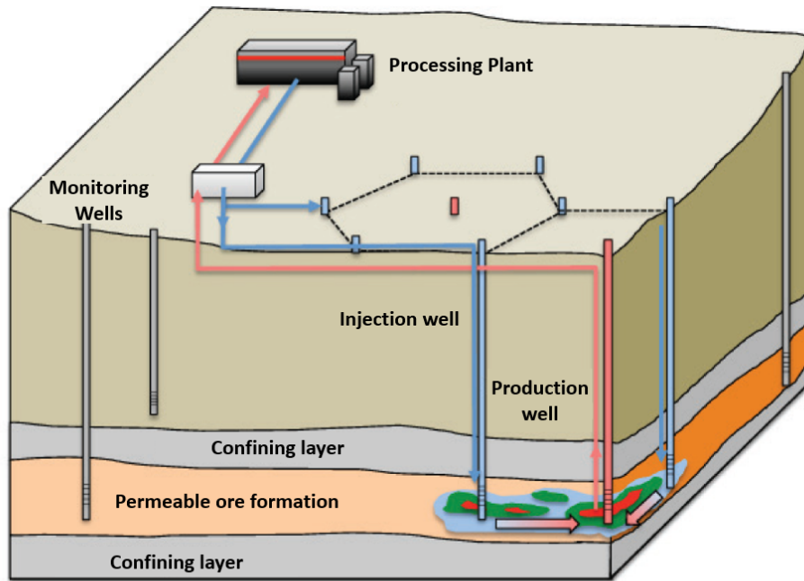
Figure 1. Schematic view of an ISR operation.
