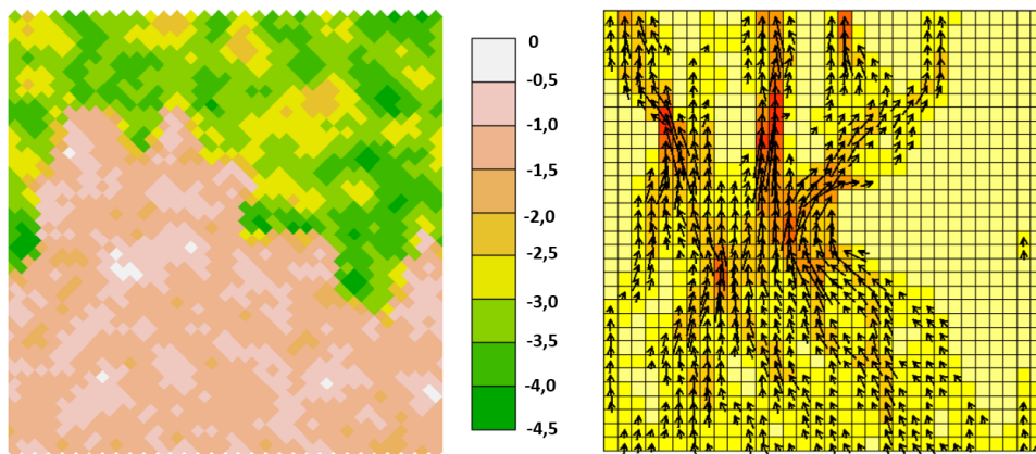
Figure 2: Example of the impact of the heterogeneous spatial distribution of permeability on fluid flow. The fluid flow controls the transport of chemical elements, and thus the transport of reactant. Chemical reactions in the systems are influenced by the heterogeneities [10]. Left: permeability field in decimal log scale, Right: resulting flow field
