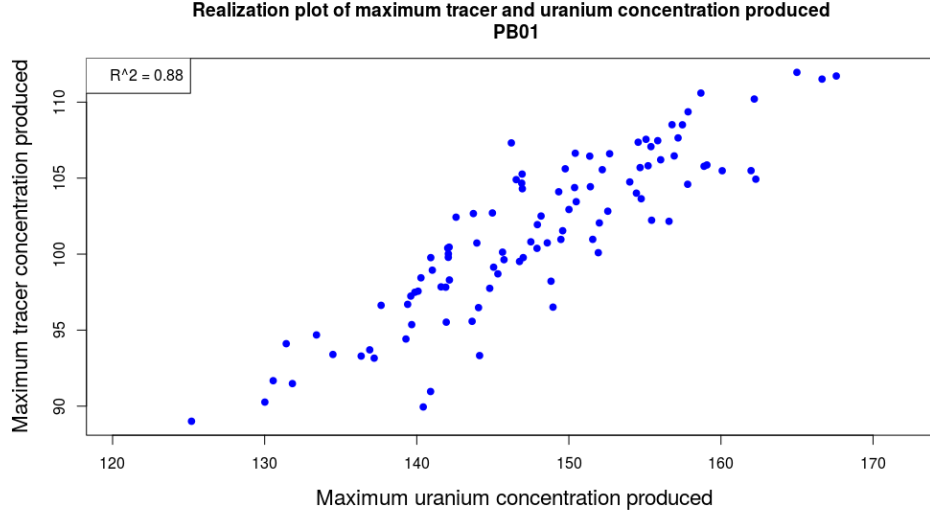
Figure 12: Comparison between maximum daily tracer production and maximum daily uranium production for the 100 realizations - PB01
