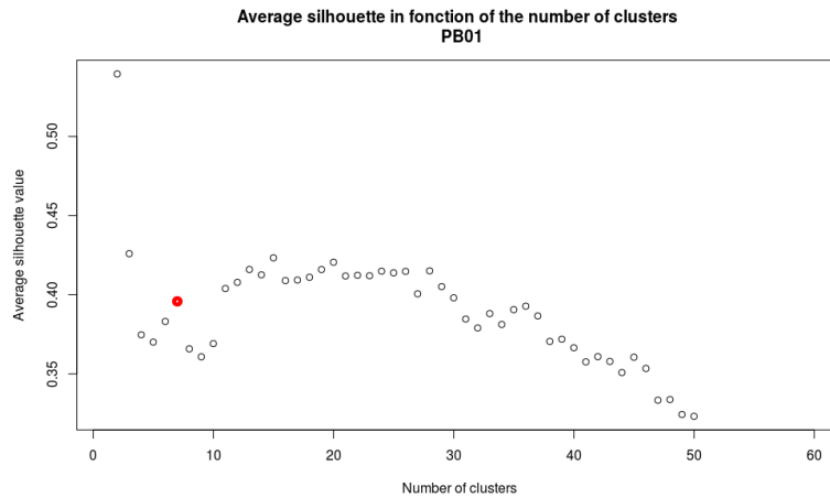
Figure 13: Value of computed the average silhouette in PB01 as a function of the number of cluster. The chosen number of cluster to perform the scenario reduction regarding these values and the allowed computational time is 7 clusters
