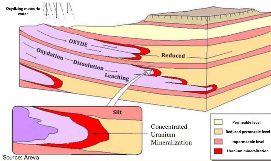
Figure 3: Roll-front uranium deposit scheme, from Fontaine et al [15]
