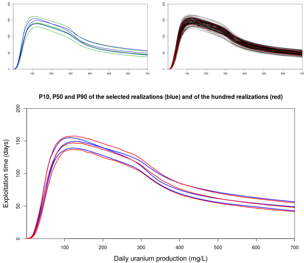
Figure 14: Uranium production UQ from the selected realizations compared to uranium production UQ of the reference realization set. The top left graph shows the UQ of the sampled realizations and the top right graph, the uranium production UQ of the whole realization set. The third graph shows the comparison between the UQ of the whole set of realization (red) and the sampled set of realizations (blue)
