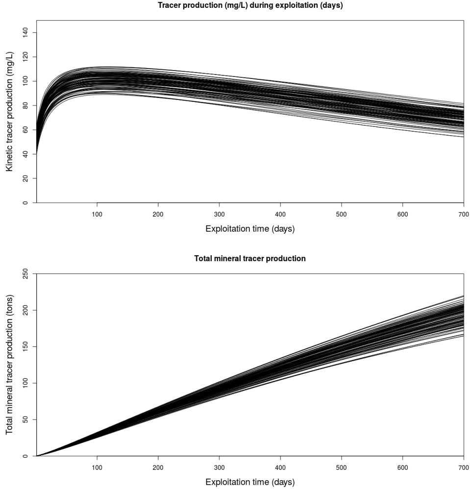
Figure 11: Daily and cumulative mineral tracer production for 100 realizations on PB01
