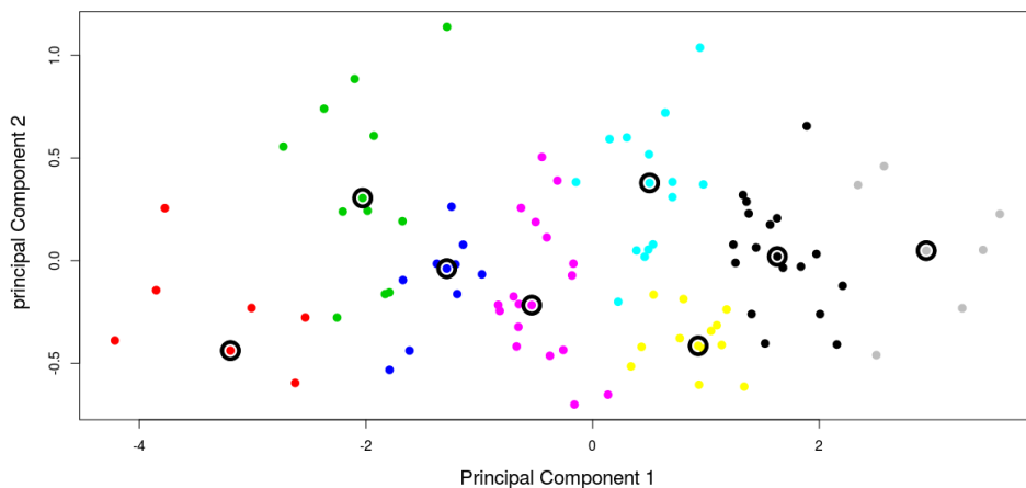
Figure 8: k -medoids algorithm result in a realization set. In this scatter plot, each point represents a realization, each color a cluster attribution, and each circled realization, the realization of the cluster that is nearest to its barycenter. The scatter plot is represented on the plan defined by the first two principal components obtained by MDS
