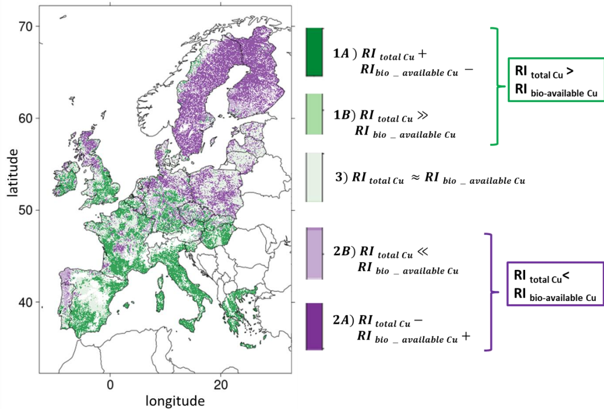
Fig. II.1.A.6: Map of risk assessment showing the comparison between the RI_{total\ Cu} and RI_{bio\text{-}available\ Cu} following the 5 cases defined in the material and method section 2.3, from purple meaning an underestimation of risk based on total rather than to bio-available Cu to green meaning an overestimation of risk based on total rather than to bio-available Cu
