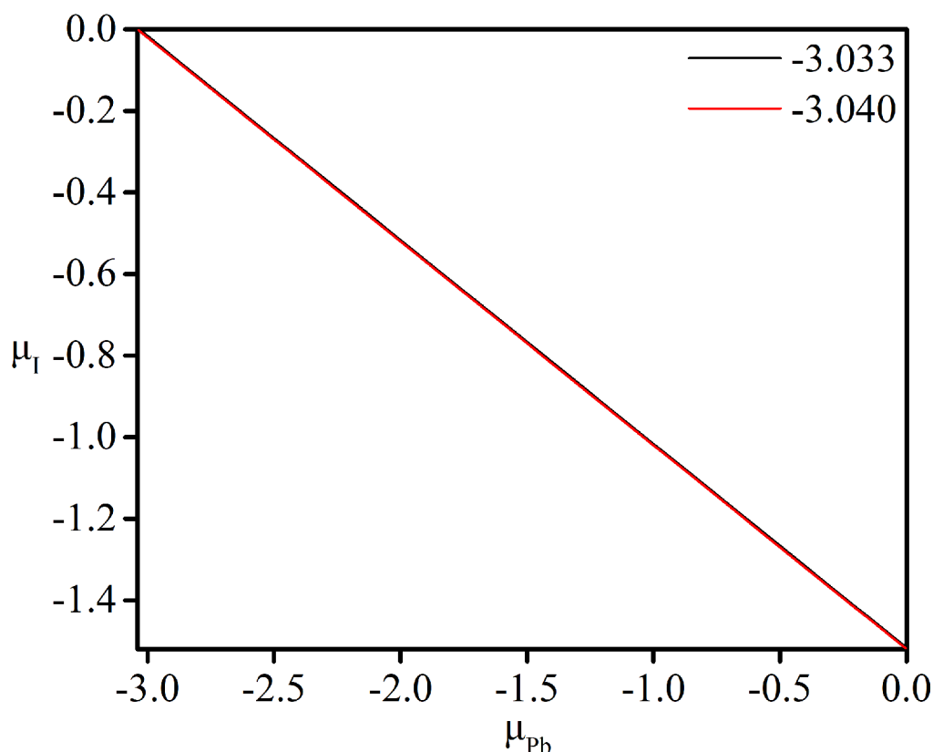
Figure 5.5.2: Stability diagram of \alpha -FAPI as a function of the range of variation of the Pb and I chemical potentials, with two values considered for \Delta H(PbI_2) . The -3.033 eV value corresponds to \Delta H(PbI_2) , while the -3.040 eV value corresponds to the value of [\Delta H(FAPI) - \Delta H(FAI)] . The red region is the thermodynamic stable range for equilibrium growth of \alpha -FAPI.
