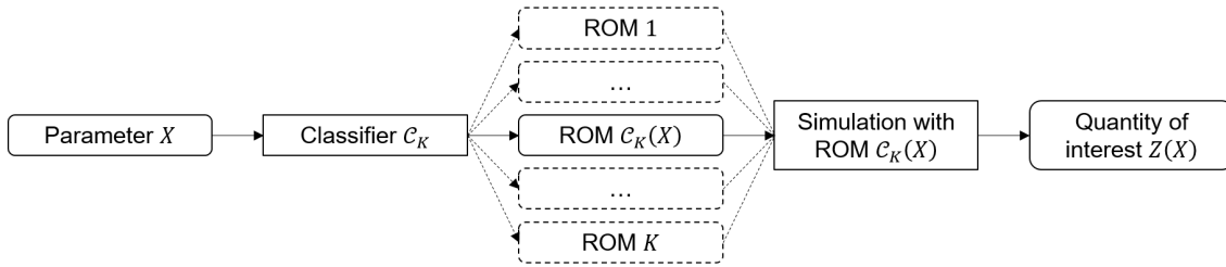
Figure 8.1: Exploitation phase of a dictionary-based ROM-net. K local ROMs are combined with a classifier \mathcal{C}_K for automatic model recommendation.
