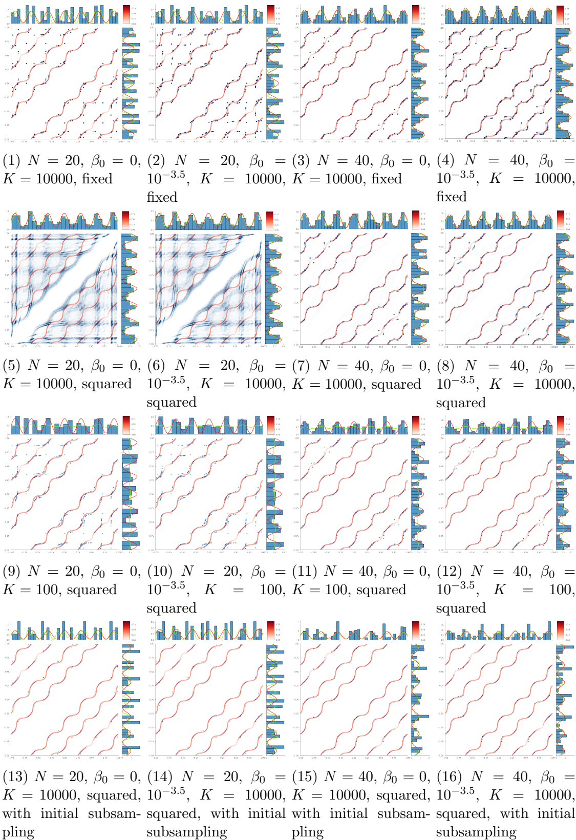
Figure 3.9: Optimal transport with \mu_3 and M = 5, \Delta t_0 = 10^{-3} . In each plot, on the main graph \frac{1}{M(M-1)} \sum_{k=1}^K \sum_{m \neq m'=1}^M w_k \delta_{x_m^k, x_{m'}^k} is represented by blue particles. The darker the heavier the particle. Particles have some transparency which allows to see more clearly areas of high concentration. Red curves represent the functions T^i for i \in \{1, \dots, M-1\} defined in Theorem 3.3. The higher the density the darker. On side graphs are represented in blue a weighted histogram of the particles, in red the marginal law and in green a normal kernel density estimate based on the weighted particles (with a bandwidth rule based on Scott's rule with d = 0 ).
