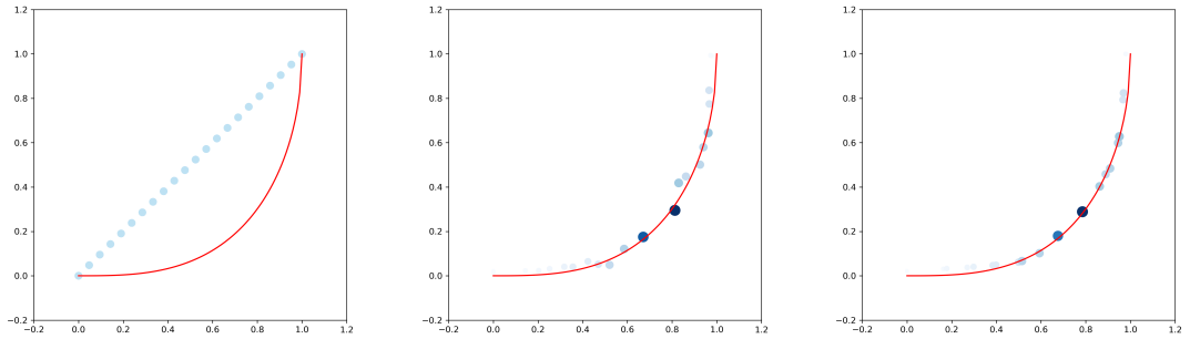
(7) Gauss, N = 10 , iter. 0. (8) Gauss, N = 10 , iter. 201. (9) Gauss, N = 10 , iter. 4201.
