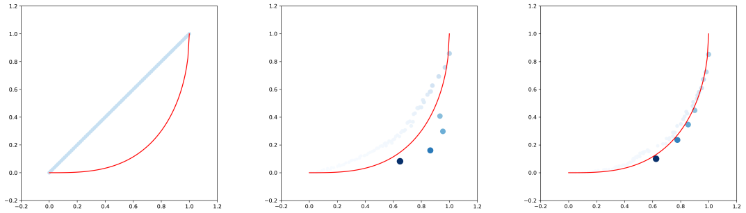
(4) RCPA, N = 40 , iter. 0. (5) RCPA, N = 40 , iter. 101. (6) RCPA, N = 40 , iter. 501.
