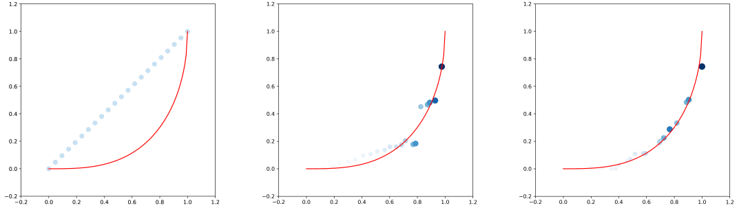
(1) RCPA, N = 10 , iter. 0. (2) RCPA, N = 10 , iter. 26. (3) RCPA, N = 10 , iter. 301.
