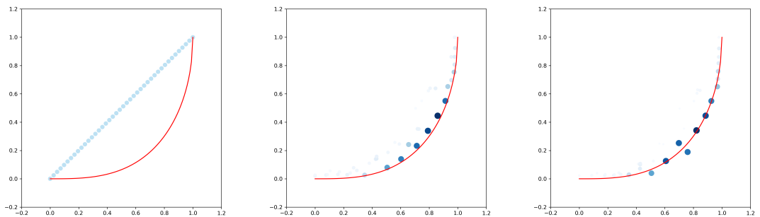
(10) Gauss, N = 20 , iter. 0. (11) Gauss, N = 20 , iter. 201. (12) Gauss, N = 20 , iter. 4201.
