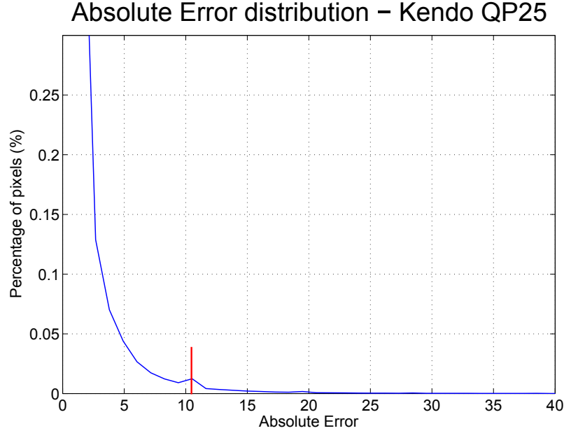
Figure 3.2 – Absolute error distribution for a synthesized frame in Kendo sequence, at QP=25.
