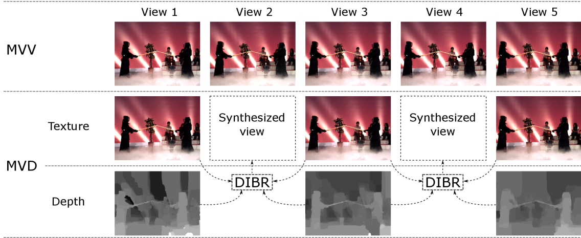
Figure 1.10 – MultiView and MultiView-plus-depth video.
