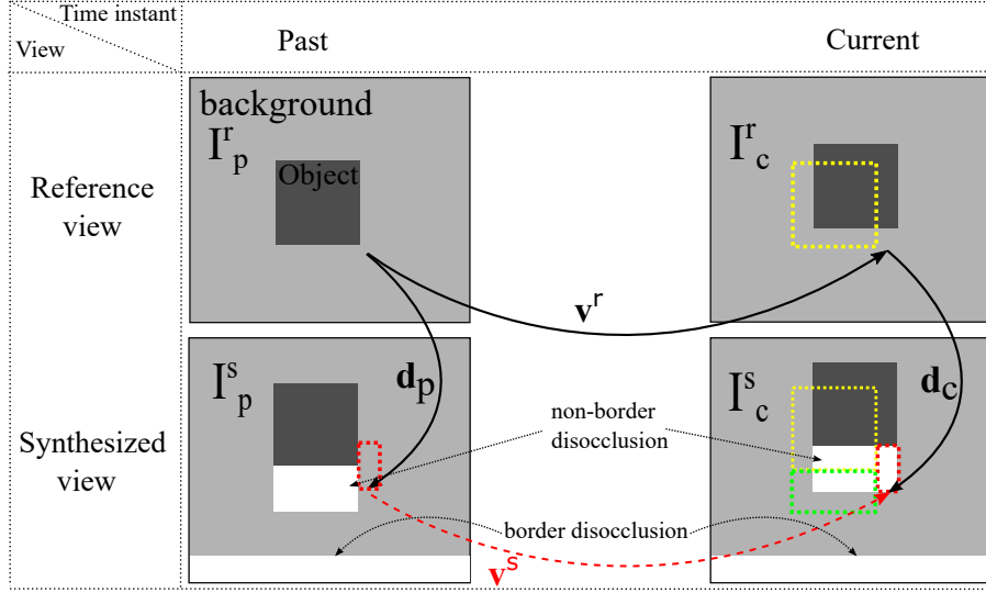
Figure 2.4 – Temporal retrieval of disoccluded area. Yellow dotted squares mark the position of the object in the previous frame, the green dotted square shows the disocclusions in the previous frame and red dotted squares mark the disoccluded area that was visible in a previous frame.
