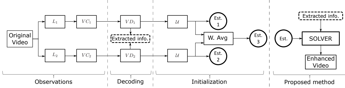
Figure 4.4 – A schematic view of the experimental setup. Two re-sampling operators are applied on an input sequence. Each observation is compressed and decompressed, and useful information is extracted. Decoded observations are up-sampled to their original resolution using either the reverse of the degradation operator or a SOA SR method. Then, the proposed framework is initialized with one high-resolution estimate and the information extracted during the decoding.
