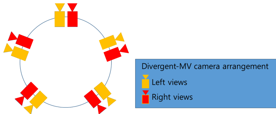
Figure 1.13 – Divergent-MV camera setup. [BLTW16].
