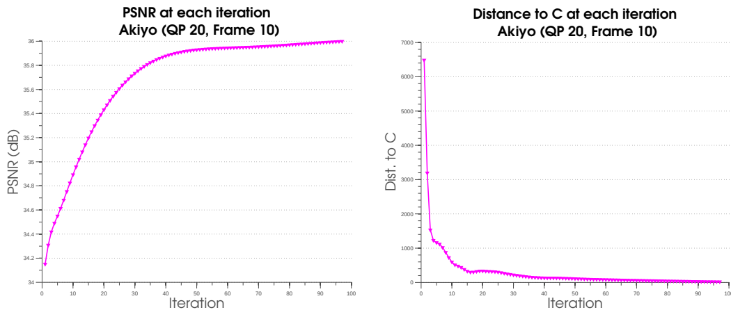
Figure 4.12 – PSNR and distance to the convex set C for each iteration. The distance represents the absolute error between the transformed, LR, estimated image and its projection onto C .
