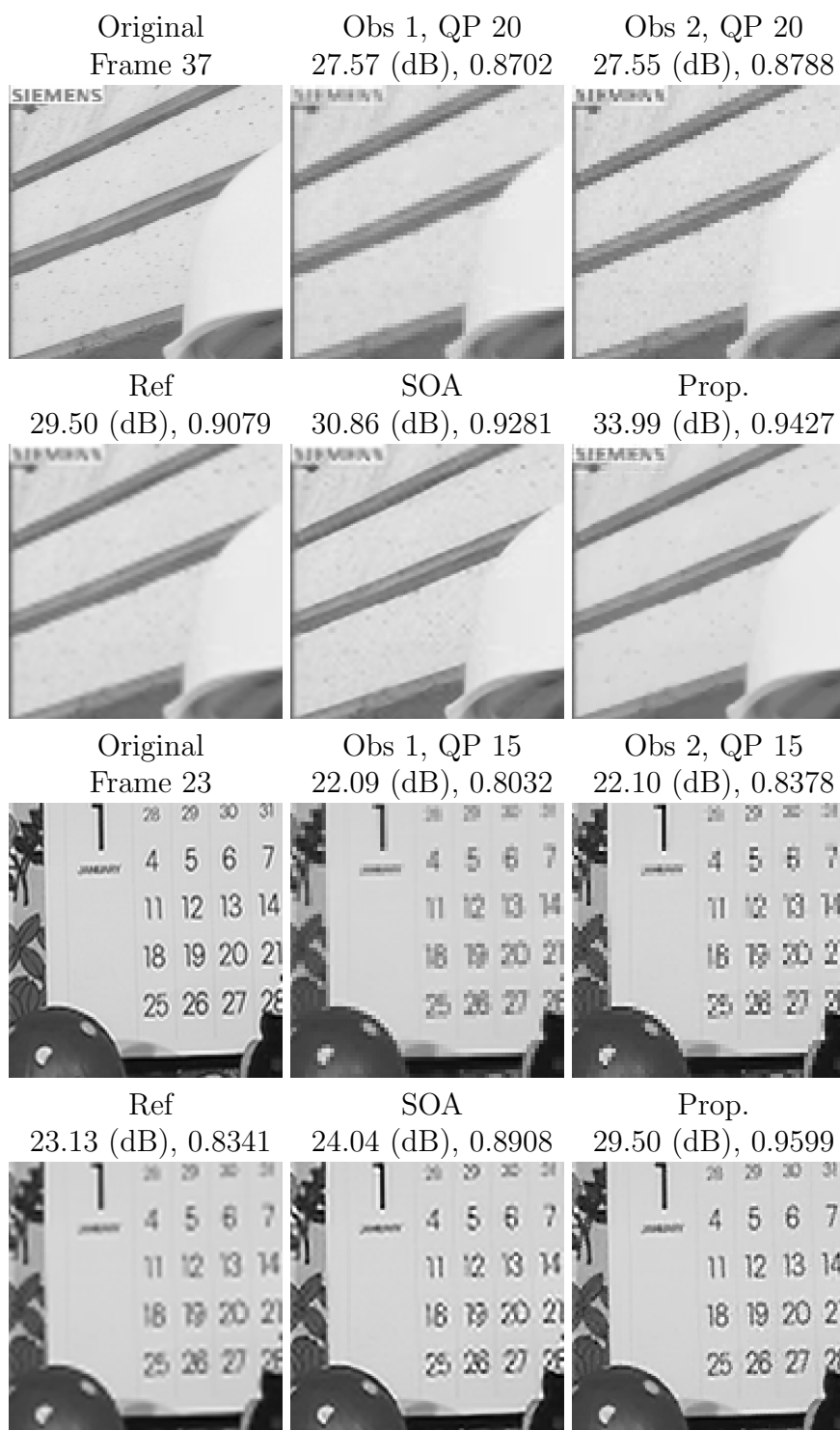
Figure 4.9 – Details of the up-sampled images and corresponding results of the super-resolution tested methods on Foreman and Mobile sequences. PSNR and SSIM values are computed on the compared image patch.
