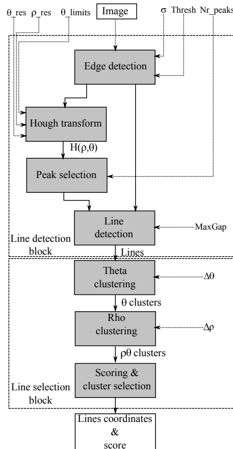
Figure 5.1 – Algorithm general scheme. Dotted lines indicate input data.
