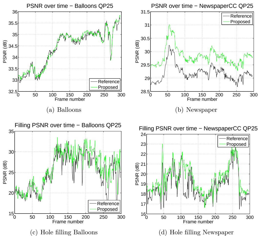
Figure 2.7 – PSNR variation of the middle synthesized view over time for the reference and proposed method at QP 25 in Balloons and Newspaper sequences. 2.7(a), 2.7(b):full frame; 2.7(c), 2.7(d):disoccluded areas.
