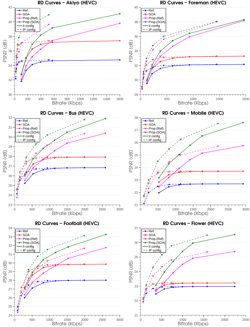
Figure 4.5 – Rate-distortion curves for the reference, SOA and proposed method initialized with the reference or SOA using HEVC encoding.
