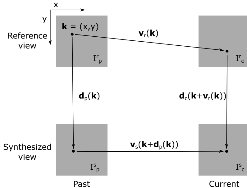
Figure 2.3 – Epipolar constraint, the relation between the disparity vector fields (DVs) \mathbf{d}_p and \mathbf{d}_c at two time instants c and p respectively, and the MVFs in the synthesized and reference view \mathbf{v}_s and \mathbf{v}_r respectively for a position \mathbf{k} in the reference frame I_p^r .
