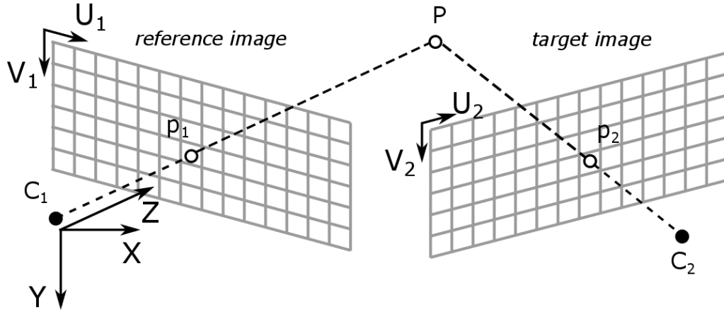
Figure 1.12 – Warping a pixel from a reference to a target image.
