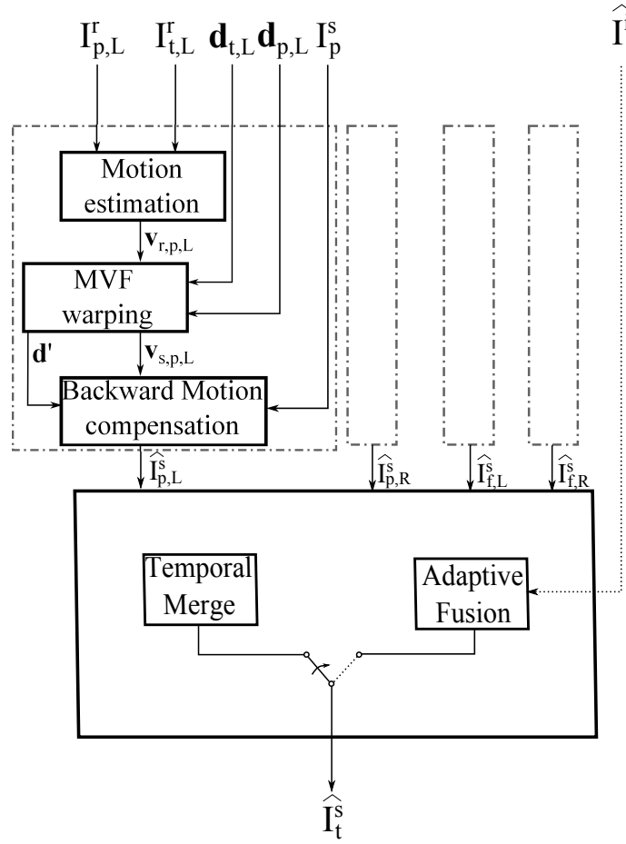
Figure 2.14 – Flow diagram for View Synthesis exploiting Temporal Prediction (VSTP). The dotted dash line is the temporal prediction block, which is applied four times, i.e. past and future time instants ( p and f ) in the left and right ( L and R ) reference ( r ) views.
