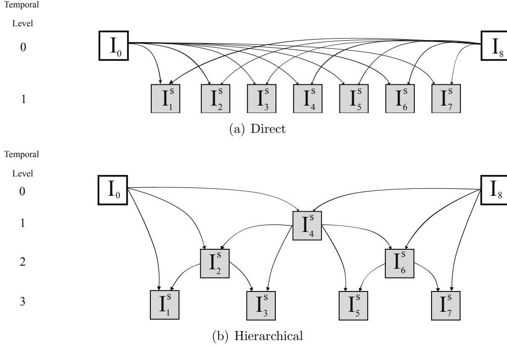
Figure 2.15 – Temporal prediction schemes inside a GOP of the synthesized view.
