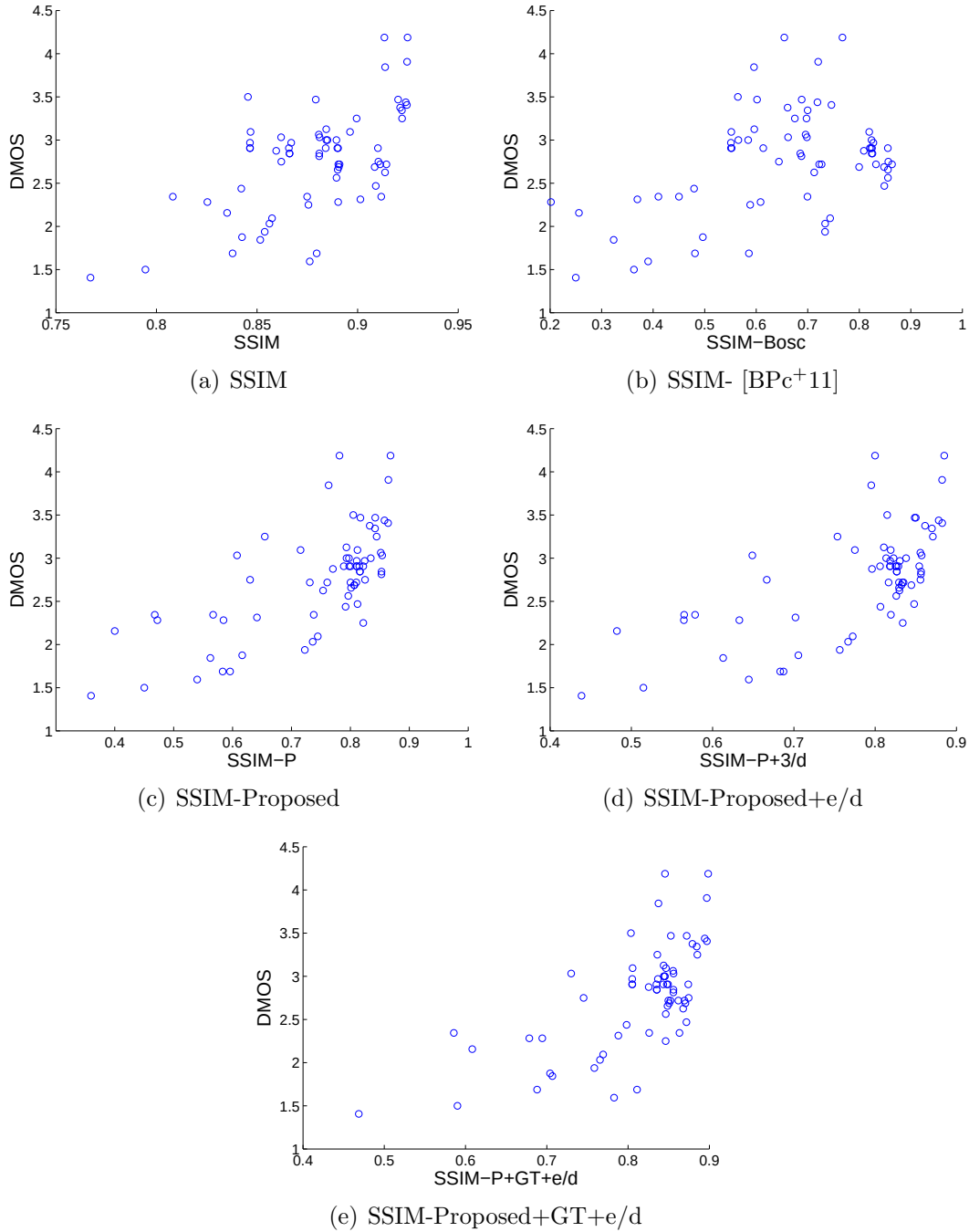
Figure 3.7 – Scatter plots of objective results for SSIM with tested ROIs. Each point is the DMOS against the average objective score over all frames for a sequence, synthesis and method.
