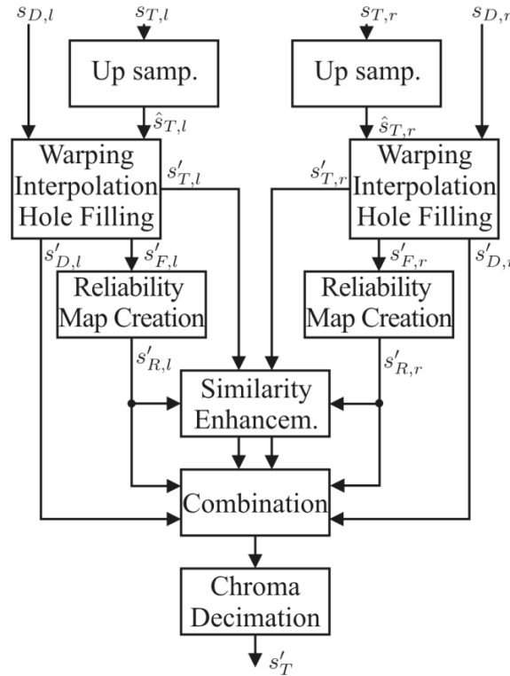
Figure 2.2 – Flow diagram for View Synthesis Reference Software 1D Fast (VSRS-1DFast) [ZTWY13].
