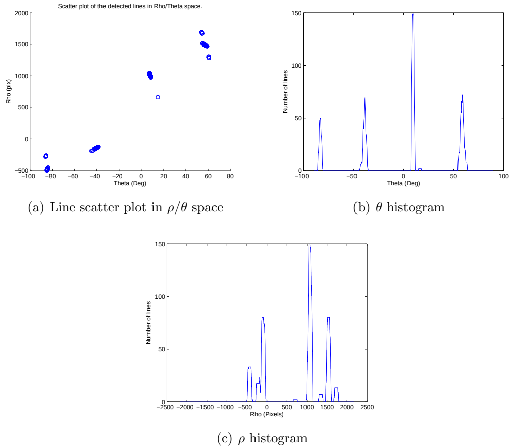
Figure 5.3 – The line scatter plot in \rho/\theta space 5.3(a) and the lines histograms with respect to Theta 5.3(b) and \rho 5.3(c).
