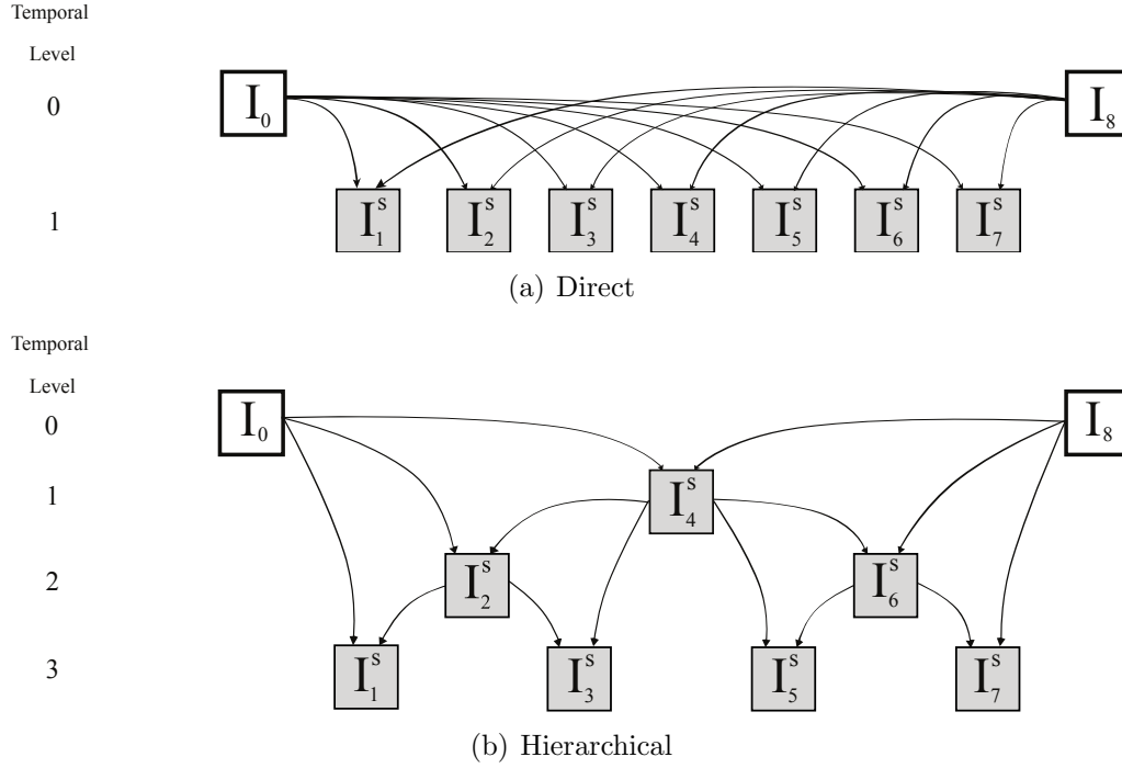
Figure 11 – Temporal prediction schemes inside a GOP of the synthesized view.
