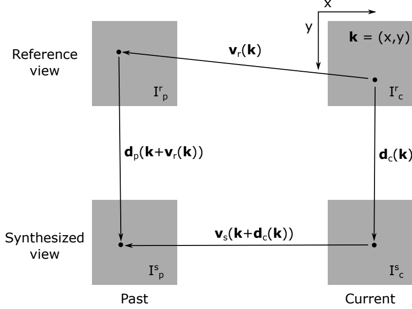
Figure 2.9 – Epipolar constraint when using forward prediction.
