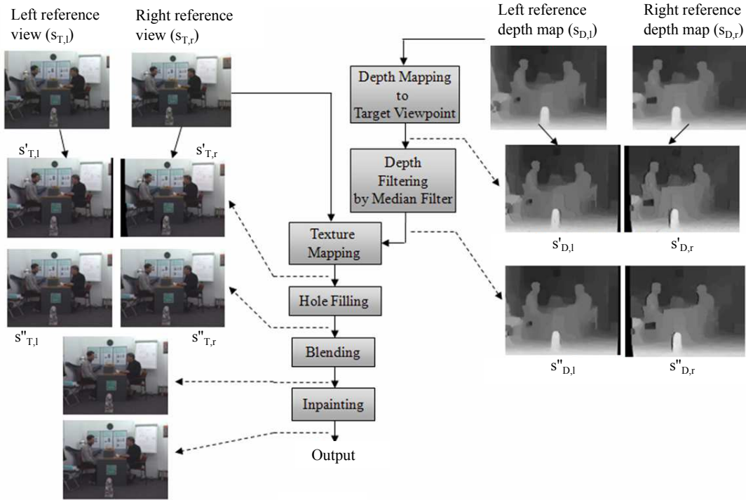
Figure 2.1 – Flow diagram for View Synthesis Reference Software (VRSR) general mode [EXP10].
