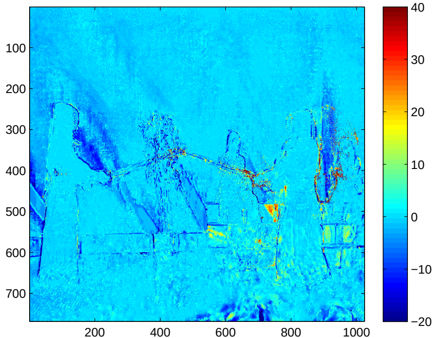
Figure 2.21 – Difference between inter-view and temporal prediction error ( \Delta\text{MAE} ) on frame 4 in Kendo sequence, QP 30.
