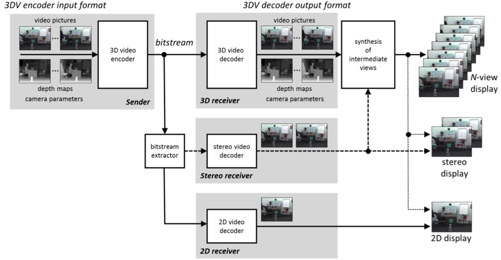
Figure 1.11 – MPEG's overview of an MVD transmission system [CTWY14].
