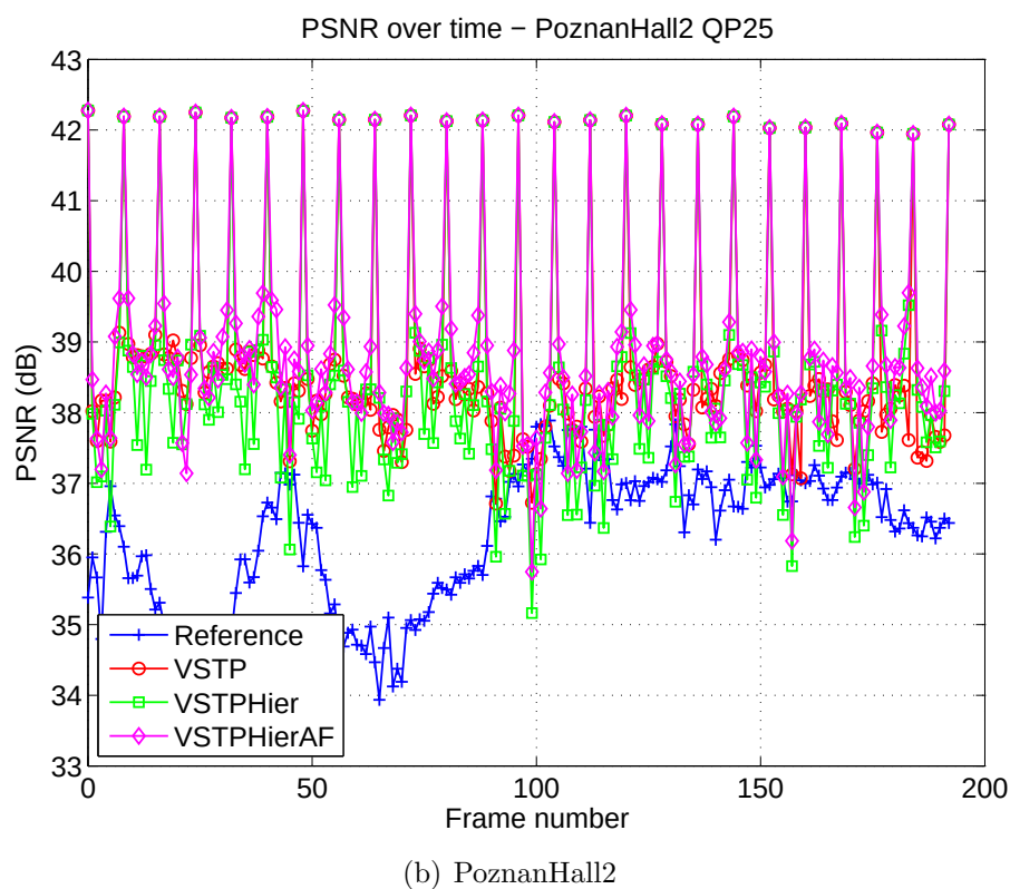
Figure 2.19 – PSNR variation over time of the middle synthesized view for the reference and proposed methods at QP 25 on NewspaperCC and PoznanHall2 sequences.
