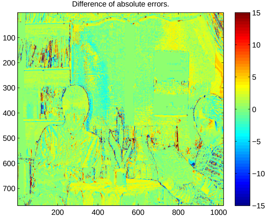
Figure 2.8 – Difference between absolute errors for frame 15 from Newspaper sequence.
