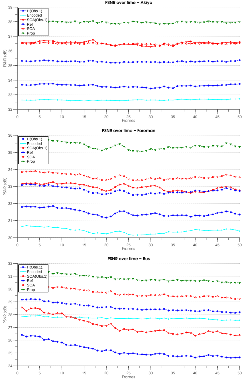
Figure 4.7 – PSNR over time on Akiyo, Foreman and Bus sequences. One down-sampled observation encoded at QP15 (Obs 1) and one observation at full resolution encoded at QP40 (Encoded). H(Obs 1) and SOA(Obs 1) denote the two up-sampling methods applied on Obs 1; Ref and SOA denote the weighted average of the encoded observation and the up-sampled Obs 1 and Prop is the proposed method.
