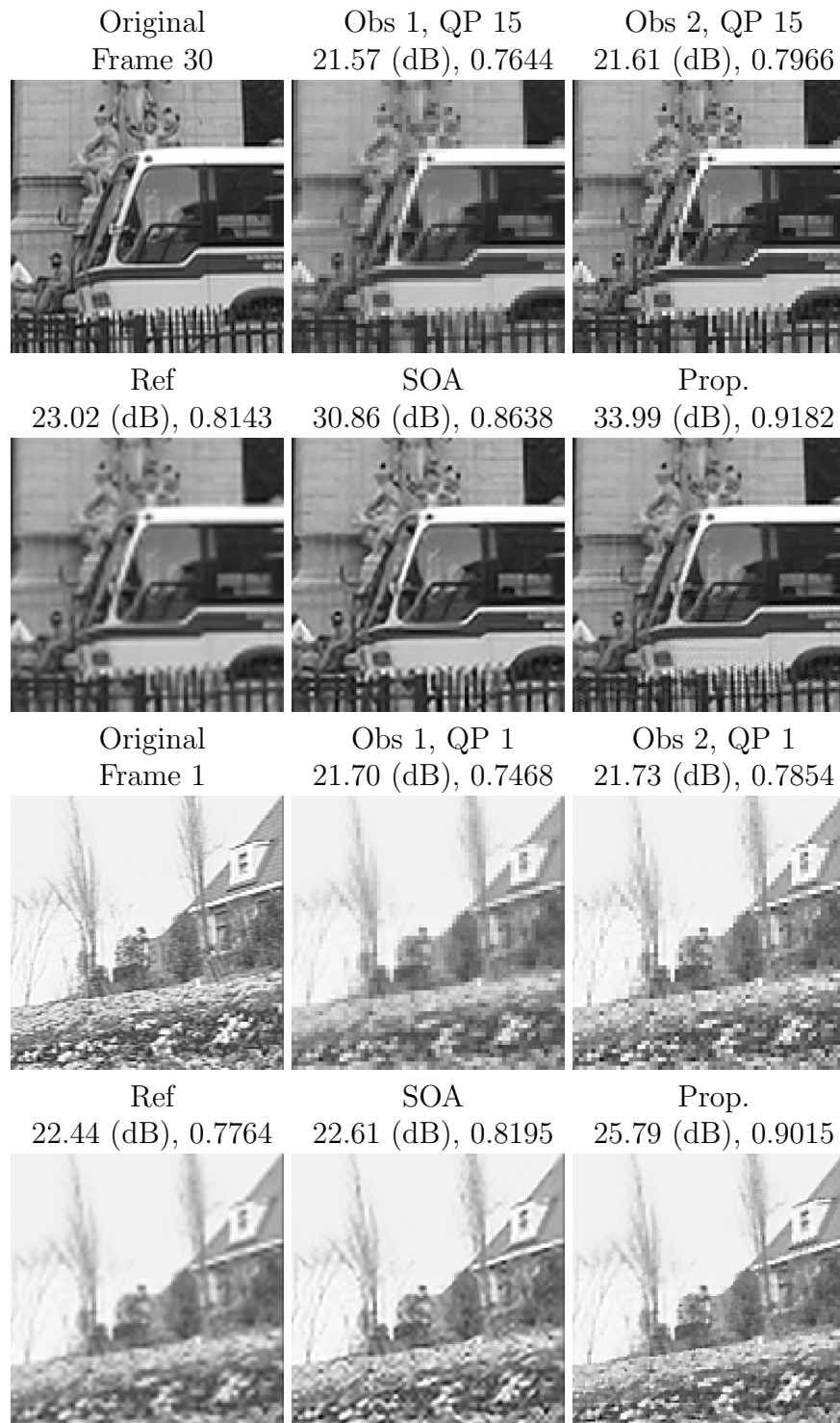
Figure 4.10 – Details of the up-sampled images and corresponding results of the super-resolution tested methods on Bus and Flower sequences. PSNR and SSIM values are computed on the compared image patch.
