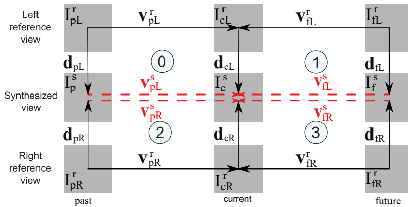
Figure 2.5 – Temporal hole filling scheme, for two base views and an intermediary synthesis, using past and future synthesized frames to retrieve information.
