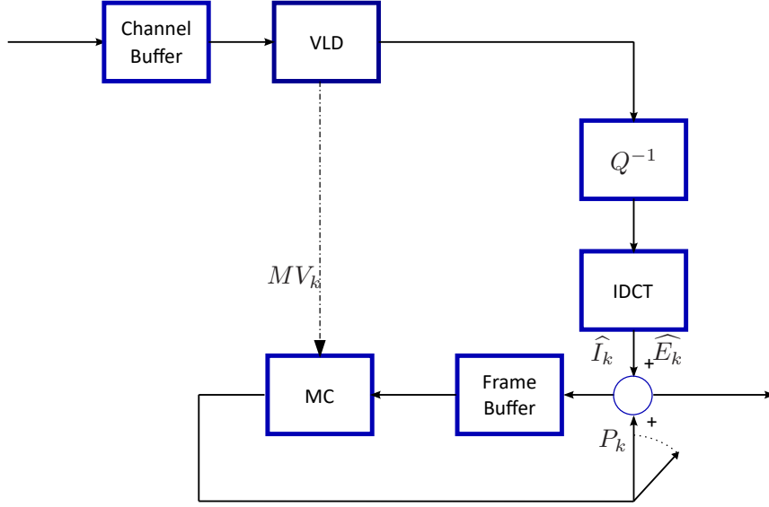
Figure 1.6 – Generic hybrid decoder scheme.
