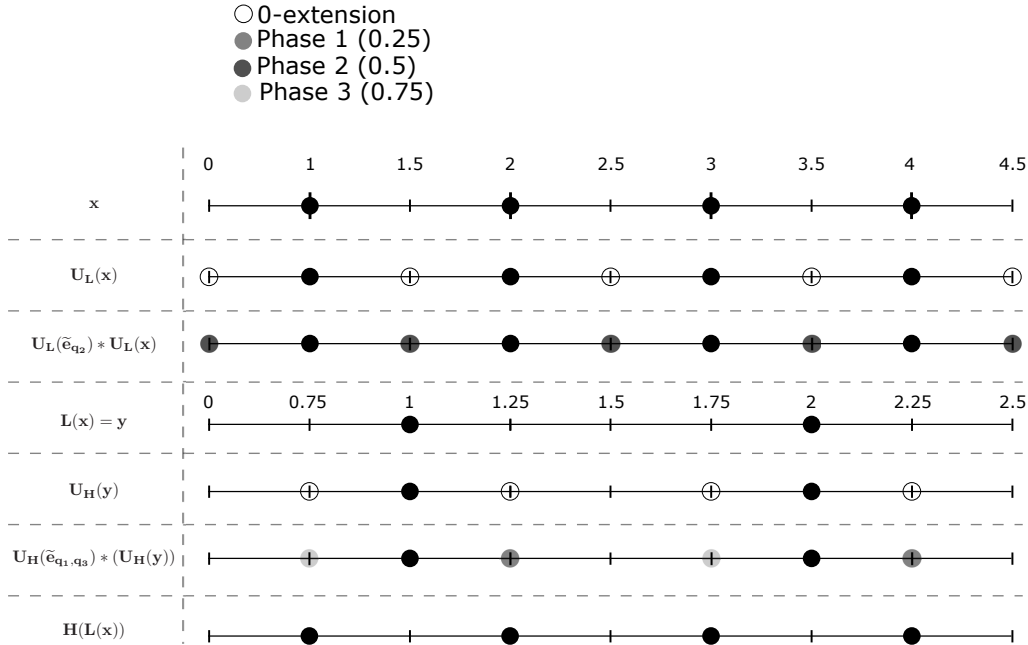
Figure 4.3 – Down-sampling and up-sampling operators.
