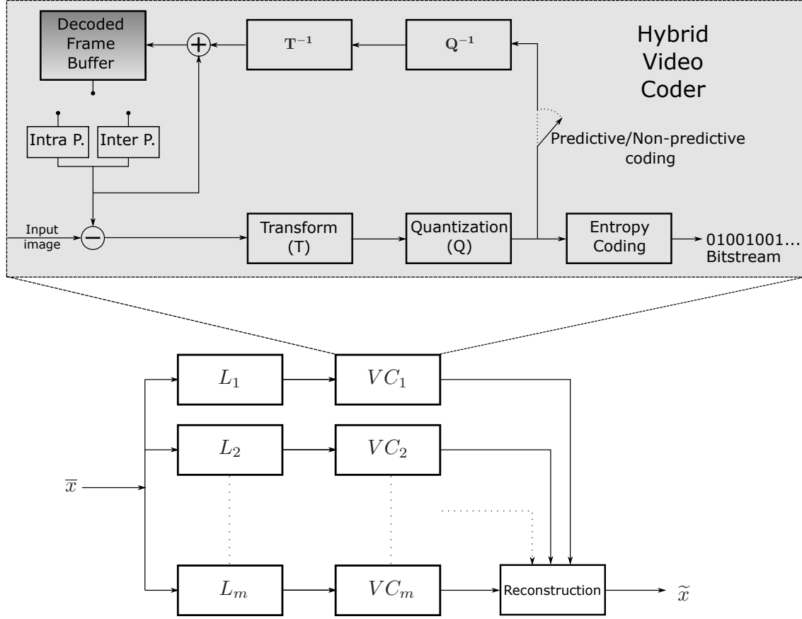
Figure 4.1 – A generic model for multiple video sources sub-sampling, compression and reconstruction.
