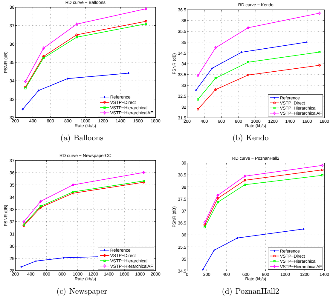
Figure 2.16 – RD curves of the reference and proposed method on 3 view test scenario for the Balloons, Kendo, NewspaperCC and PoznanHall2 sequences.
