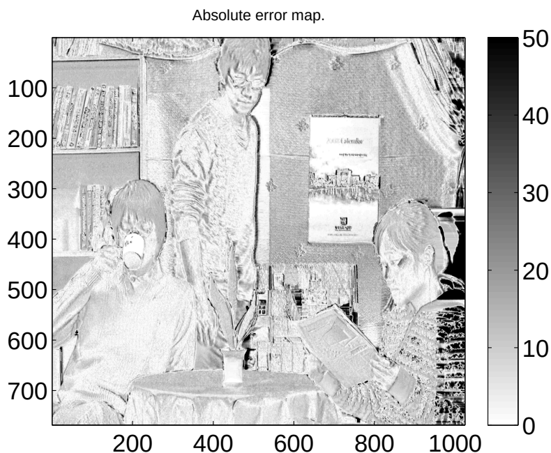
Figure 3.5 – Absolute error gray scale map for frame 93 of Newspaper sequence. View 6 synthesized from view 4 using [Feh03].
