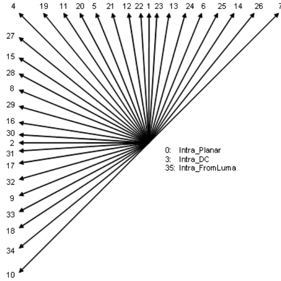
Figure 1.8 – HEVC intra modes.
