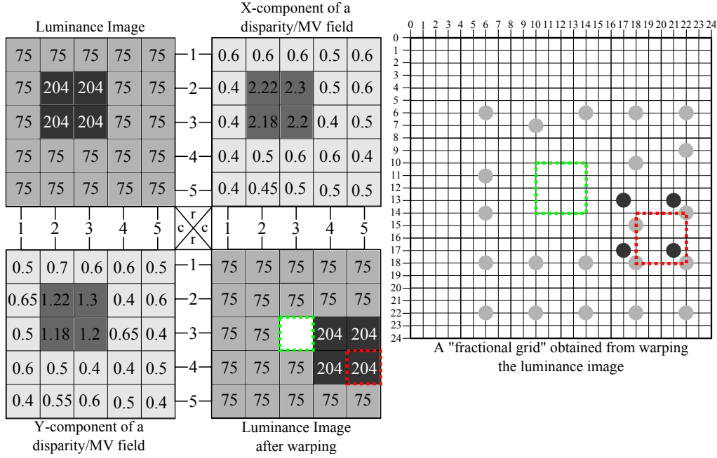
Figure 2.6 – A simple sub-pixel precision warping example with our proposed technique. Dotted lines represent filtering windows and the corresponding result in the warped image; green indicates a hole and red a case of foreground and background overlapping.
