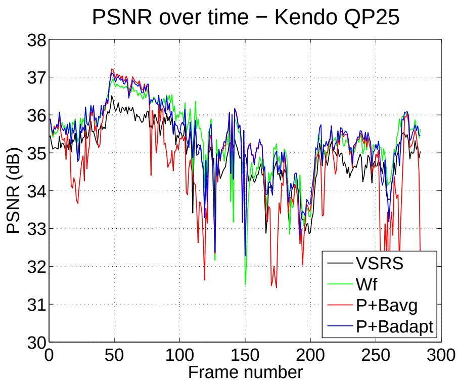
Figure 2.11 – PSNR variation of the synthesized view over time for the reference and proposed methods at QP 25 in Balloons 2.11(a), Kendo 2.11(b), NewspaperCC 2.12(a) and Poznan Hall2 2.12(b) sequences.
