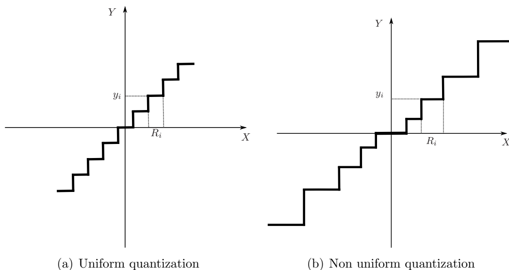
Figure 1.2 – Uniform and non uniform quantization.
