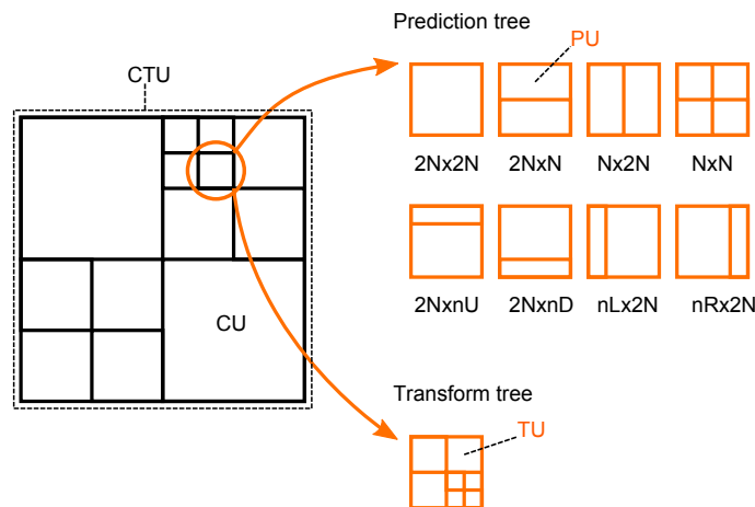
Figure 1.7 – Frame partitioning structure in HEVC.
