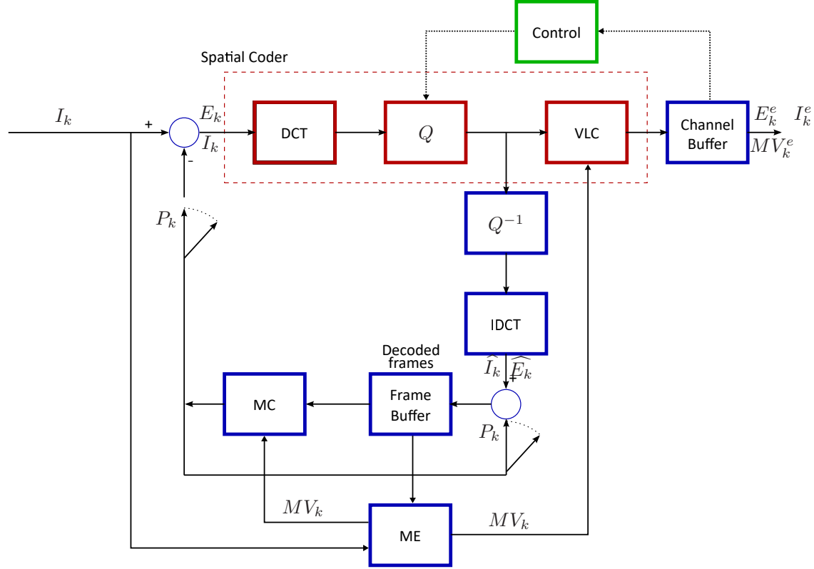
Figure 1.5 – Generic hybrid coder scheme.
