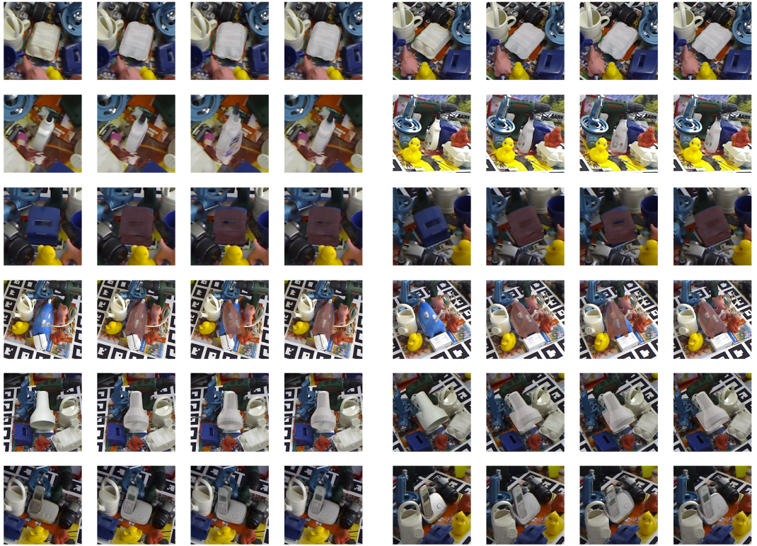
Figure 3.5: (cont.) Visual results of object pose estimation on LINEMOD ( Hinterstößer et al., 2012b ). For each sample, the four columns from left to right represent: the input image, the correct shape and orientation, our initial estimate and the final estimate after refining our initialization with DeepIM ( Li et al., 2018b ).
