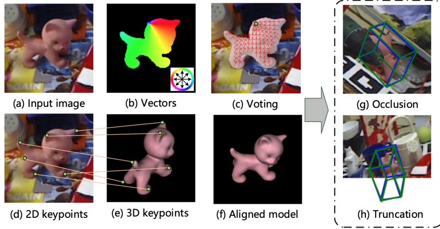
Figure 2.8: Figure from (Peng et al., 2019). Network is trained to predict an unit vector pointing to keypoints for each pixel, and the localization is done in a RANSAC based voting scheme.
