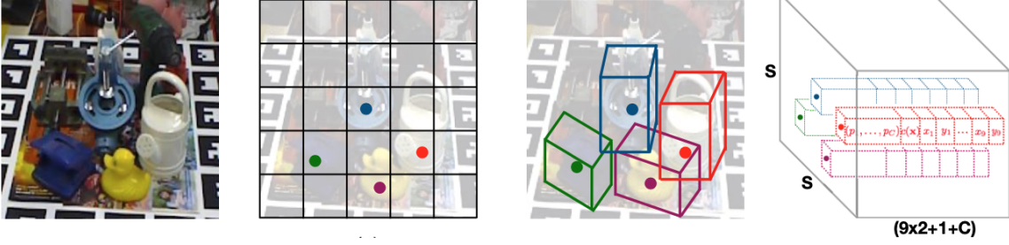
Figure 2.7: Figure from (Tekin et al., 2018). Given an input image, a grid of regular cells are generated. Each cell is responsible for predicting the 2D locations of the eight 3D bounding box corners and the object centroid in the image, together with a confidence score and the class probabilities.
