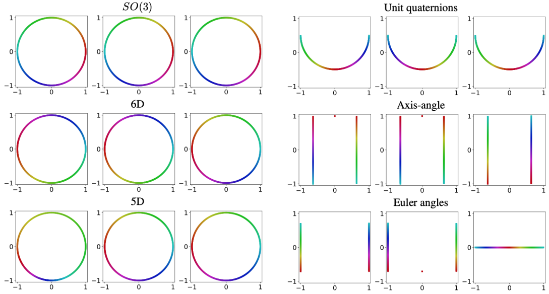
Figure 2.16: Figure from (Zhou et al., 2019). Visualization of discontinuities in 3D rotation representations. Each column represent the rotation about the corresponding axis for "X", "Y" and "Z". The curve in 2D should be homeomorphic to a circle with similar colors in nearby spatial locations if the representation is continuous.
