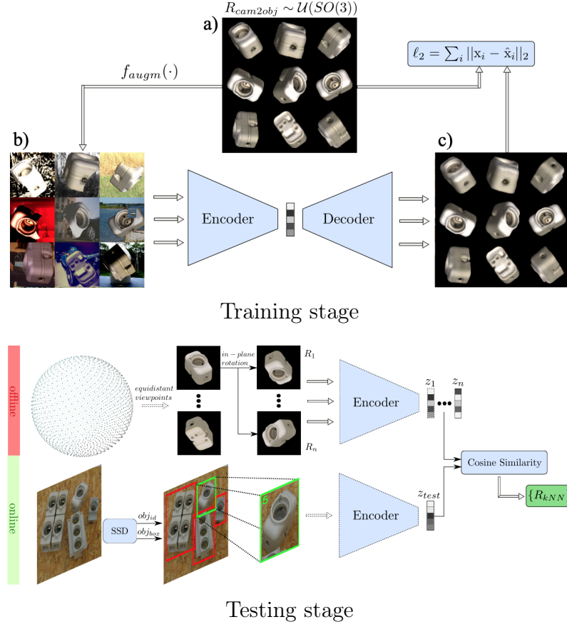
Figure 2.6: Figure from (Sundermeyer et al., 2018). By training the Autoencoder with a reconstruction loss, image encodings of clean rendered views are mapped closer with image encodings of randomly augmented images in the same pose. The learned encoder is then used to create a codebook from the encodings of discrete synthetic object views, and pose estimation is done by matching the input image encoding against the codebook.
