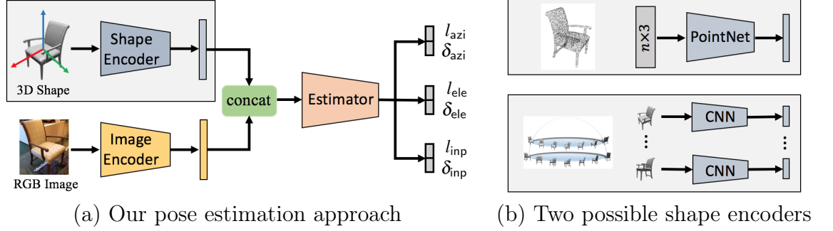
Figure 3.2: Overview of our method. (a) Given an RGB image of an object and its 3D shape, we use two encoders to extract features from each input, then estimate the orientation of the pictured object w.r.t. the shape using a classification-and-regression approach, predicting probabilities of angle bins l and bin offsets \delta . (b) For shape encoding, we encode a point cloud sampled on the object with PointNet (top), or we rendered images around the object and use a CNN to extract the features (bottom).
