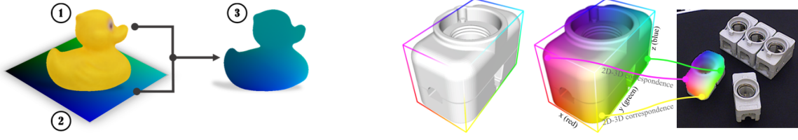
Figure 2.9: (Left) Figure from (Zakharov et al., 2019), a UV-mapping is used to get the 2-channel correspondence map with values in 0 to 255. (Right) Figure from (Park et al., 2019), normalized coordinates of each 3D vertex are directly mapped to RGB values in the color space.
