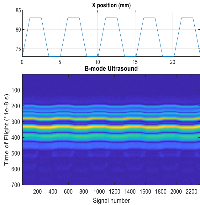
Figure 5a.12: Variation of ultrasound ToF with respect to the displacement of the horizontal stage.
