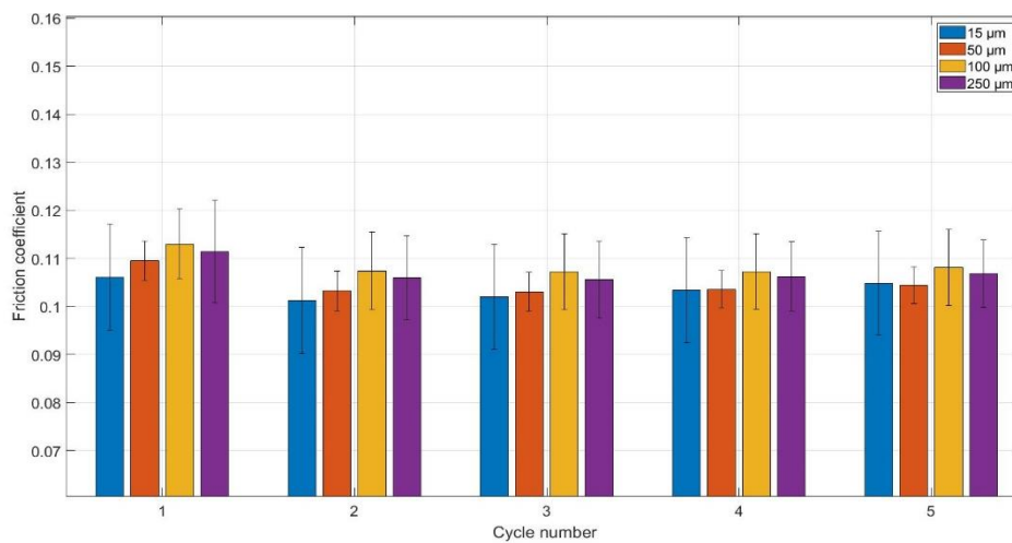
Figure 6.4: Friction coefficient values for the diluted cottage cheese with vivapur particles on soft model tongue ( 50.17 \pm 1.46 kPa) with rough surface profile. Normal stress and shearing velocity were 9 kPa and 10 mm/s, respectively. The error bars represent the standard deviations across six replicates.
