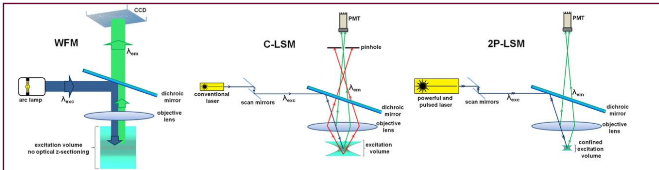
Figure 7: The direction of the optical paths in the different microscopy modes. Wide field microscopy (WFM), confocal laser scanning microscopy (C-LSM), two photons laser scanning microscopy (2P-LSM). Illumination light is blue (excitation wavelength: \lambda_{exc} ), in focus fluorescence emission is green (emission wavelength: \lambda_{em} ), out of focus emission fluorescence is red. Detector: Charge Coupled Device camera (array) or PhotoMultiplifier tube (point source). (From: [107]).
